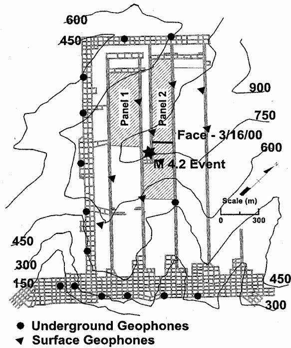
Figure 1. Plan view showing mine layout, overburden, geophone arrays, and the location of the M 4.2 event
