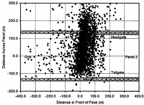
Figure 4. Plan view of the normalized event locations for the last part of panel 2
