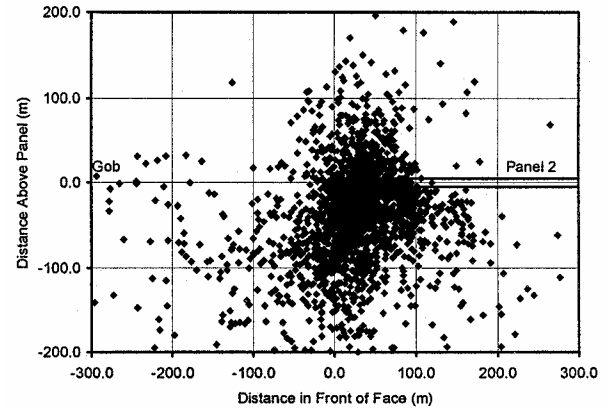
Figure 5. Vertical view parallel to face advance showing the normalized event locations for the last part of panel 2
