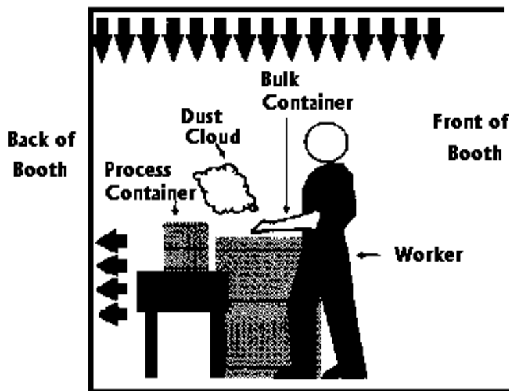
Illustration: A Semidowndraft Ventillated Booth
