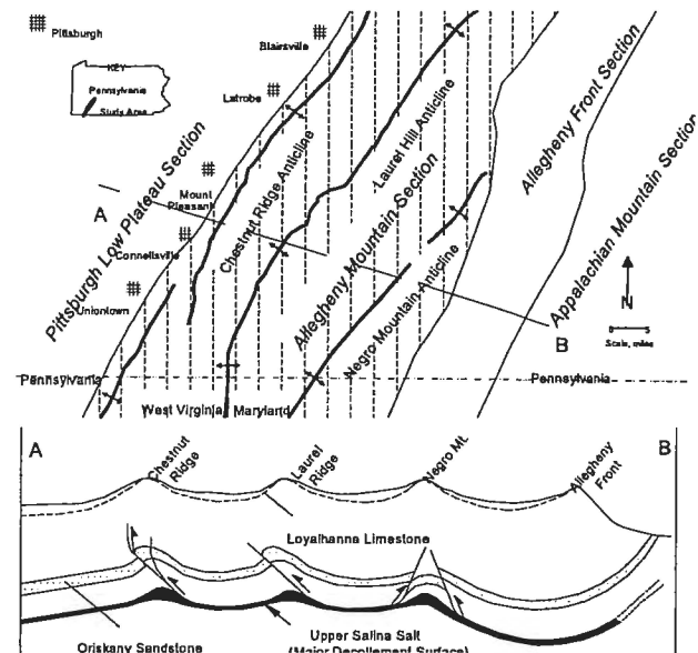
Figure 1. Location of major anticlinal structures and a generalized cross-section through the Allegheny Mountain Section of the Appalachian Plateaus Province.
