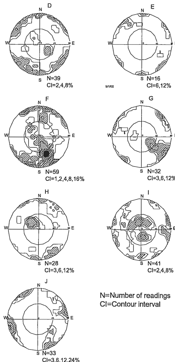
Figure 9. Stereonet projections for seven of the sites visited during this study.
