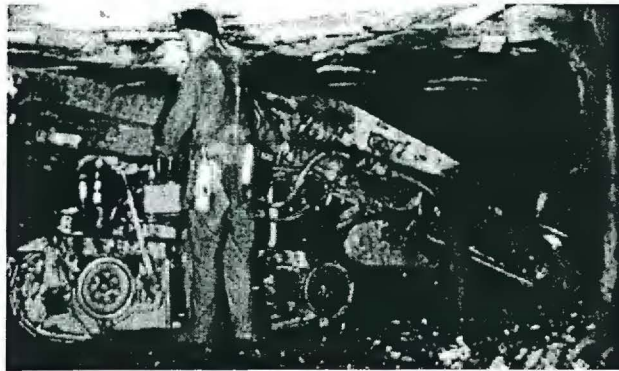
Figure 14. Machine loading with roof bolts.
