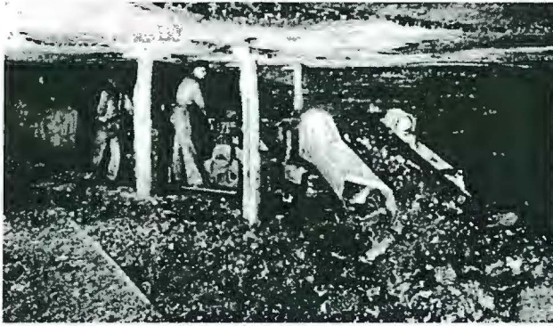
Figure 5. Machine loading with timber support.
