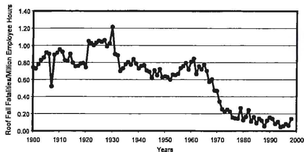
Figure 2. Roof fall fatalities in underground coal mines.
