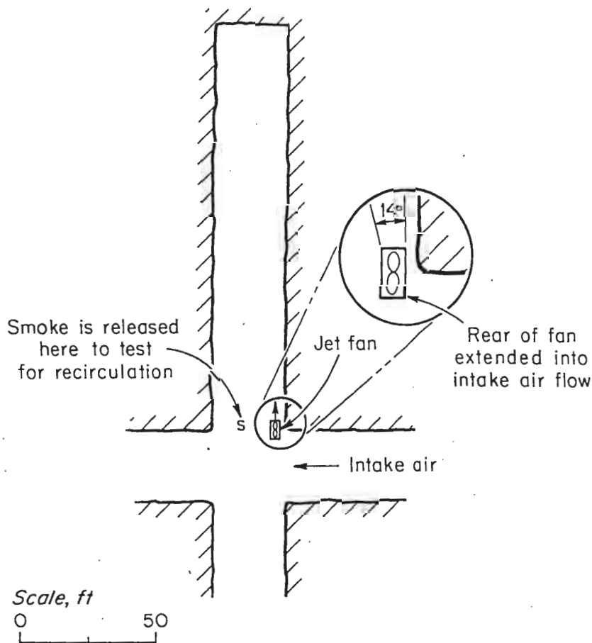
Figure 1. Jet fan ventilating a straight single heading.
