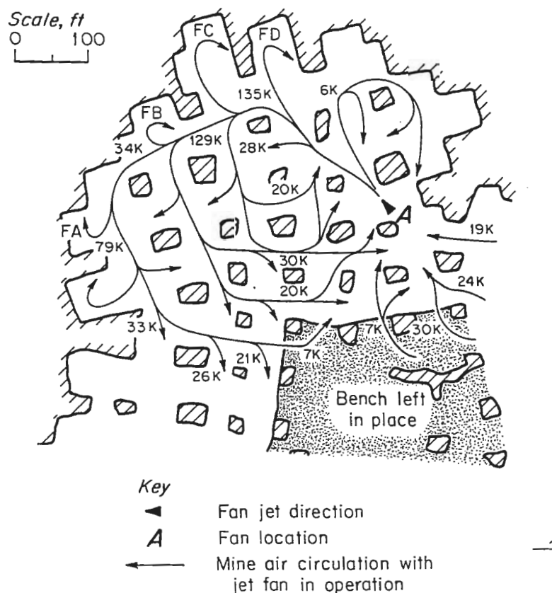
Figure 4. Airflows obtained with jet fan in operation.
