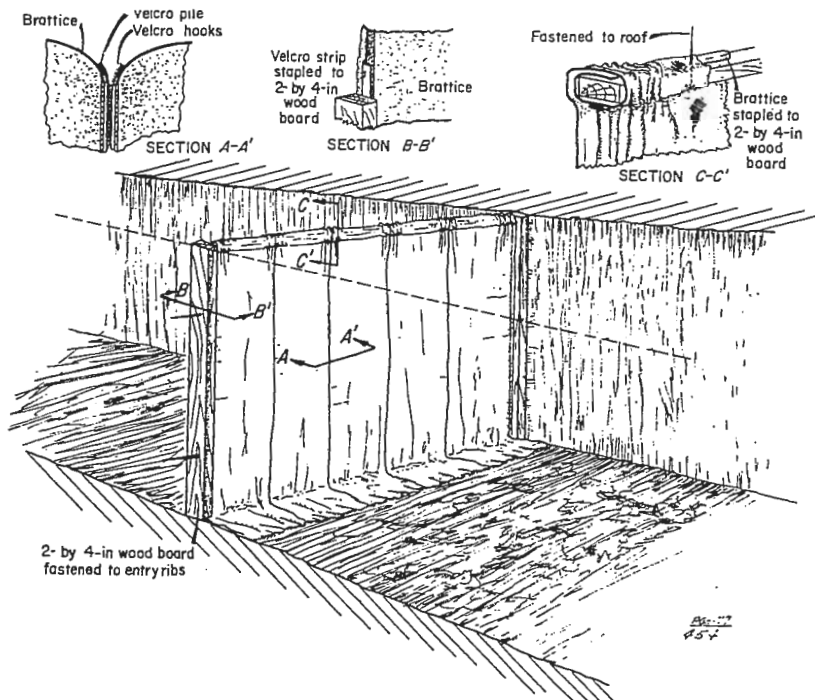
Figure 5. Stopping constructed from damage-resistant brattice.
