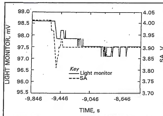
Figure 4: Sensor SA and light monitor response to diesel emissions for experiment No 4
