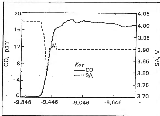
Figure 2: CO and sensor SA response to diesel emissions for experiment No 4
