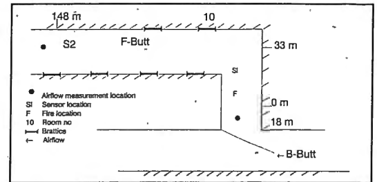
Figure 1: Plan view of mine section
