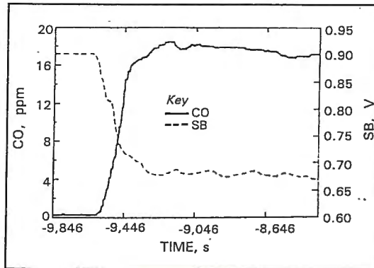
Figure 3: CO and sensor SB response to diesel emissions for experiment No 4
