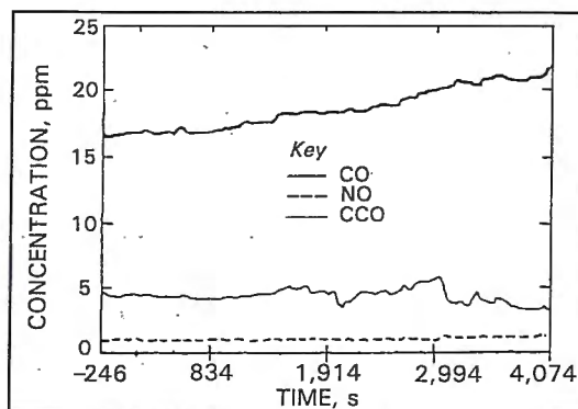
Figure 8: Response of diesel discriminating mine fire sensor SC
