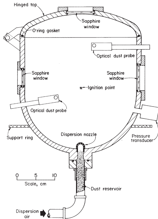
Fig. 4. 20-L laboratory explosibility test chamber.
