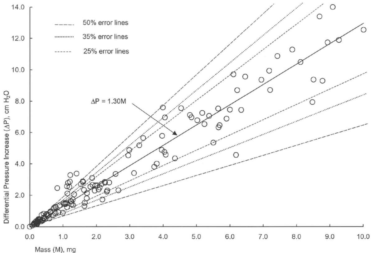
FIGURE 4 Regression for 2 L/min flow rate data, \Delta P = 1.30 M , bracketed by \pm 25\% , \pm 35\% , and \pm 50\% lines.
