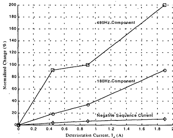
Fig. 2. Measured parameters vs. deterioration in the ULM.
