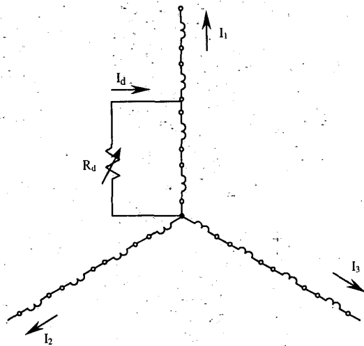
Fig. 1. ULM stator winding with simulated deterioration.
