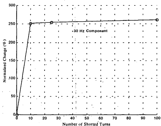
Fig. 4. Bearing vibration vs. rotor winding deterioration.
