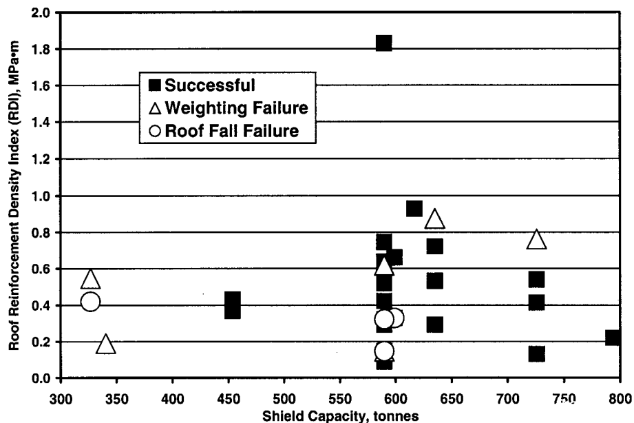
Figure 9. Shield Capacity versus Roof Reinforcement Density Index, indicating results of the mine through.
