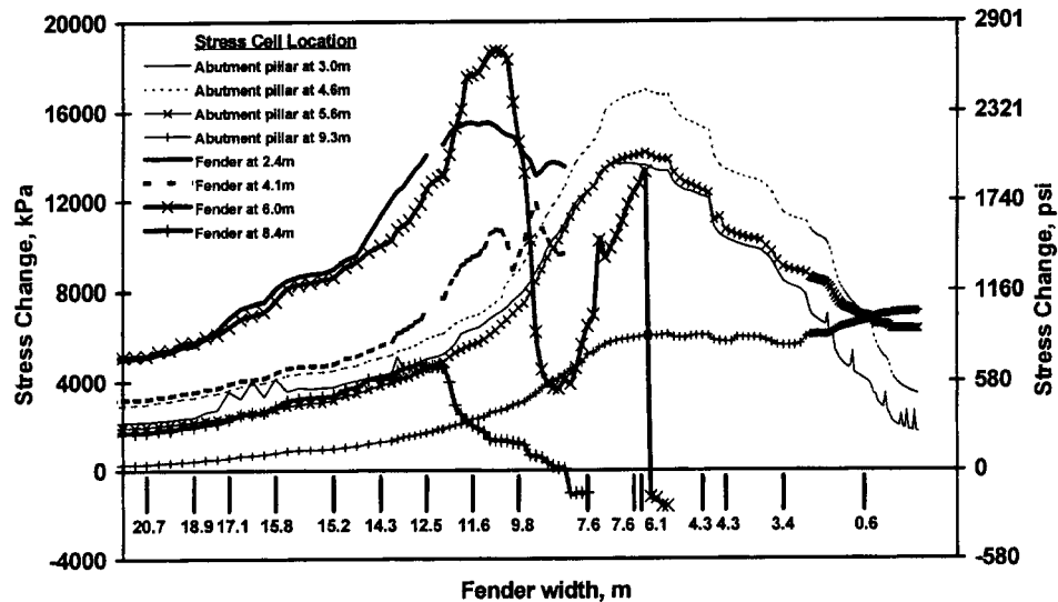
Figure 13. Pennsylvania mine "B". Stress changes measured by vibrating wire stress cells installed in the longwall panel and mid face abutment pillar.
