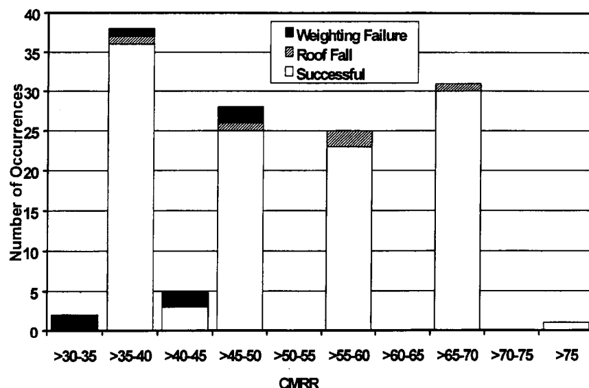
Figure 3. Histogram of CMRR versus mine through occurrences, and indicating results of the mine through.
