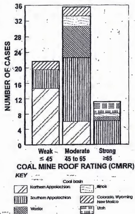
Fig. 5. Geographic distribution of CMRR measurements in the U.S.
