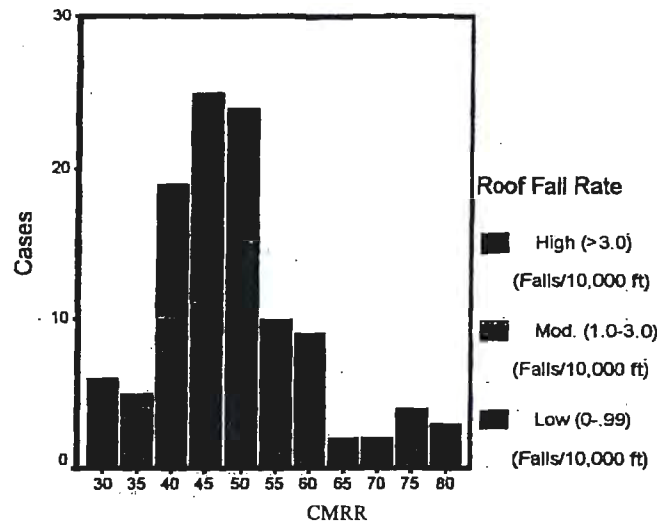
Fig. 10. Relationship between the CMRR and roof fall rate (1 metre = 3.28 ft).
