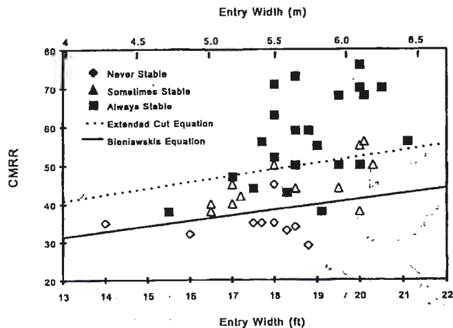
Fig. 9a. Relationship between CMRR and entry width for extended cut roof data.
