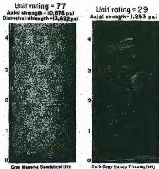
Fig. 4. Rock units with firm number and rock strength (1 mega pascal = 145 pounds/ft 2 ).
