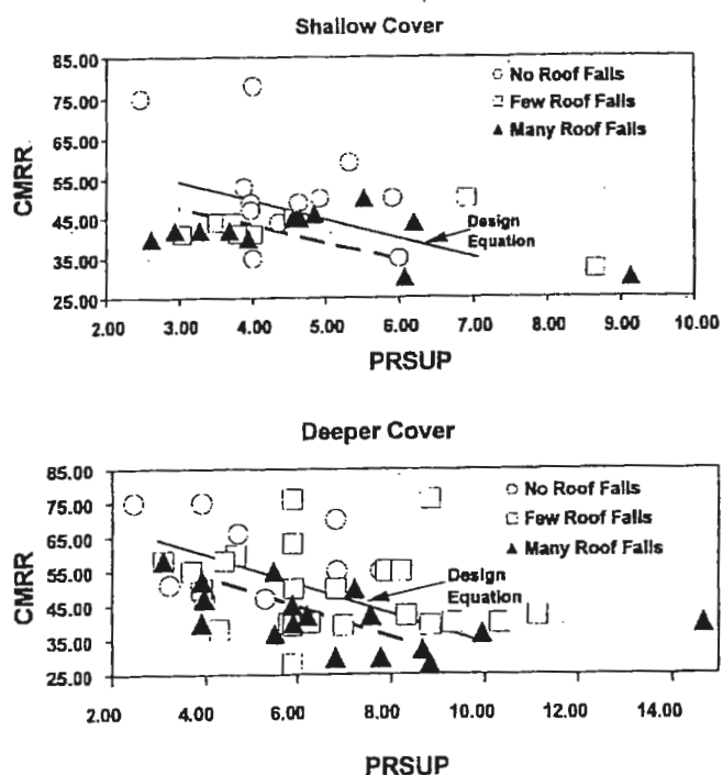
Fig. 12a. Design equations for selecting bolt pattern and capacity. The field data used in the derivation of the formulas are shown along with the original "discriminate equations" (dotted line). Deeper cover (depth>120m).
