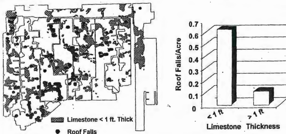
Fig. 8. Map of an Illinois mine showing limestone thickness and roof falls (1 acre = 0.405 hectare and 1 metre = 3.28 ft).
