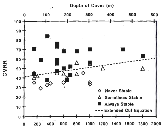
Fig. 9b. Relationship between CMRR and depth of cover for extended cut roof data.
