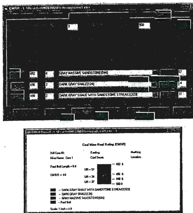
Fig. 14. Output of the CMRR visual basic program (1 metre = 3.28 ft and 1 inch = 2.54 cm).
