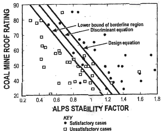
Fig. 13. Relationship between the CMRR and ALPS stability factor in U.S. tailgates.
