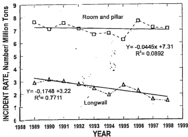
Fig. 2. Comparison of longwall and room and pillar injury rates.
