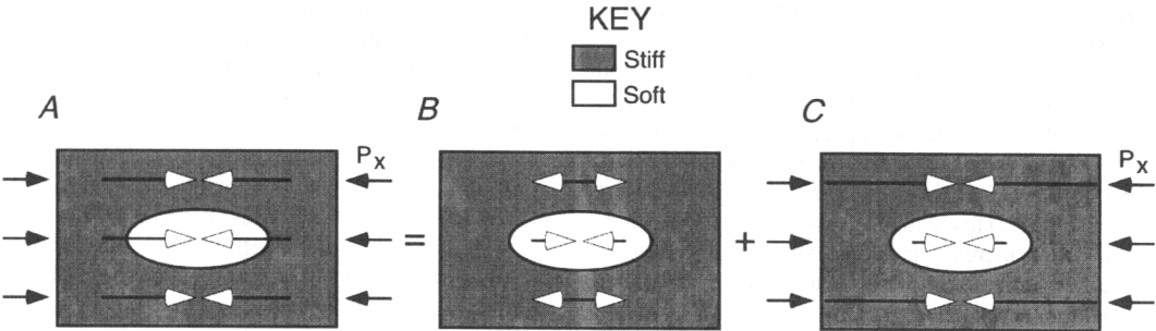
Figure 3.—Tectonic (B) and residual (C) components of a uniform stress field in an elastic model of an elliptical soft inclusion (A).
