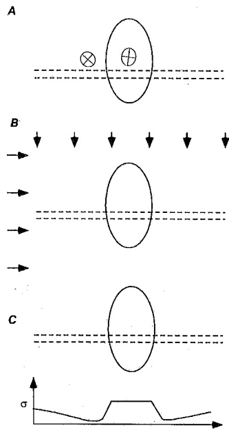
Figure 1.—Outline of modeling method. Stress measurements (A) are analyzed in light of lithologic inclusions to find regional loads (B). Loads are thus applied to the model to determine stresses in the region of interest, in this case, the course of a planned tunnel or mine drift (C).
