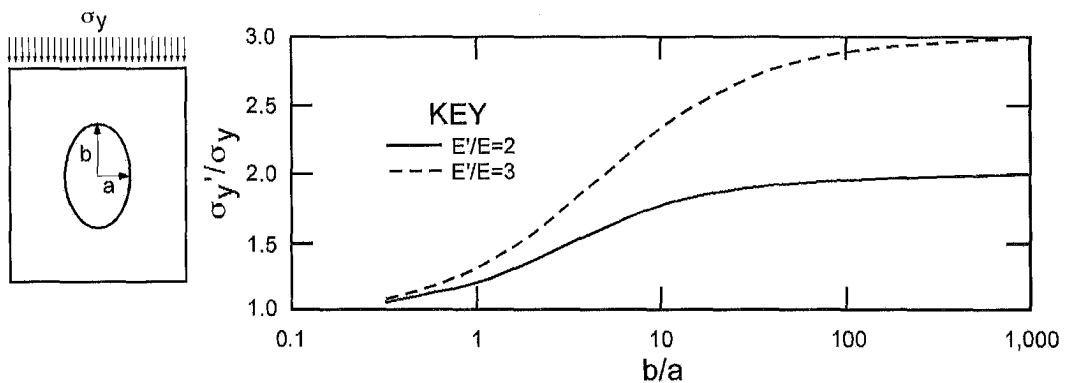
Figure 2.—Stress-concentrating effect of elliptical inclusion (plane stress).
