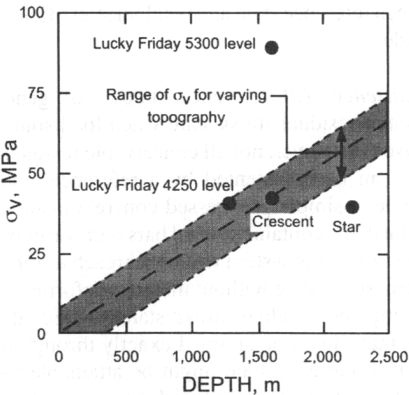
Figure 4.—Observed magnitude of vertical stress from four in situ stress measurements at various depths. Variability that can be attributed to topography is indicated by the shaded region.
