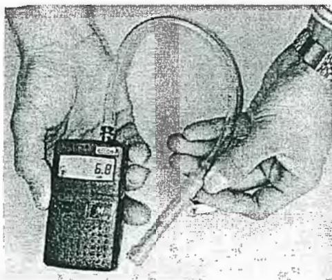
Figure 2. Respirable dust dosimeter showing pump with pressure readout and new plastic dust detector tube
