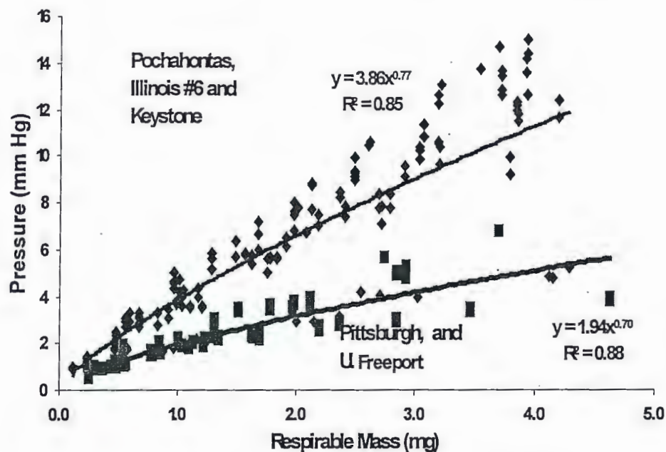
Figure 4. Dust dosimeter data for all laboratory results
