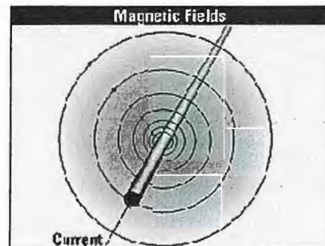
Figure 1. Magnetic fields.
