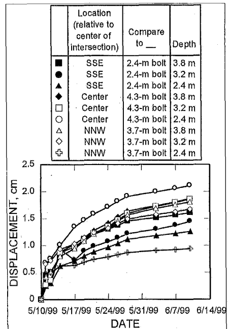
Figure 8.—Displacement of back over time.
