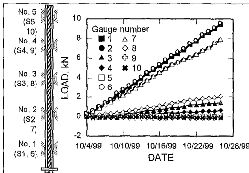
Figure 10.—Load on bolt 4 at Getchell Mine.
