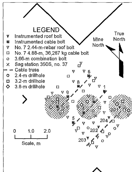
Figure 5.—Bolt and sagmeter locations.
