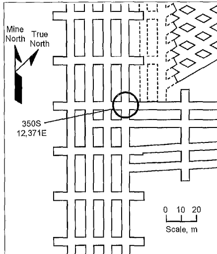
Figure 4.—Instrument locations in trona mine.
