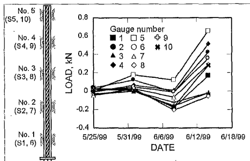
Figure 11.—Load on bolt 14 at K-2 Mine.
