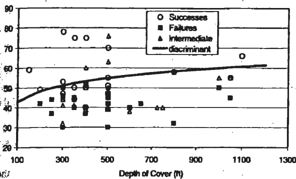
Figure 4. Support mechanisms in practice. Above the discriminant line is the skin support/suspension regime; below the line is the beam building/supplemental support regime.
