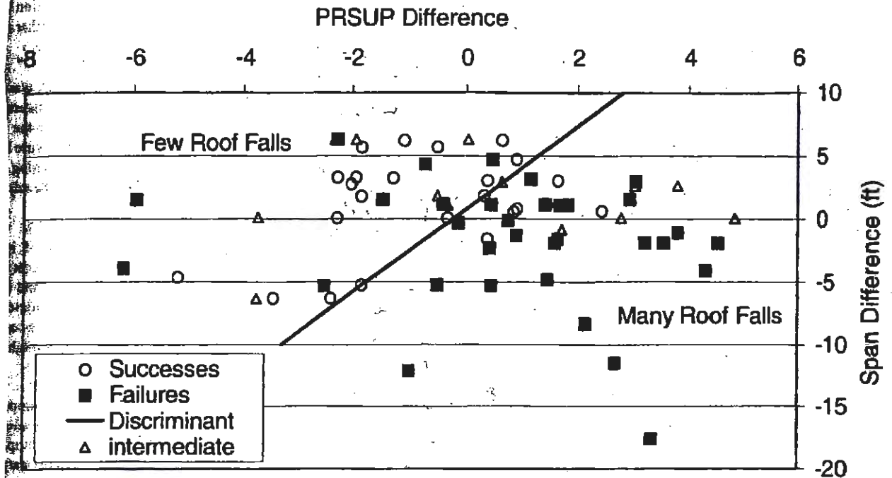
Figure 9. Verification of the design equations (3), (6), and (7). The case histories are plotted according to the difference between the actual PRSUP and the calculated PRSUP (X-axis), and between the actual span and the calculated span (Y-axis). The discriminant line is equation (7)
