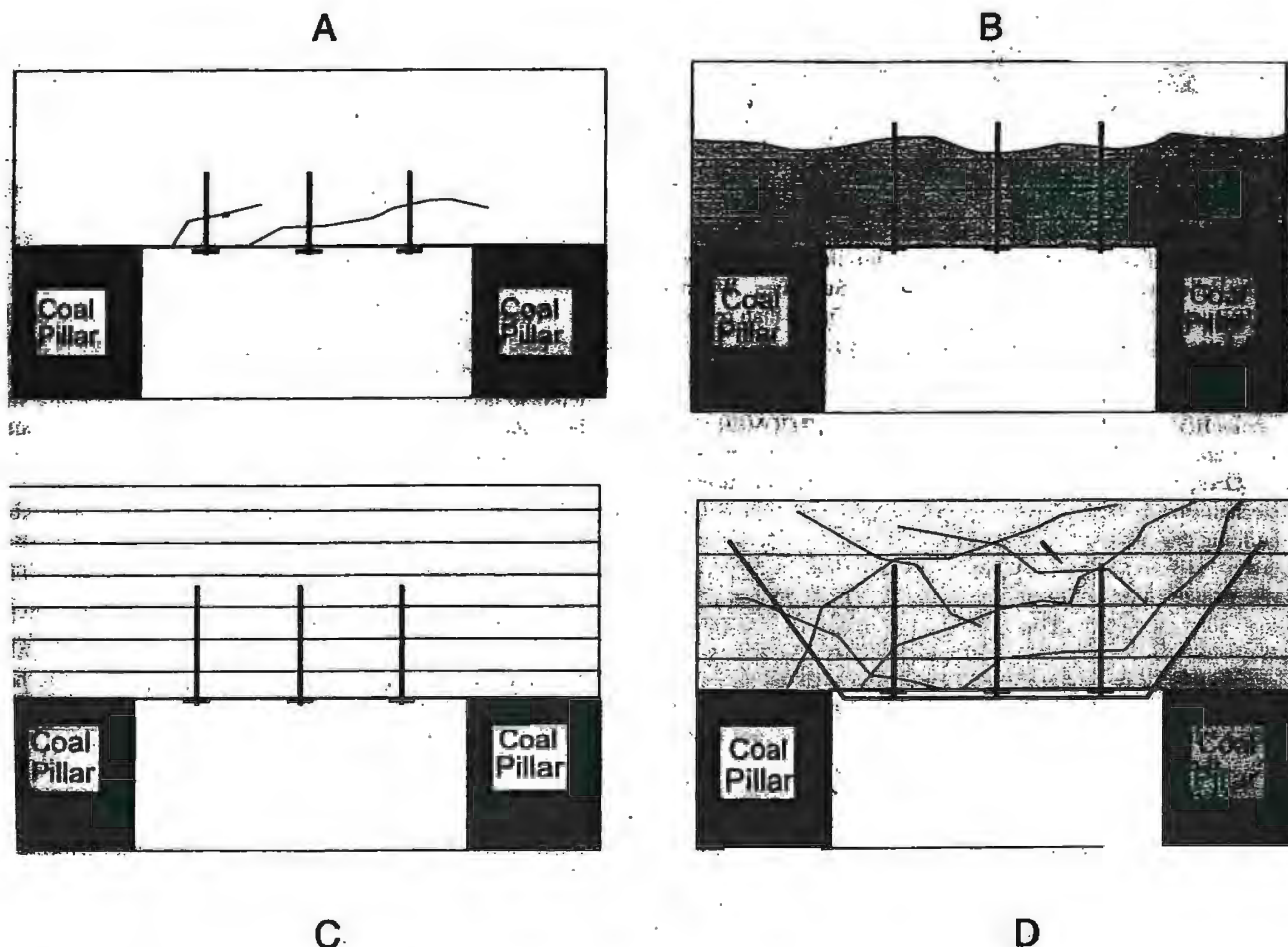
Figure 1. Roof bolt support mechanisms: (A) simple skin support, (B) suspension, (C) beam building, and (D) supplemental support in failing roof.
