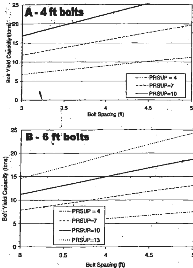
Figure 10. PRSUP design charts relating the bolt spacing to bolt yield capacity. Based on 4 bolts per row and 18 ft wide entries. (A) Bolt length = 4 ft and (B) Bolt length = 6 ft
