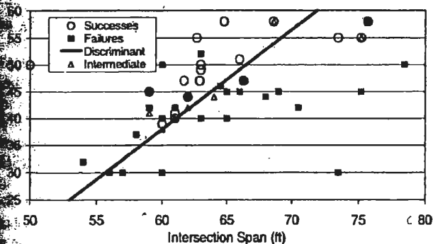
Figure 5. Effect of roof span on roof fall rate. Above the line spans are appropriate, below the line spans are generally too wide.
