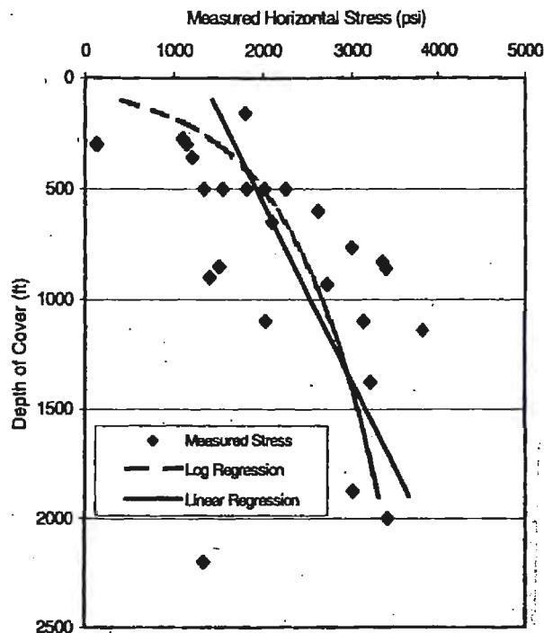
Figure 3. Horizontal stress in eastern U.S. coal mines. Actual stress measurements from Mark and Mucho (9).
