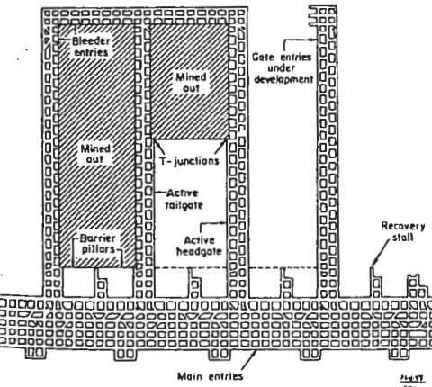
Figure 3. Plan view of a typical U.S. longwall mine.
