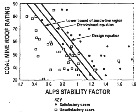
Figure 4. ALPS case history data base and design guidelines.
