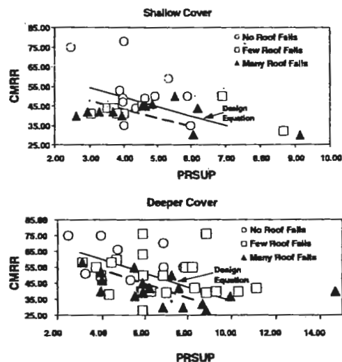
Figure 10. Design equations for roof bolts.
