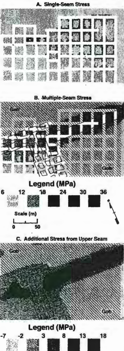
Figure 8. Stress analysis of multiple seam interaction using LAMODEL.
