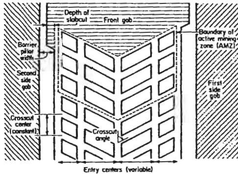
Figure 5. Model of a room-and-pillar mining section used by the ARMPS program.
