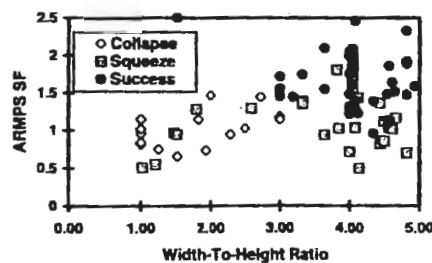
Figure 7. Pillar collapse case histories in the U.S.
