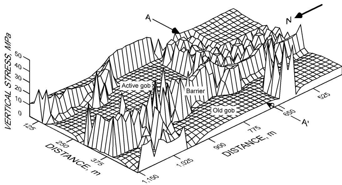
Figure 6.—Vertical stress distribution on the Tank Seam.
