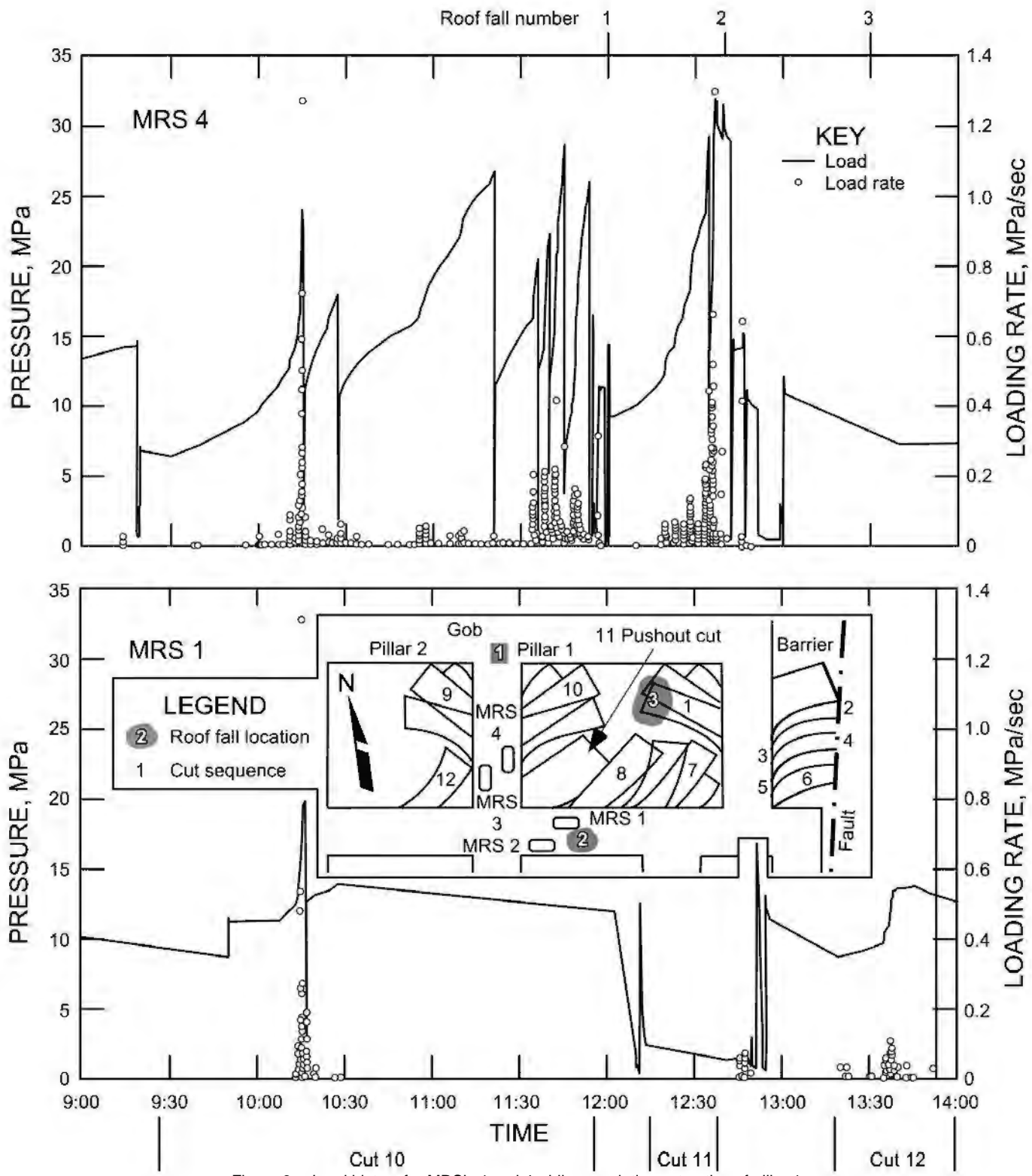
Figure 8.—Load history for MRS's 1 and 4 while completing extraction of pillar 1.
