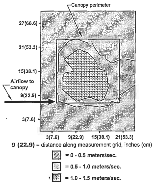
Figure 3. Velocity contours for canopy flow = 0.094 m 3 /s, 30.5 cm beneath canopy
