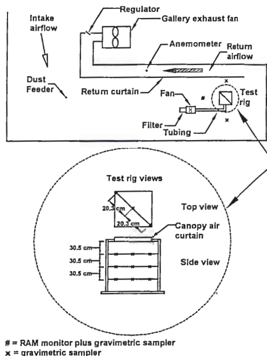
Figure 1. Experimental setup
