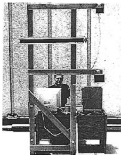
Figure 5. Photograph of the prototype interferometric radar system. The transmit antenna is seen in the center and the receive antennas are on the top-right and bottom-right.
