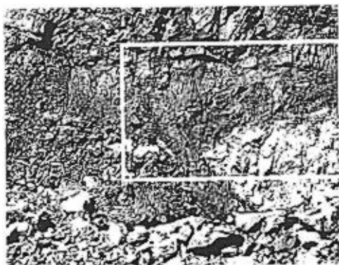
Figure 3. West highwall of the Mountain Pass Main Pit. Study area is outlined.
