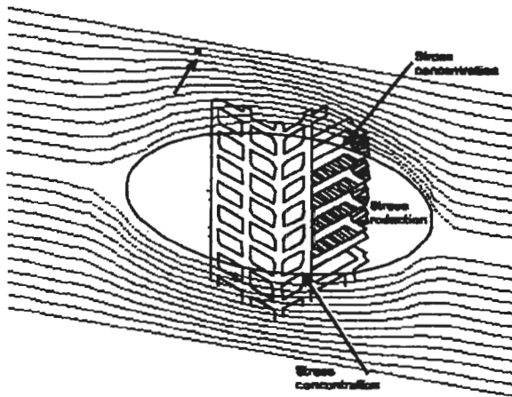
Figure 6. Plan view of stress distribution around pillaring and cave with reference to a N 70° E direction of the maximum horizontal stress
