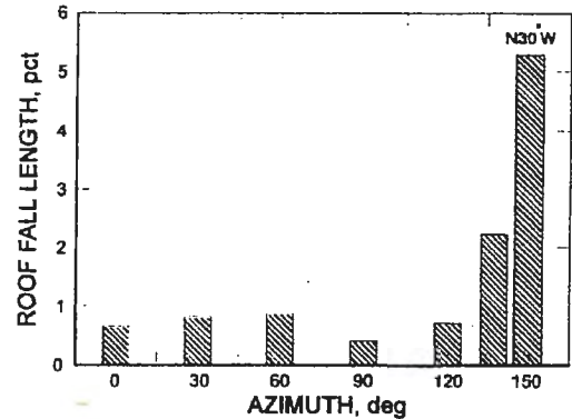
Figure 3. Direction of failed roof normalized by dridge in a given direction
