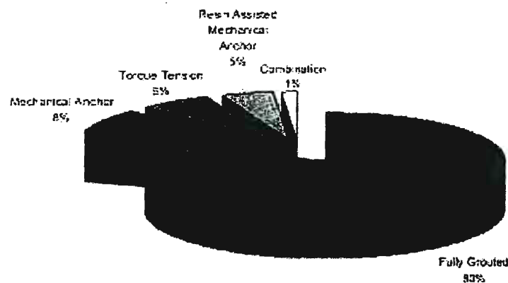
Figure 1: Percentage of a bolt type used in underground coal mines, 1999
