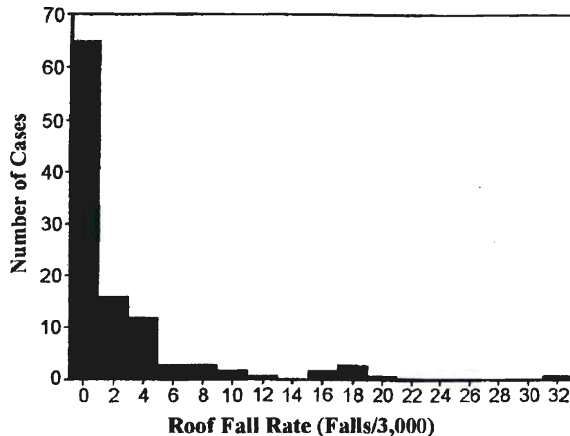
Figure 5: Distribution of roof fall rates in the study sample
