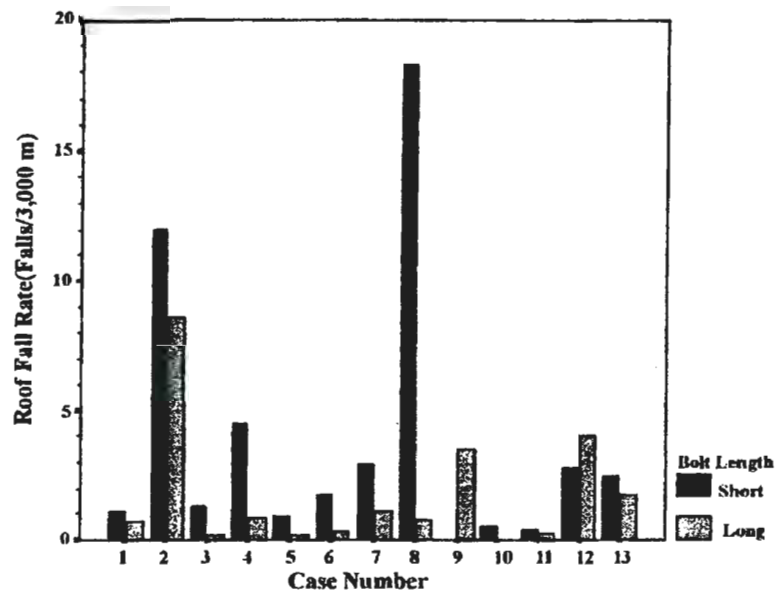
Figure 7: Paired cases of long and short bolts showing benefit of long bolts and decreasing roof fall rates.
