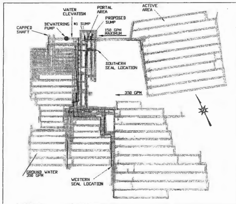
Figure 1 Mine Map With Flow Diagram
