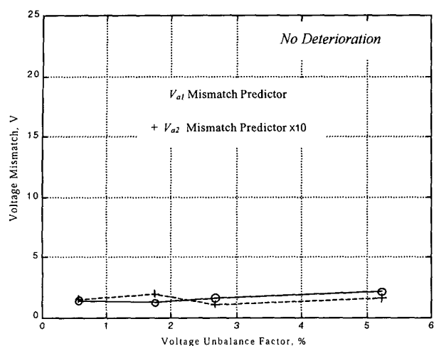
Figure 2. Illustration of the insensitivity of the voltage mismatch predictors to different levels supply unbalances for a nondeteriorated induction motor.
