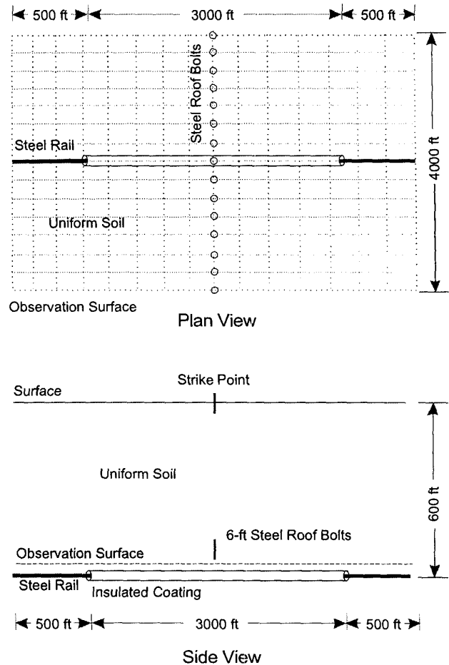
Fig. 2. Simulation model for Fig. 1.
