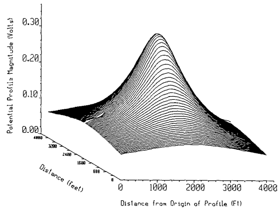
Fig. 4. Per-unit scalar potentials at dc for Scenario 1.
