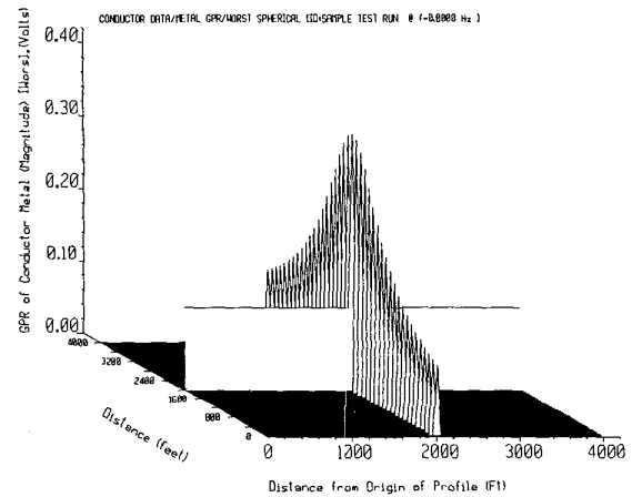
Fig. 9. GPR of rail and roof bolt segments at dc for Scenario 1.
