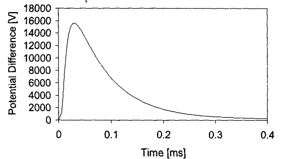
Fig. 18. Potential difference for Scenario 2.
