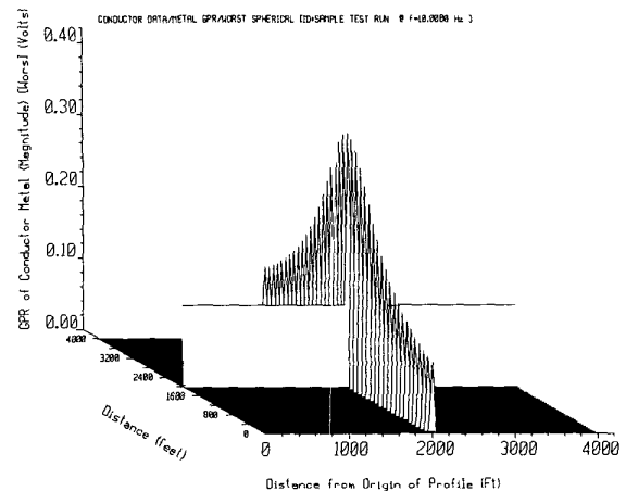
Fig. 10. GPR of rail and roof bolt segments at 10 Hz for Scenario 1.
