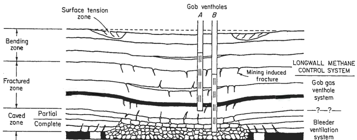
Figure 3. Schematic cross-section view of subsided strata zones and methane control system influence zones above mined-out longwall panel (modified from Peng and Chiang, 1984 and Singh and Kendorski, 1981).
