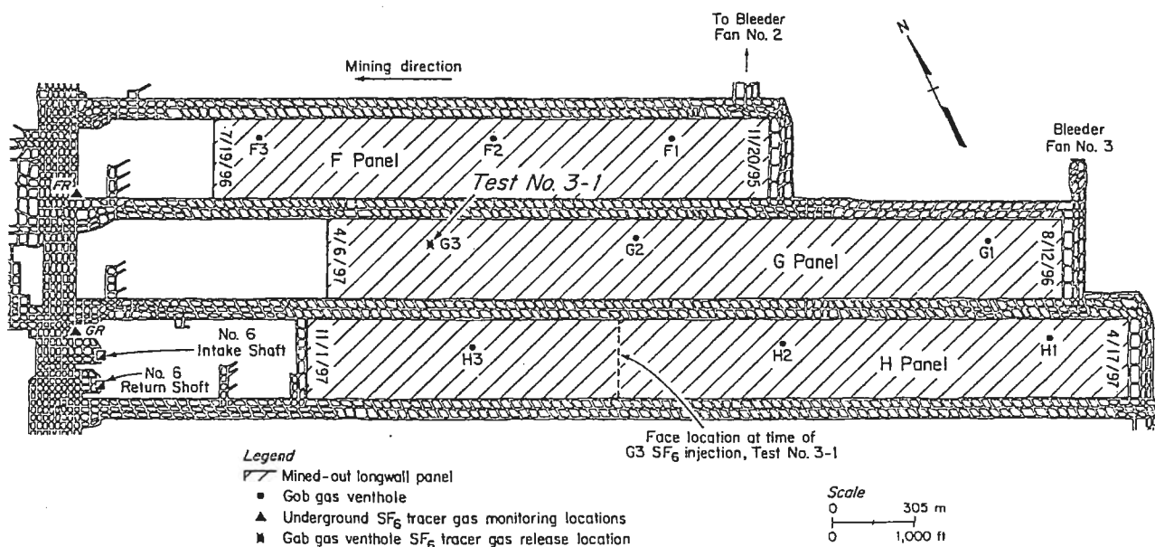
Figure 8. Detailed map of F, G, and H longwall panel area at time of the G3 gob gas venthole tracer gas injection test.
