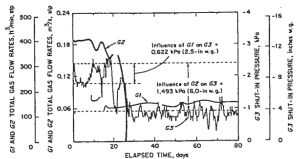
Figure 10. Influence of gob gas venthole production on G3 shut-in pressure.
