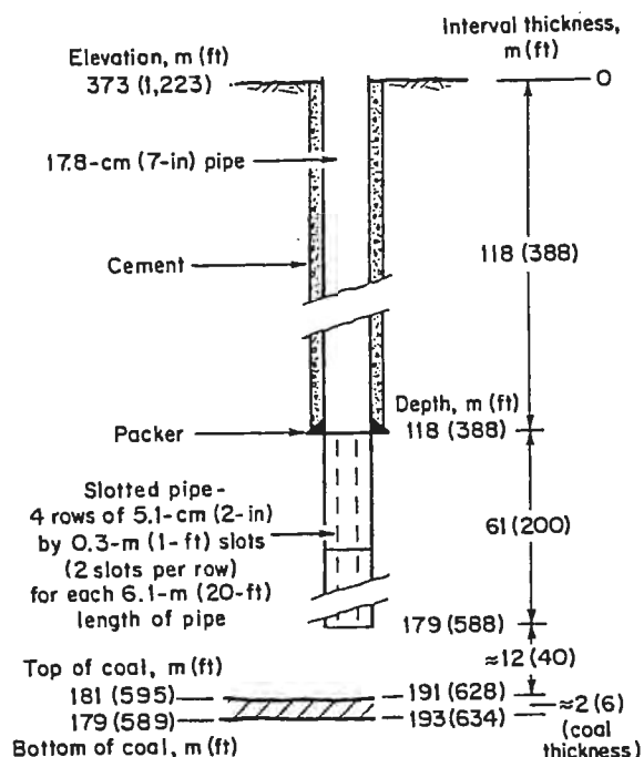
Figure 7. Schematic of gob gas venthole G3 configuration.
