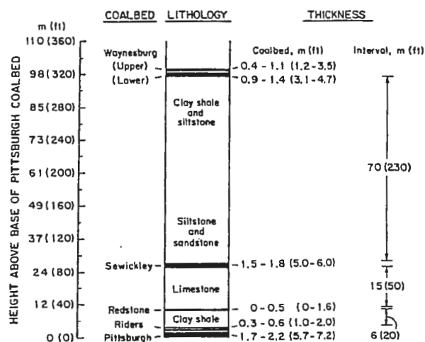
Figure 2. Generalized stratigraphic section for study area.
