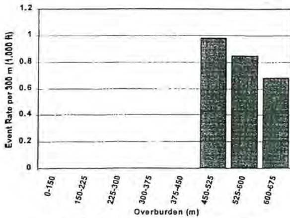
Figure 2. Event rate per 300 m (1,000 ft) vs overburden at Mine A
