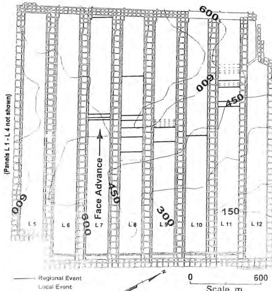
Figure 1 Panel and face locations of Regional and Local events at Mine A
