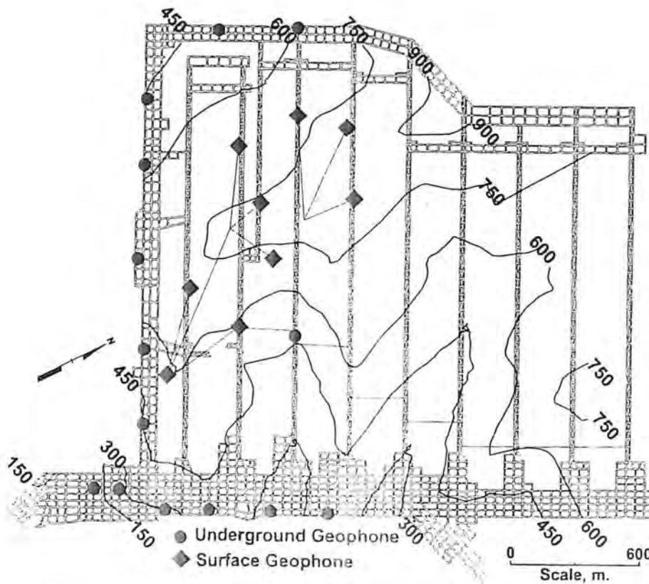
Figure 9. Mine outline showing locations of surface and underground geophones
