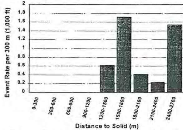
Figure 4. Event rate per 300 m (1,000 ft) vs distance to solid in meters at Mine A
