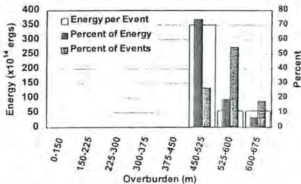
Figure 6. Distribution of energy per event, percent of energy, and percent of events at Mine A
