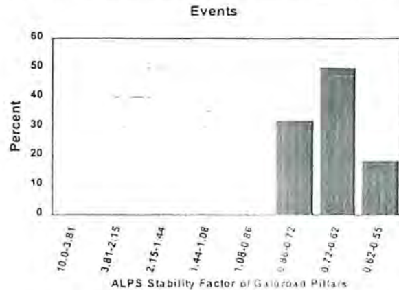
Figure 5. Percentage distribution of events by ALPS stability factor of gateroad pillars
