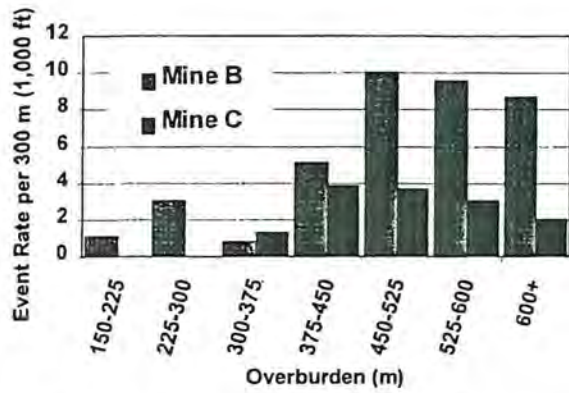
Figure 7. Event rate per 300 m (1,000 ft) versus overburden at Mines B and C
