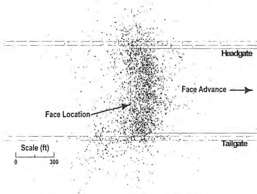
Figure 10. Plan view of event locations, normalized to face location
