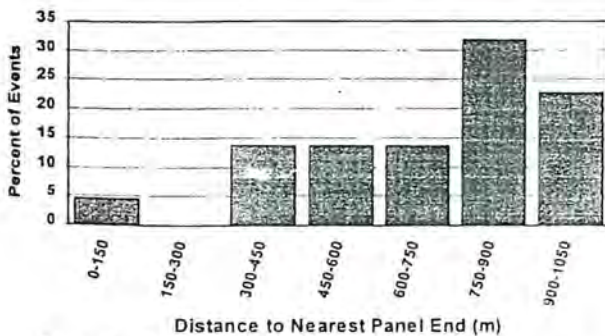
Figure 3. Distribution of events occurring at Mine A relative to the nearest panel end of the longwall panels
