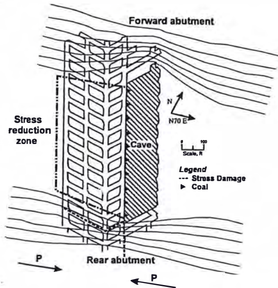
Figure 17. "Advance and relieve" panel with cave showing the forward and rear abutments and stress reduction zone
