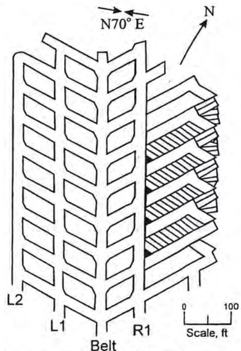
Figure 5. Plan view of E15 panel showing "advance and relieve" pillaring
