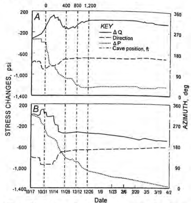
Figure 15. Horizontal stress changes measured at the test site. (a) 2-ft depth and (b) 10-ft depth. The azimuth direction is to \Delta Q
