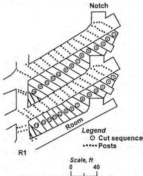
Figure 9. Second pillaring plan used in E15 and E17 panels
