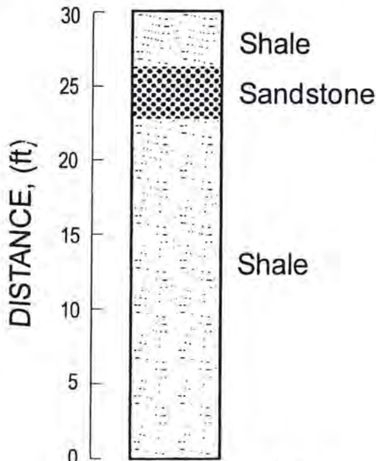
Figure 2. Roof geology in the E-mains and panels
