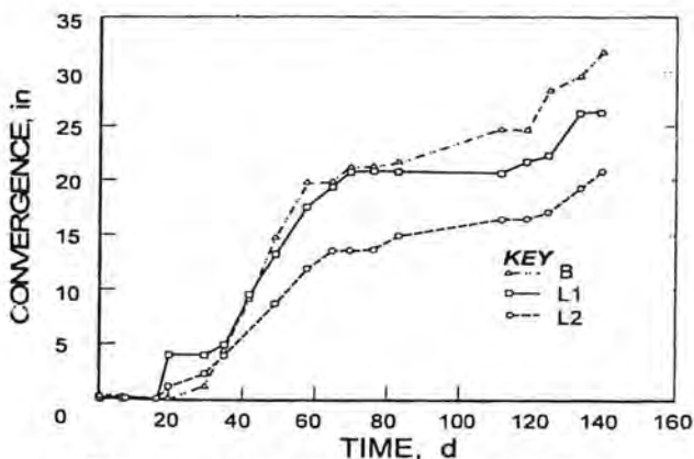
Figure 13. Floor heave rates across E17 panel
