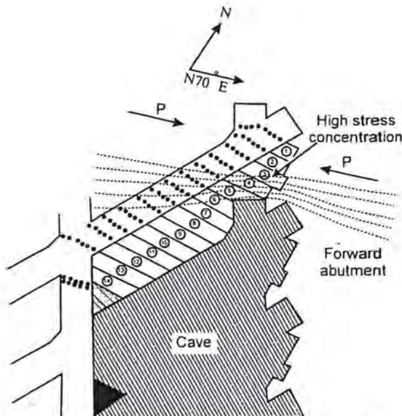
Figure 10 Forward horizontal stress abutment and concentration with respect to the second pillaring plan
