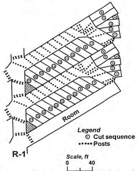
Figure 7: Original pillaring plan used in E15 panel
