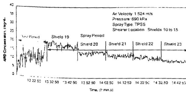
Figure 2. Typical RAM-1 output from a test along the longwall gallery
