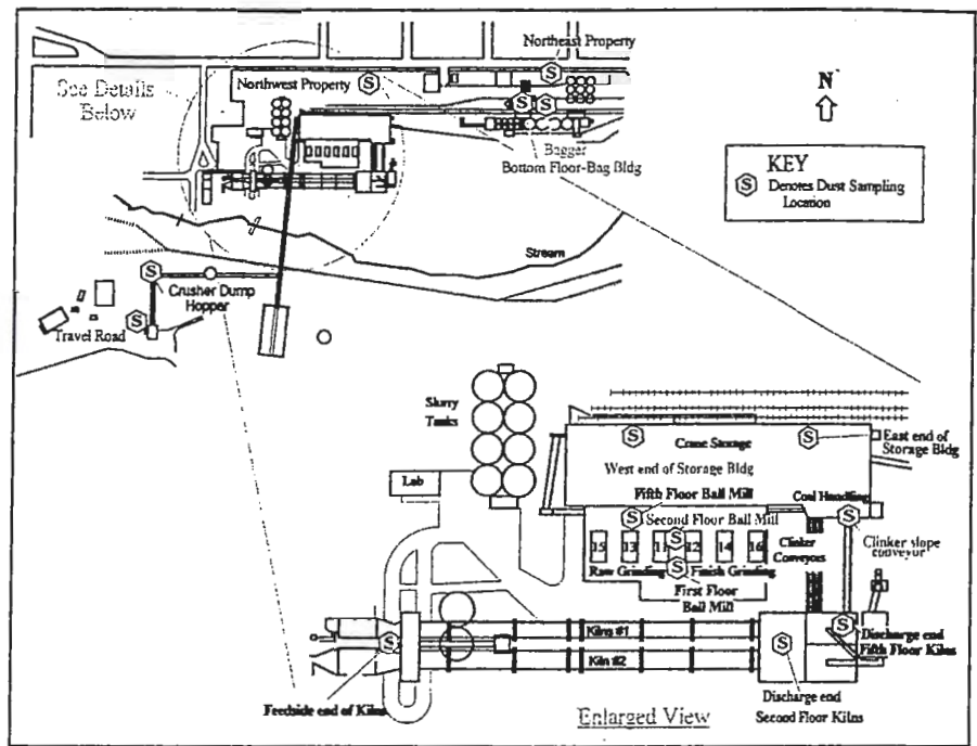
Figure 3. Dust Monitoring Locations at Wet Processing Plant
