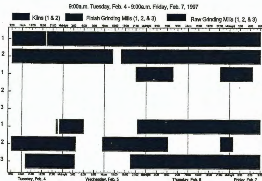
Figure 5. Operating Time of Kilns and Ball Mills
