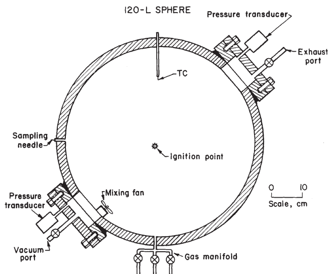
Fig. 1. 120 L flammability test sphere.
