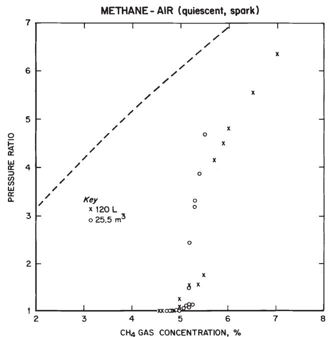
Fig. 6. Lean limit flammability data for quiescent mixtures of methane in air in 120 L chamber, compared to earlier data from 25.5 \text{m}^3 chamber (Burgess et al., 1982) and to dashed curve for calculated adiabatic values.
