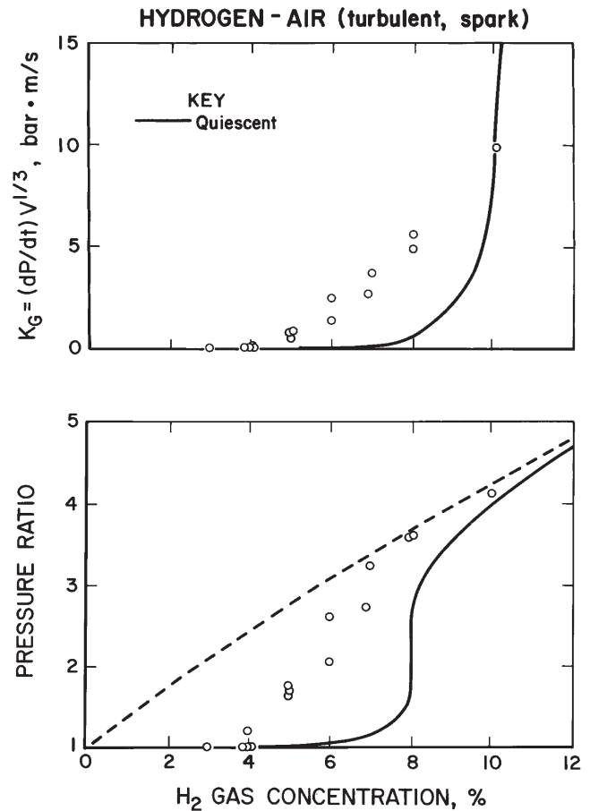
Fig. 13. Flammability data (open circles) near the LFL for “turbulent” mixtures of hydrogen in air in 120 L chamber, compared to solid curve for quiescent experimental data and to dashed curve for calculated adiabatic values.
