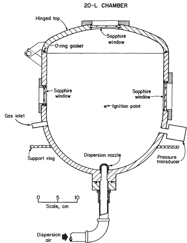
Fig. 2. 20 L flammability test chamber
