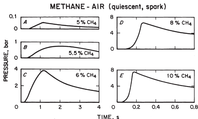
Fig. 3. Pressure-time traces for mixtures of (A) 5% CH 4 in air, (B) 5.5% CH 4 in air, (C) 6% CH 4 in air, (D) 8% CH 4 in air, and (E) 10% CH 4 in air.
