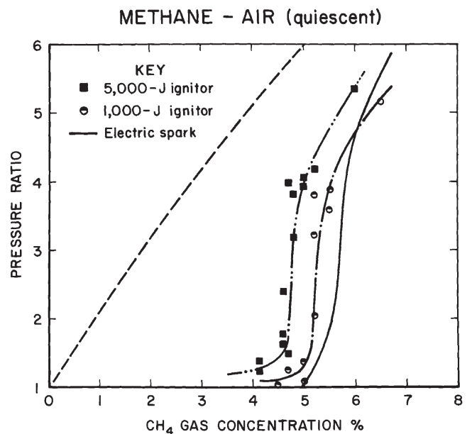
Fig. 8. Flammability data for quiescent mixtures of CH 4 in air in 120 L chamber, using 1000- or 5000 J pyrotechnic ignitors, compared to solid curve for spark data and to dashed curve for calculated adiabatic values.
