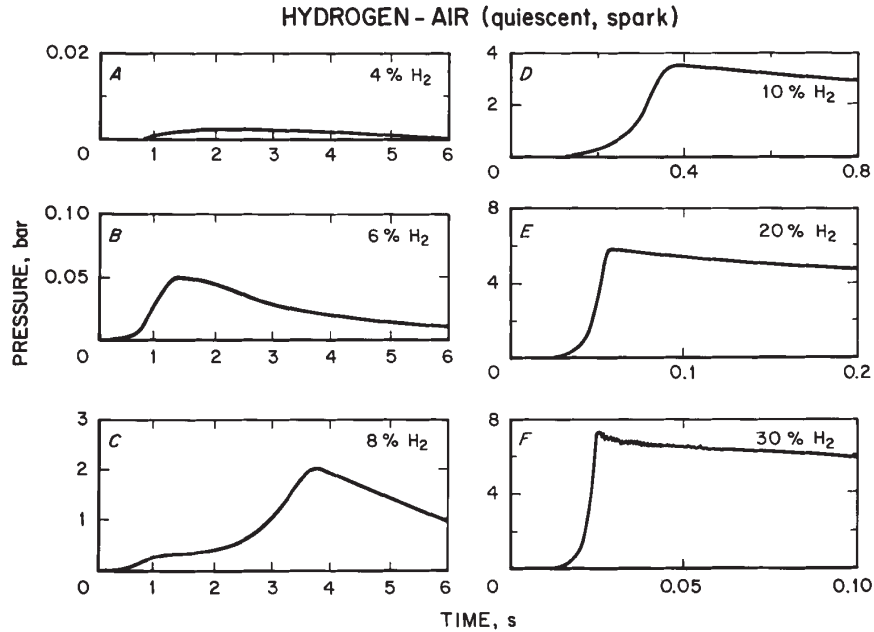
Fig. 4. Pressure-time traces for mixtures of (A) 4% H 2 in air, (B) 6% H 2 in air, (C) 8% H 2 in air, (D) 10% H 2 in air, (E) 20% H 2 in air, and (F) 30% H 2 in air.
