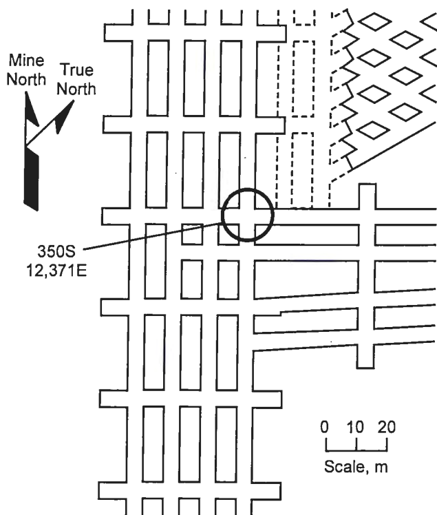
Figure 6.—Instrument locations in mine.
