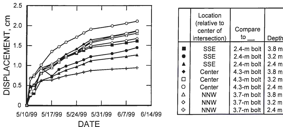
Figure 11.—Displacement of back over time.
