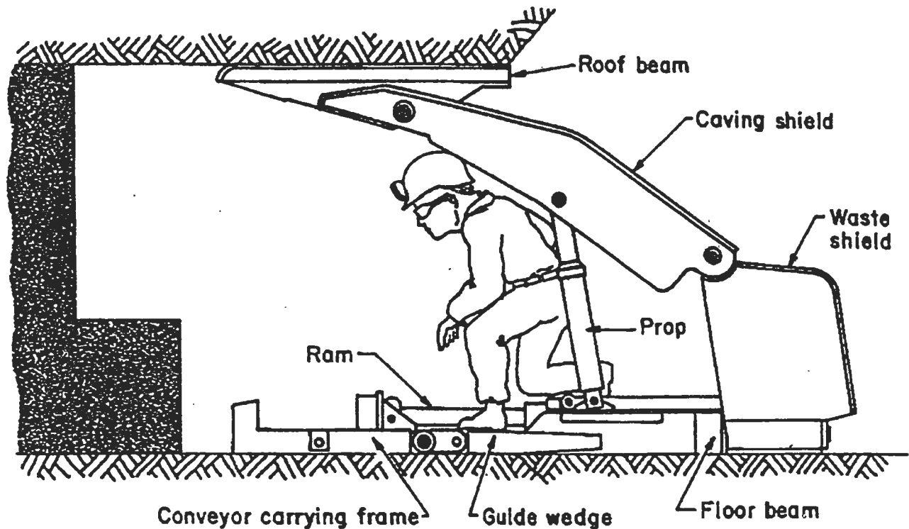
Figure 2. Shield-type roof support.
