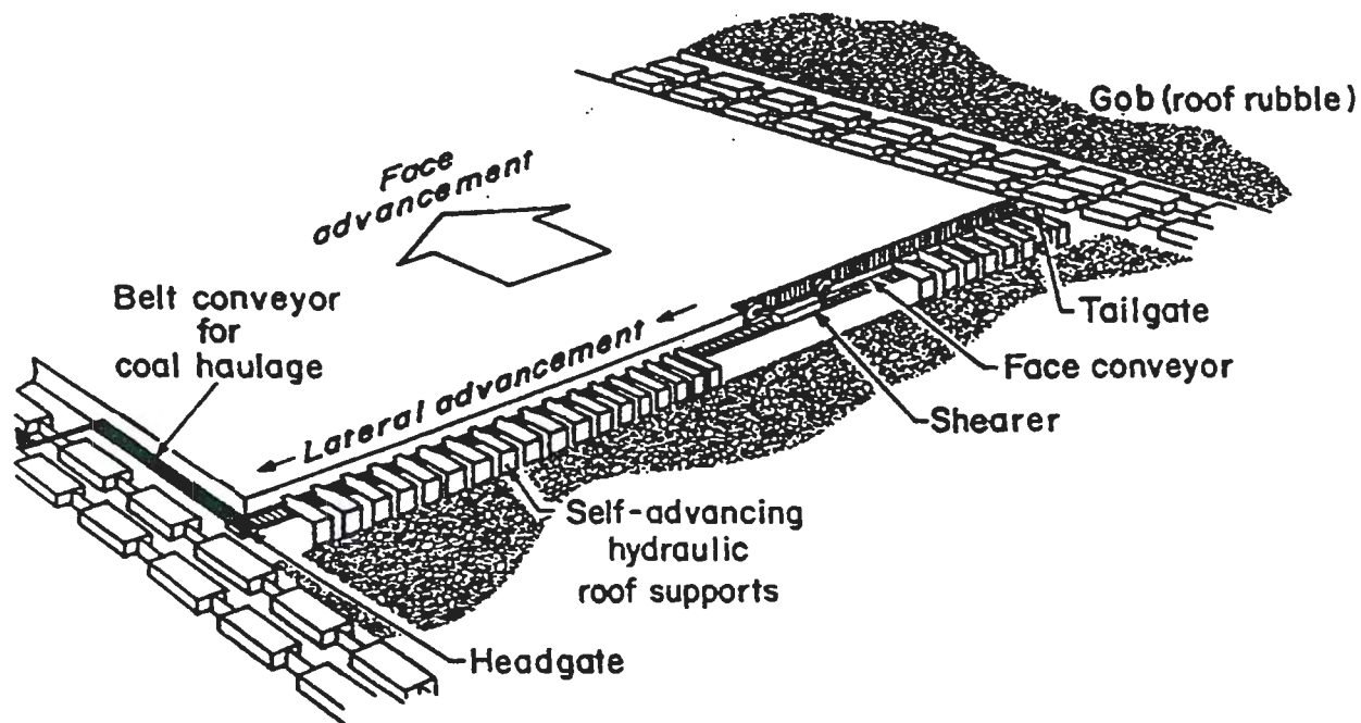
Figure 1. Basic components on a longwall face.
