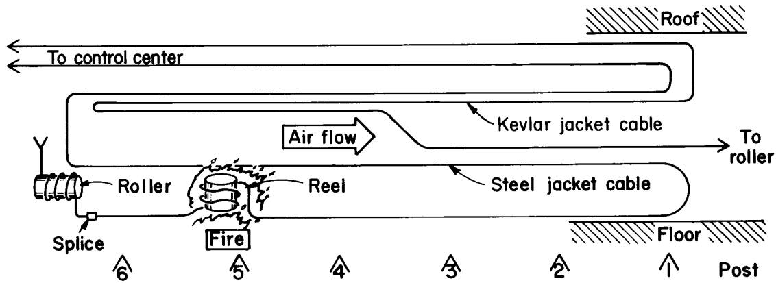
Fig. 6. The test arrangement at Lake Lynn.
