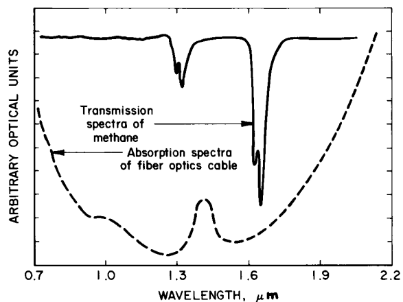
Fig. 2. Fiber optic window and methane absorption peak.
