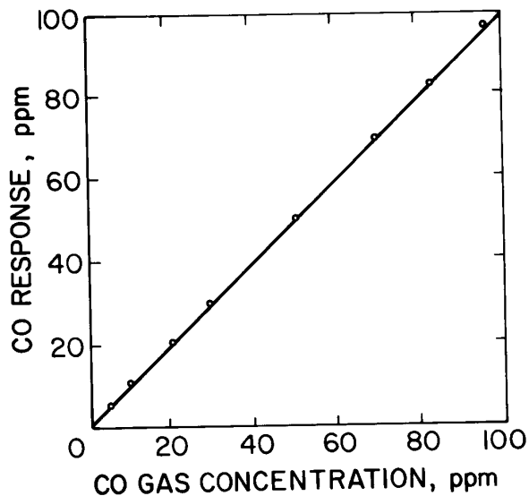
Fig. 5. CO Monitor output linearity.
