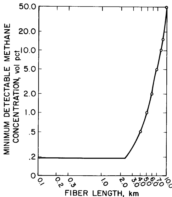
Fig. 3. Minimum detectable methane concentrations.
