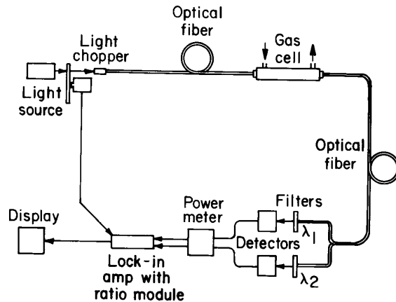
Fig. 1. Fiber optic methane monitor.
