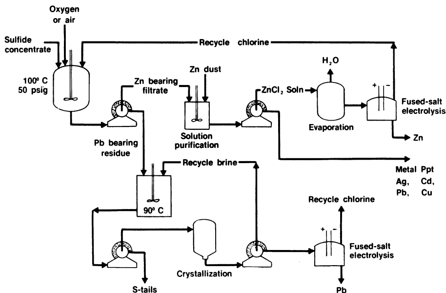
Fig. 5. Flowsheet for processing of lead-zinc sulfide concentrates.
