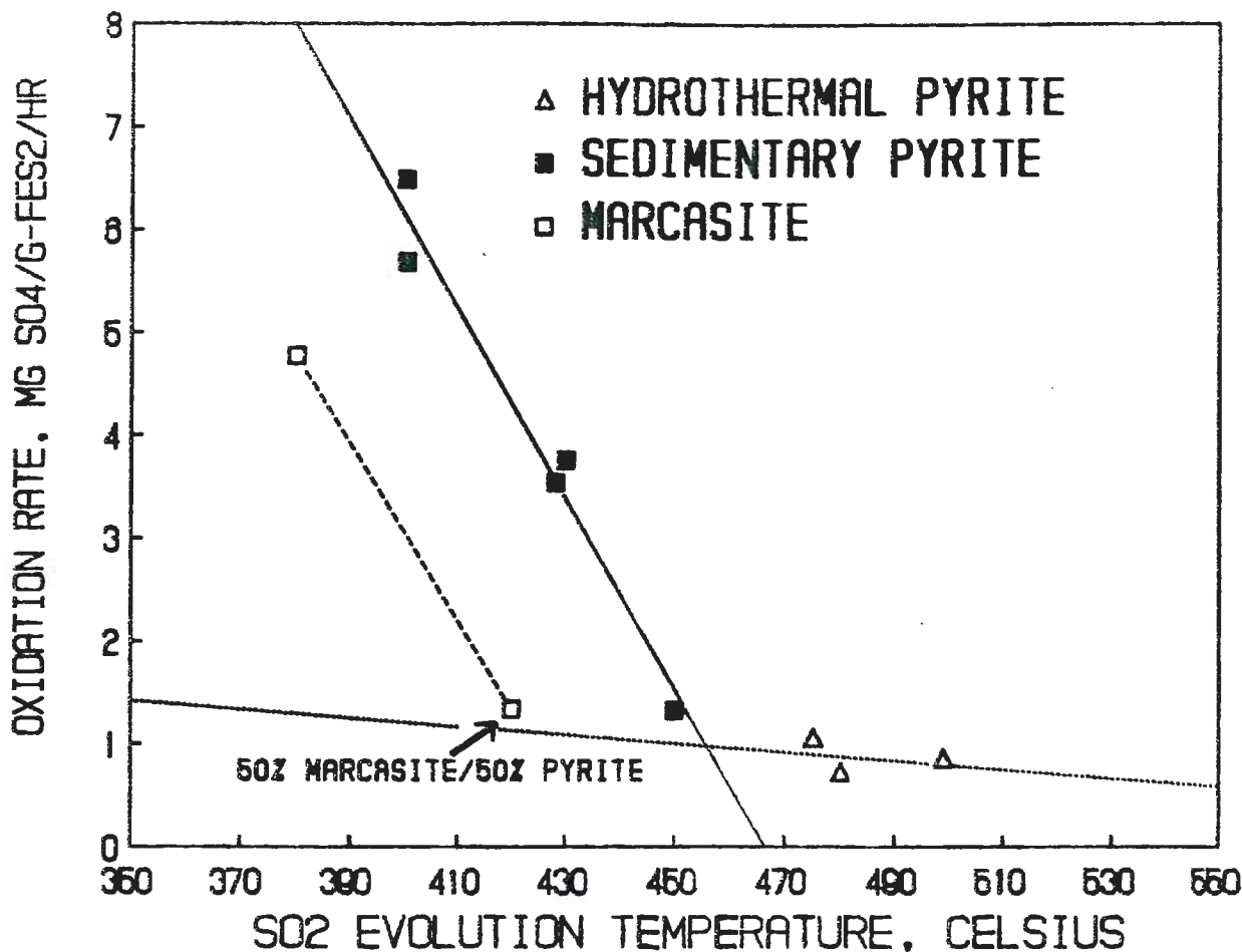
Figure 10. Plot of SO 2 evolution temperature from evolved gas analysis versus XPS monitored weathering rates.
