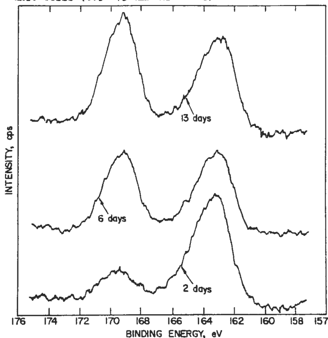
Figure 1. XPS SCAN of the sulfur (2p) region showing pyritic sulfur (B.E. = 163.5eV) and sulfate sulfur (B.E. = 169.5eV) after 2, 6, and 13 days weathering.
