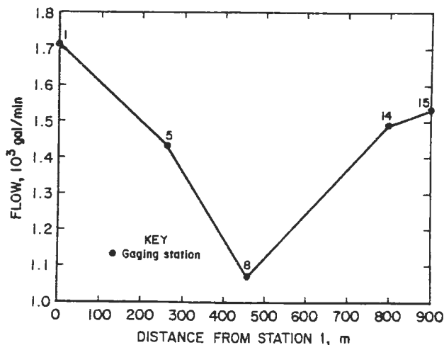
Figure 2.--Mean annual discharge at Staub Run.
