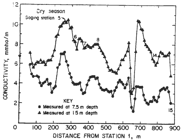
Figure 3.--Conductivity survey (dry season) at Staub Run.
