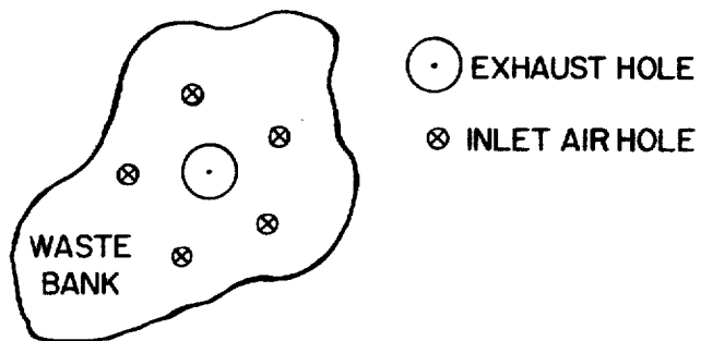
PLAN VIEW OF MULTIPLE BOREHOLE SYSTEM
