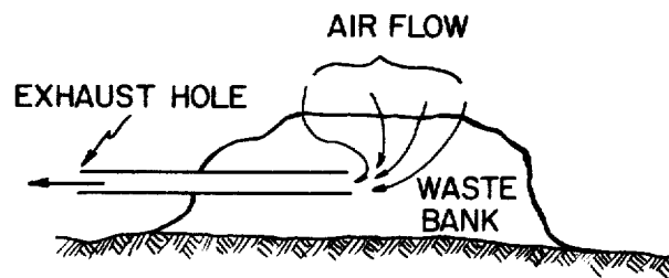
SIDE VIEW OF "BLIND" BOREHOLE SYSTEM
