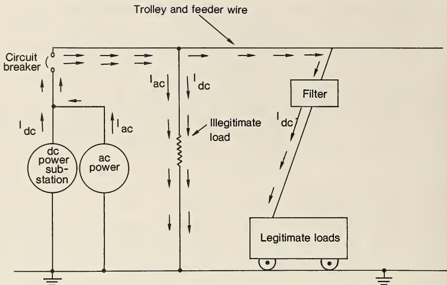
FIGURE 1. - DISCB current flow.
