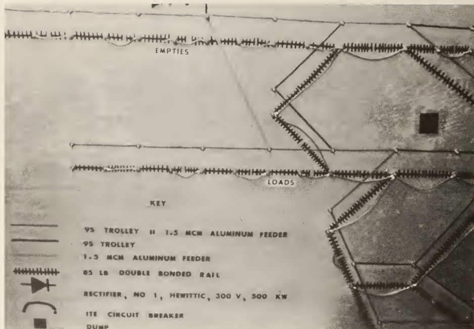
FIGURE 11. - Haulage model.
