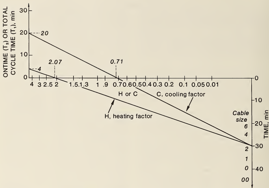
FIGURE 4. - Intermittent duty rating nomograph 2.
