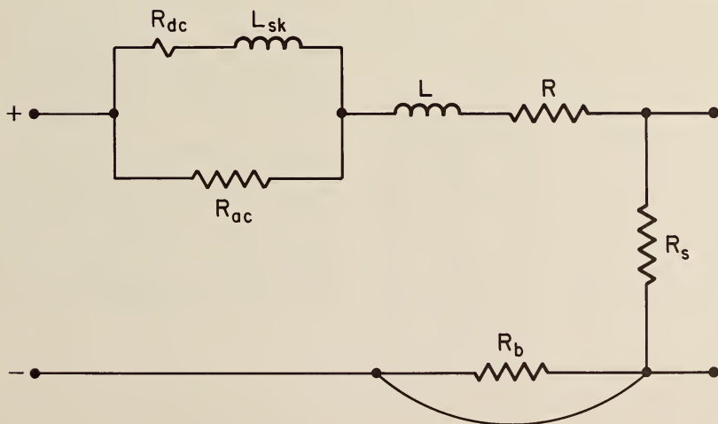
FIGURE 10. - Lumped haulage simulation.
