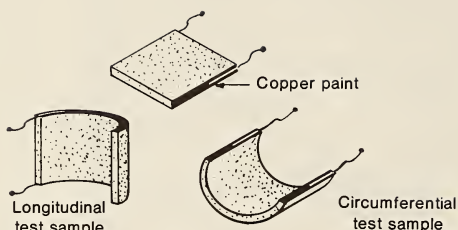
FIGURE 9. - Sample configurations taken from semiconducting shielded cable used to determine volume resistivity, \rho_v .
