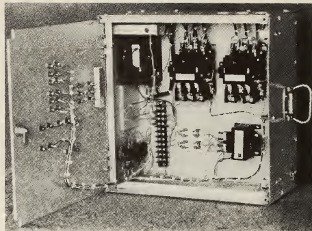
FIGURE 2. - Panel as removed after internal electrical controls are unlocked.
