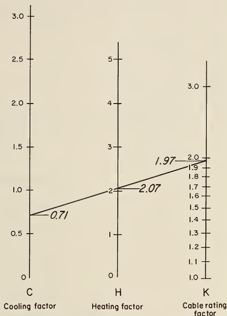
FIGURE 3. - Intermittent duty rating nomograph 1.
