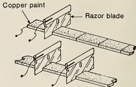
FIGURE 10. - Sample configurations used in measuring \rho_v for semiconducting tape samples.
