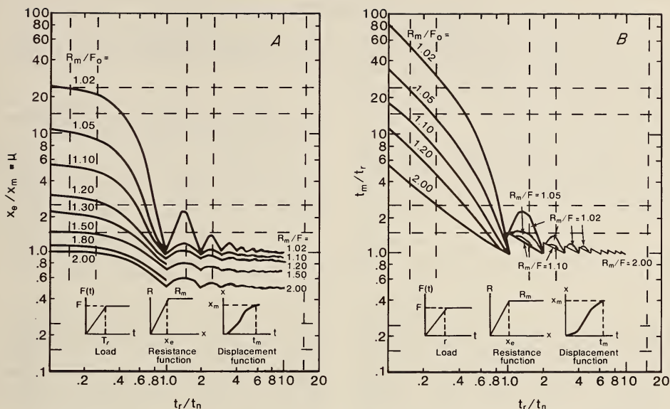
FIGURE 11. - Maximum response of undamped single-degree-of-freedom elastic-plastic system to step pulse with finite rise time (10).
