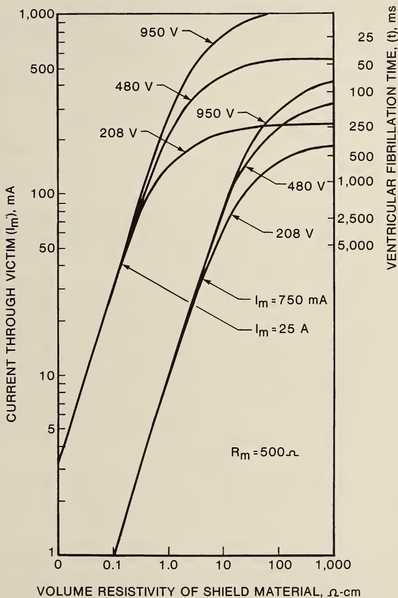
FIGURE 8. - Currents and ventricular fibrillation times versus shield resistivities for various operating voltages and ground resistor.
