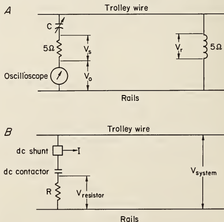
FIGURE A-1. - Testing high frequency characteristics.
