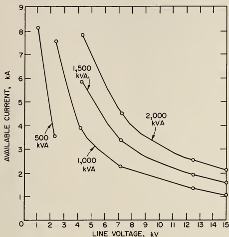
FIGURE 2. - Peak available current for various power ratings.
