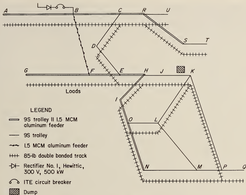
FIGURE 9. - Federal No. 1 haulage model.
