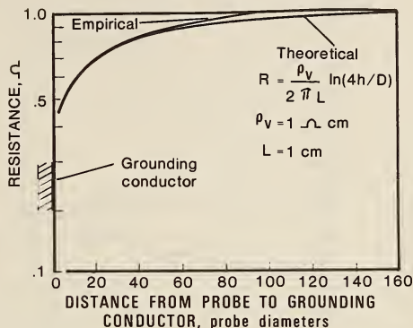
FIGURE 6. - Theoretical versus experimental resistances between probe and grounding conductor in a conductive medium.
