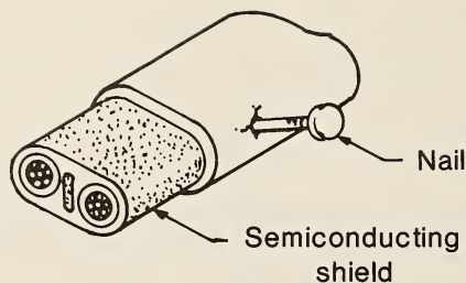
FIGURE 2. - Nail piercing cable and shorting semiconducting shield to power conductor.
