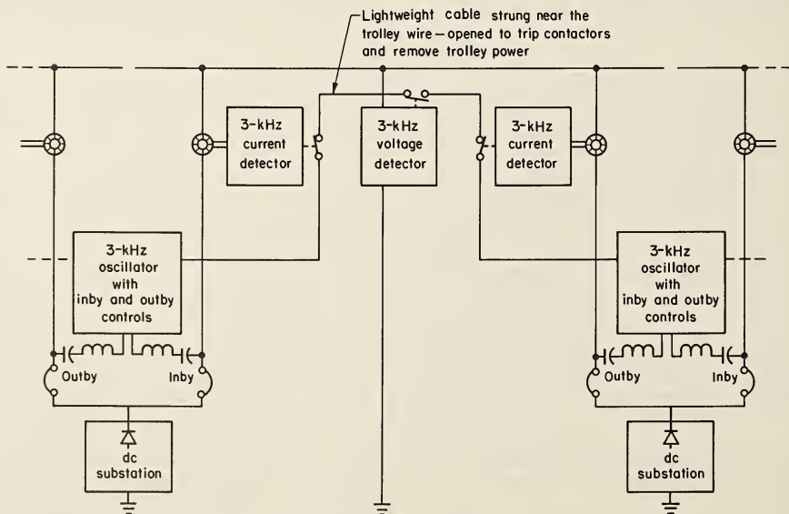
FIGURE 2. - Simplified DISCB system.
