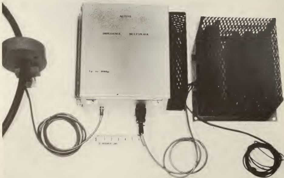
FIGURE 16. - Active impedance multiplier (AIM) with power supply.
