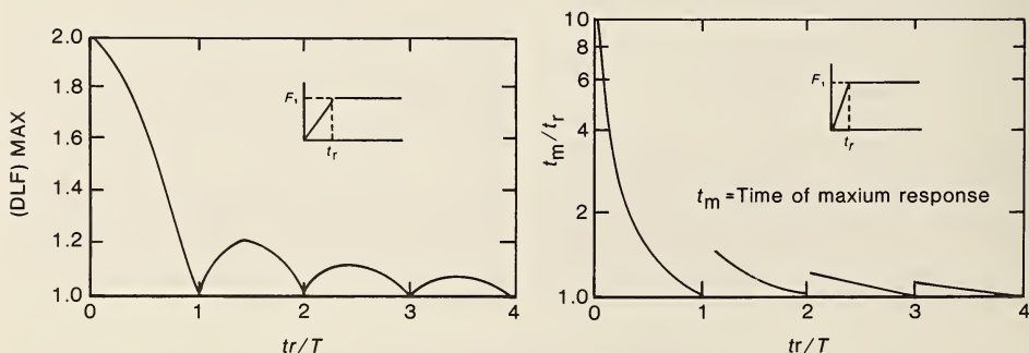
FIGURE 3. - Maximum response of 1-degree elastic systems (undamped) subjected to constant force with finite rise time (9).
