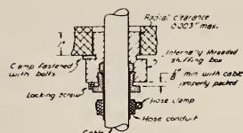
Figure 9. TYPICAL SLIP FIT STRAIGHT TYPE STUFFING BOX AND PACKING. LEAD ENTRANCE
