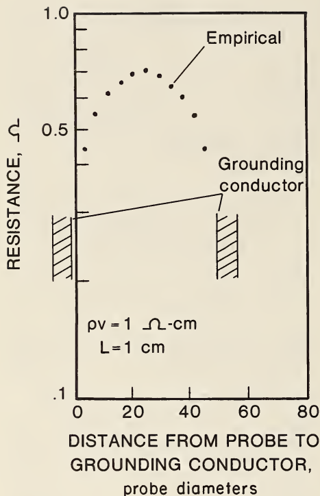
FIGURE 7. - Resistances with probe placed between two conductors.
