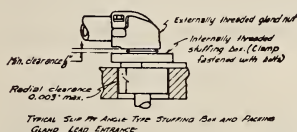
Figure 10. TYPICAL SLIP FIT ANGLE TYPE STUFFING BOX AND PACKING. LEAD ENTRANCE
