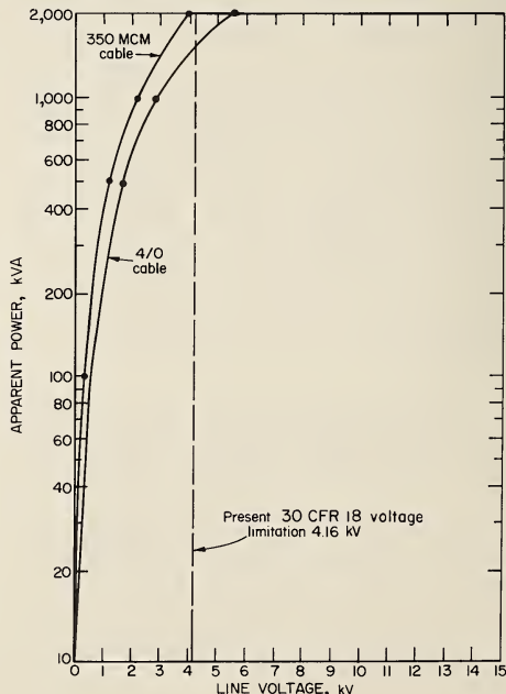
FIGURE 1. - Regions of practical interest, high-voltage permissible load centers.
