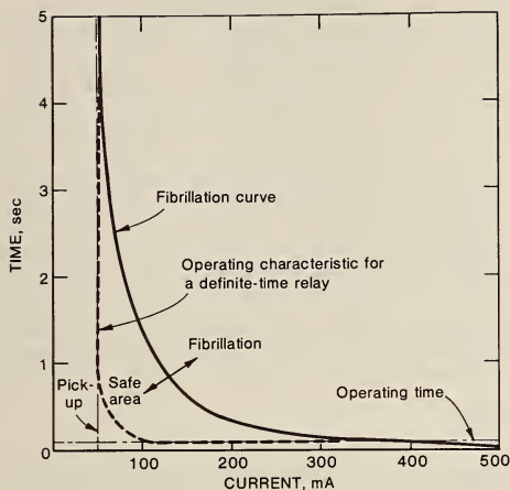
FIGURE 3. - Fibrillation curve.
