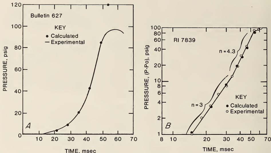
FIGURE 1. - Pressure in a 9-liter spherical chamber produced by ignition of a 9.6 vol-pct \text{CH}_4 -air mixture.
