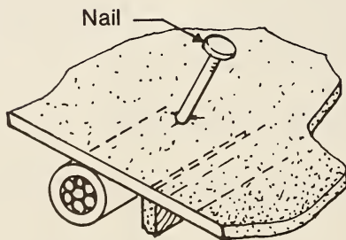
FIGURE 4. - Shielding further simplified for analysis of current between power and grounding conductors.
