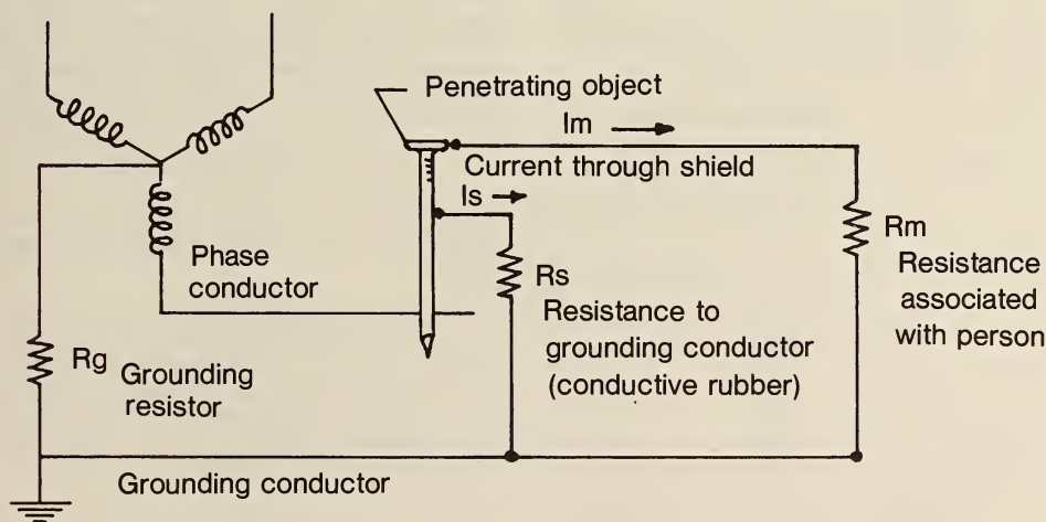
FIGURE 1. - Parallel current paths through person and shield for a simplified circuit.
