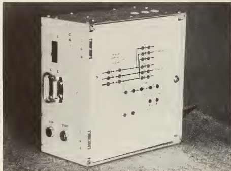
FIGURE 1. - Dead-front panel with outer lid of enclosure removed.
