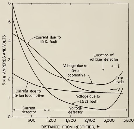
FIGURE 15. - DISCB protection.
