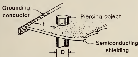
FIGURE 5. - Electrical path from piercing object to grounding conductor via the semiconducting shield material.
