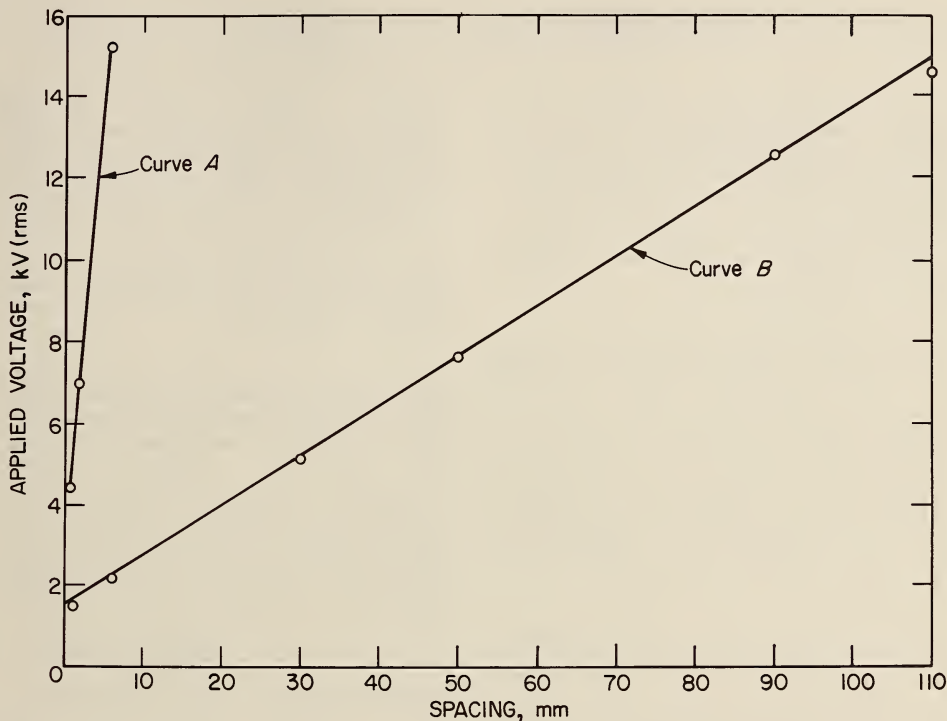
FIGURE 3. - Minimum arc of voltages versus air-gap spacings of electrodes. Curve A, in air; Curve B, in 9.8 pct methane-air mixtures.
