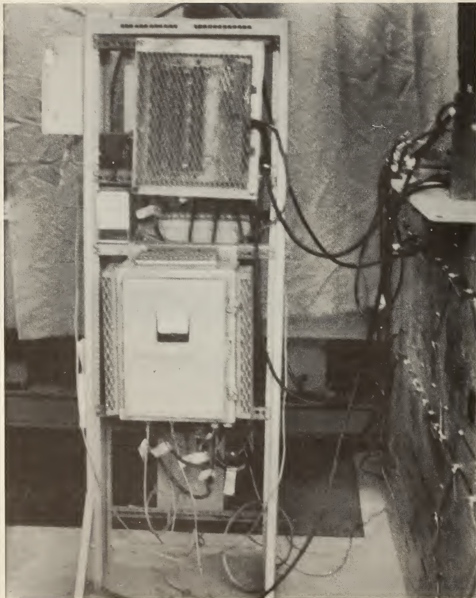
FIGURE 13. - DISCB controls at substation.
