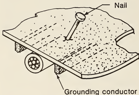
FIGURE 3. - Shielding material unwrapped from insulated conductor.
