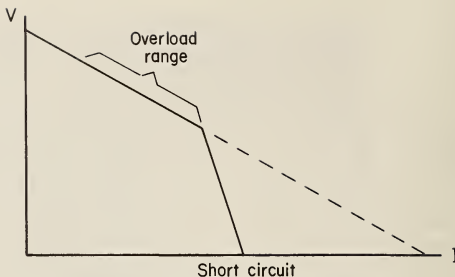
FIGURE 7. - Rectifier voltage regulation.
