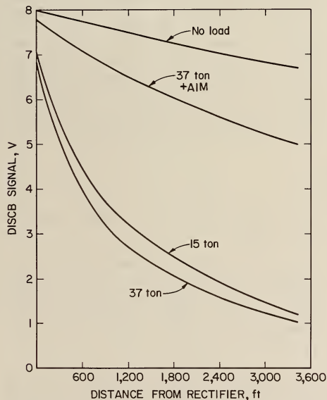
FIGURE 17. - Effects of active impedance multiplier (AIM).
