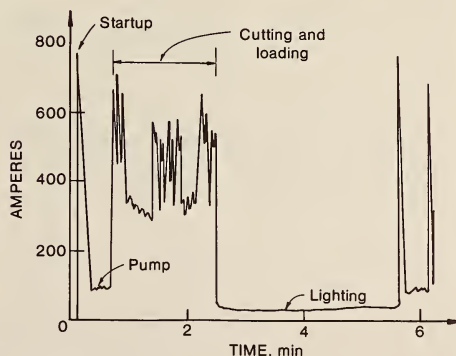
FIGURE 2. - Realistic current trace for continuous miner.
