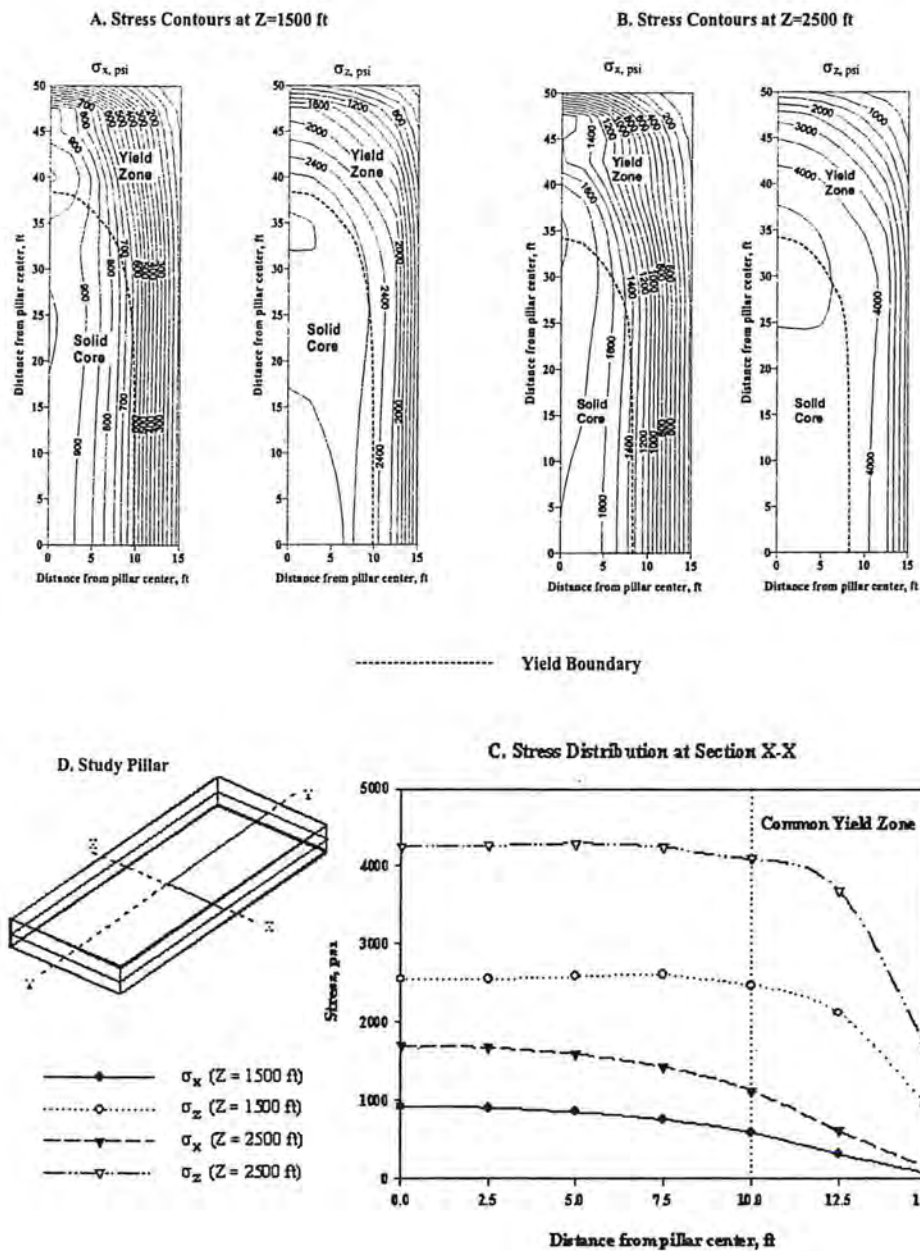
Figure 4-2 Stress distributions for linear Coulomb friction model
