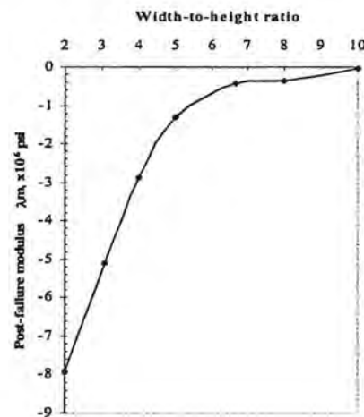
Figure 3-18 Estimated post-peak stiffness vs. the width-to-height ratio
