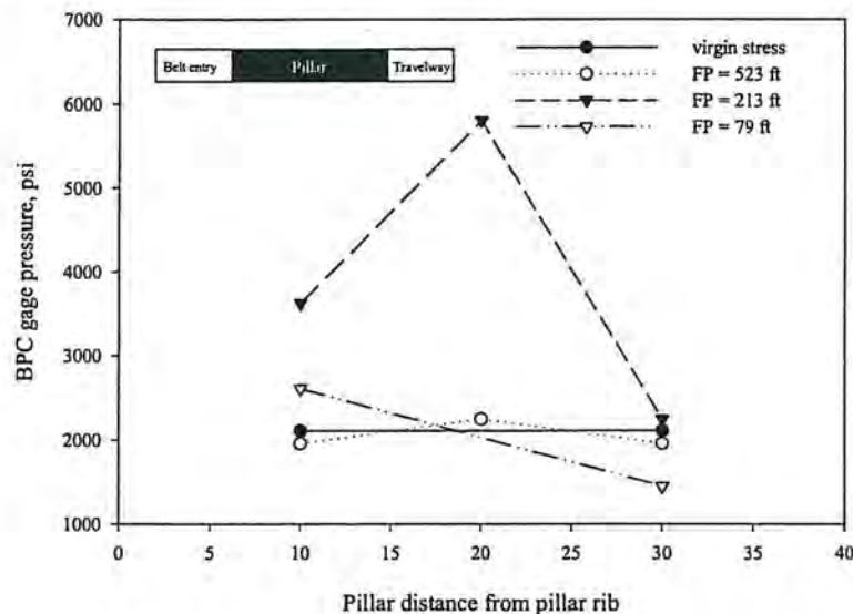
Figure 5-10 Ground pressure profiles for Site 2 [after Koehler, 1994]
