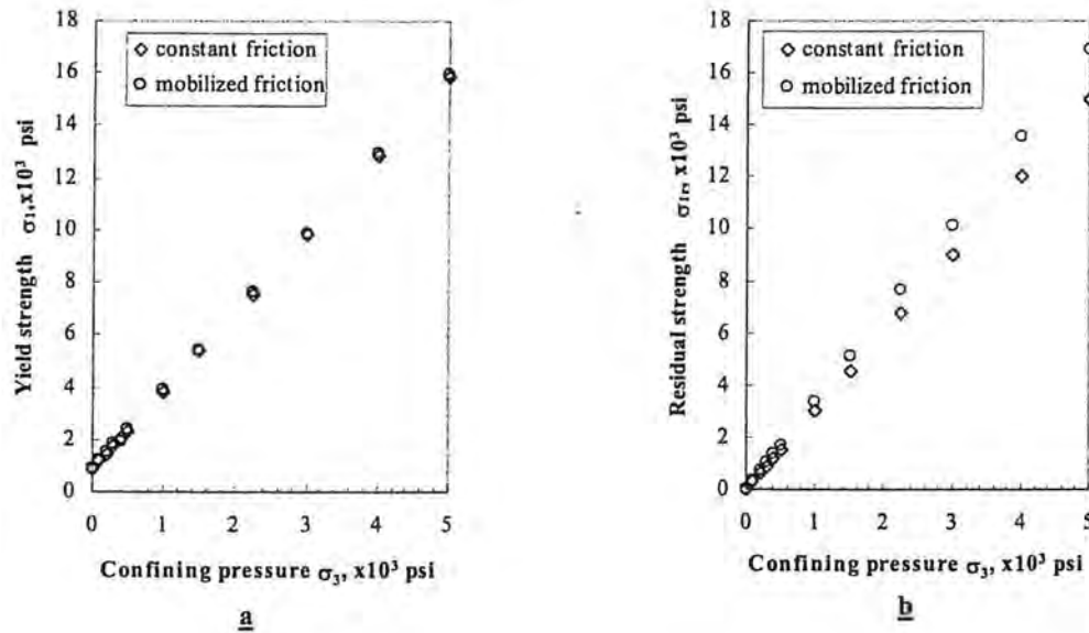
Figure 3-14 Estimated residual strength curves
