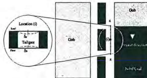
Figure 6-1 Roof-to-floor convergence locations
