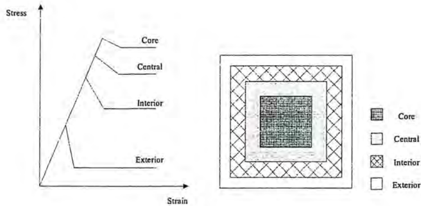
Figure 5-2 Heasley's coal pillar model [after, Heasley 1992]
