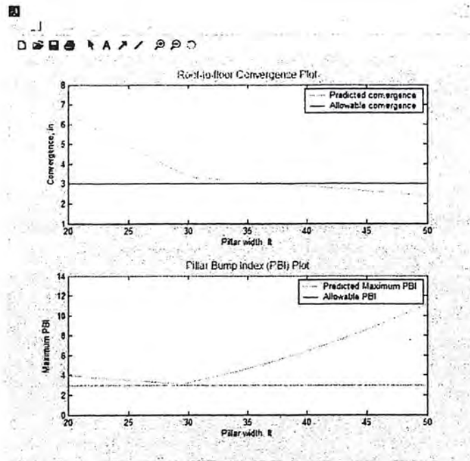
Figure C- 3 Design plots
