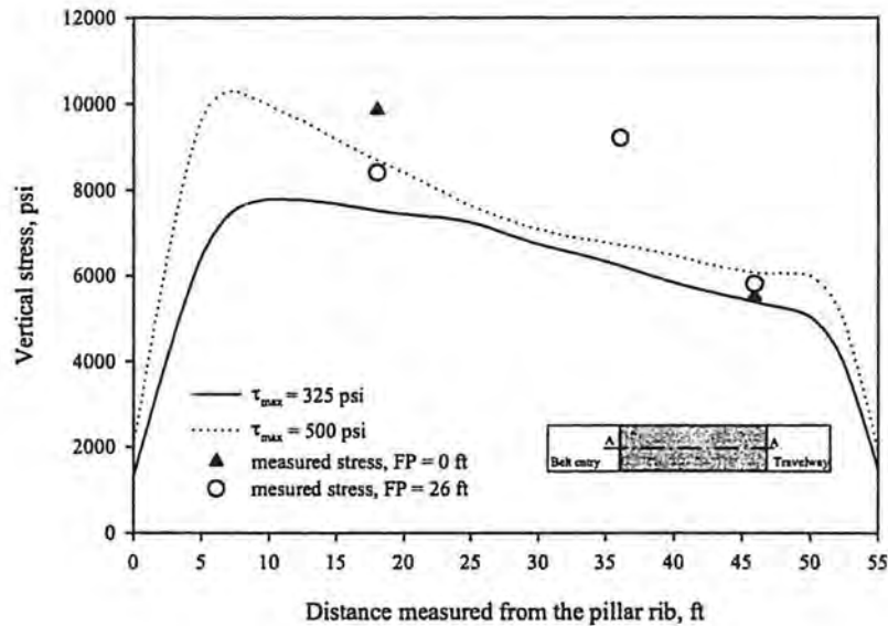
Figure 5-14 Pillar vertical stress distribution at Site 1
