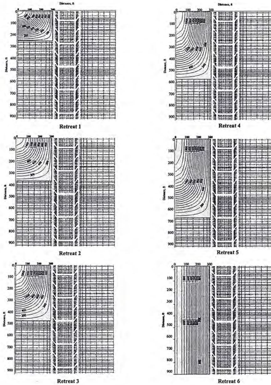
Figure 3-31 Vertical stress contours in gob area of panel S-9, (stresses are in psi)
