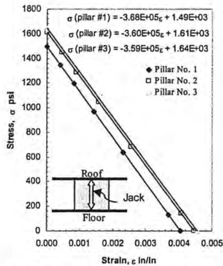
Figure 3-39 Stress-strain relations at the pillar center
