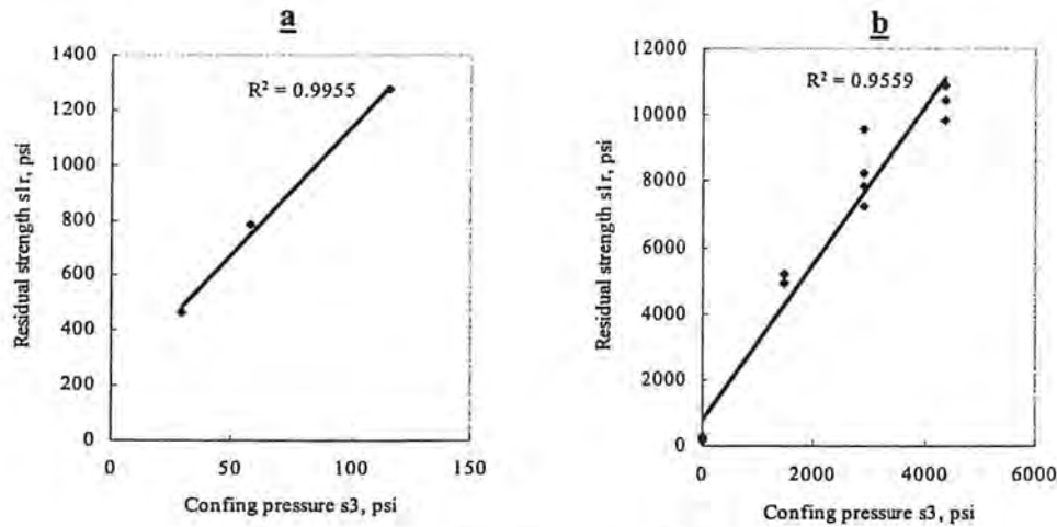
Figure 3-6 Coal residual strength vs. confining pressure
