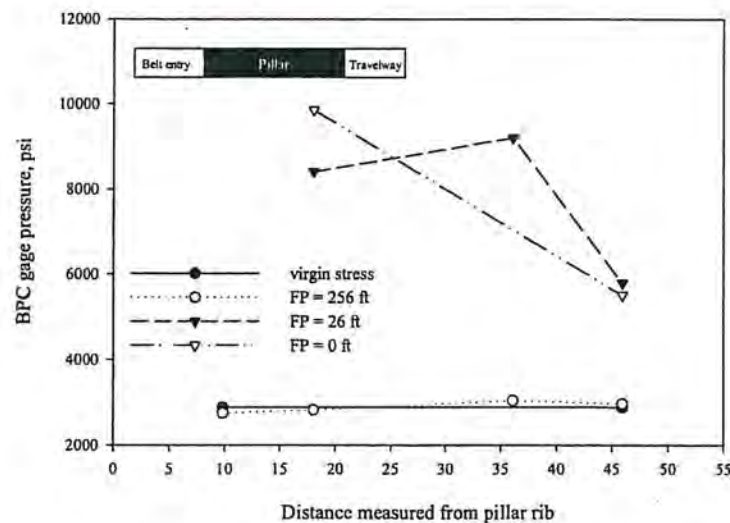
Figure 5-8 Ground pressure profiles for Site 1 [Koehler, 1994]
