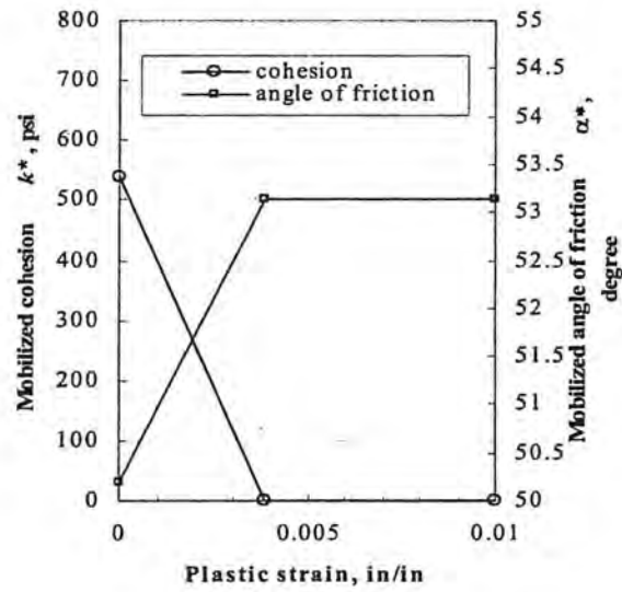
Figure 3-11 Strain softening parameters used for the simulations
