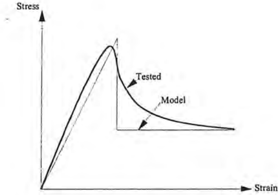
Figure 2-13 Stress-strain curve for coal, [Chen, 1988]
