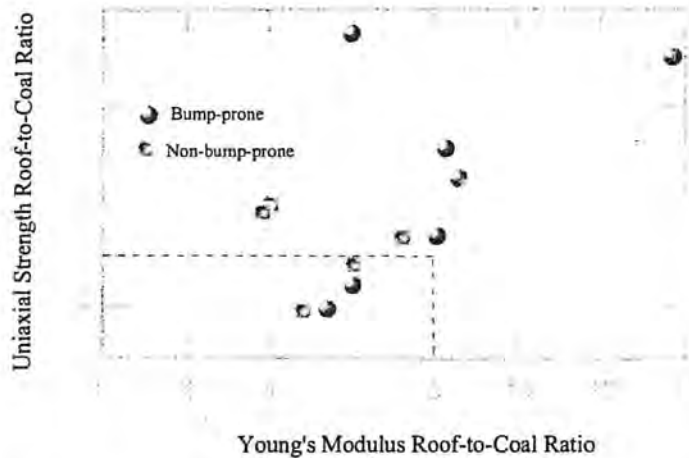
Figure 2-8 Strength ratio versus Young's modulus for roof and coal [after Malaki, 1995]
