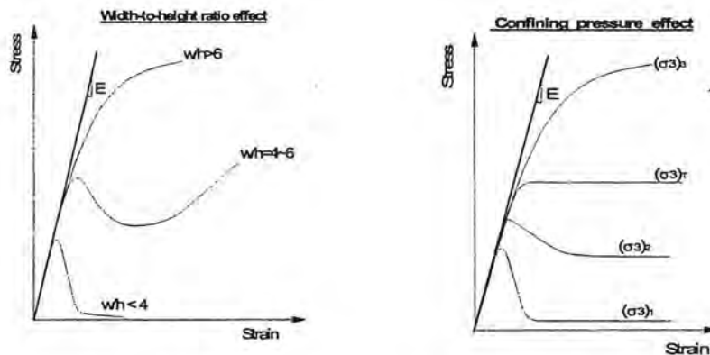
Figure 3-4 Conceptual stress-strain curves for coal material
