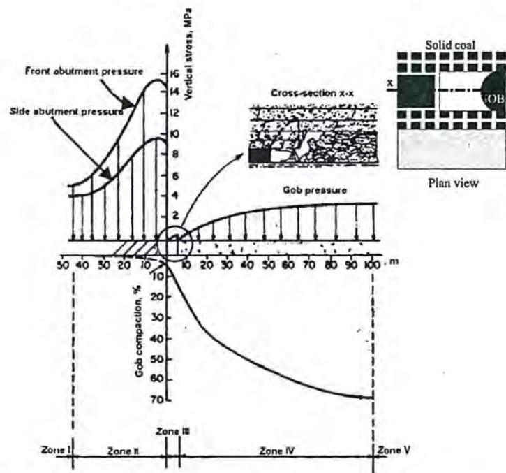
Figure 3-21 Distribution of strata pressure in the vicinity of the longwall face, (modified from Unrug et. al., 1982)
