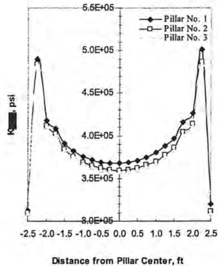
Figure 3-40 Distribution of K_{LMS} Pillars No. 1 to 3
