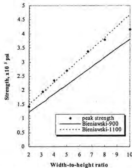
Figure 3-19 Estimated peak strength vs. width-to-height ratio
