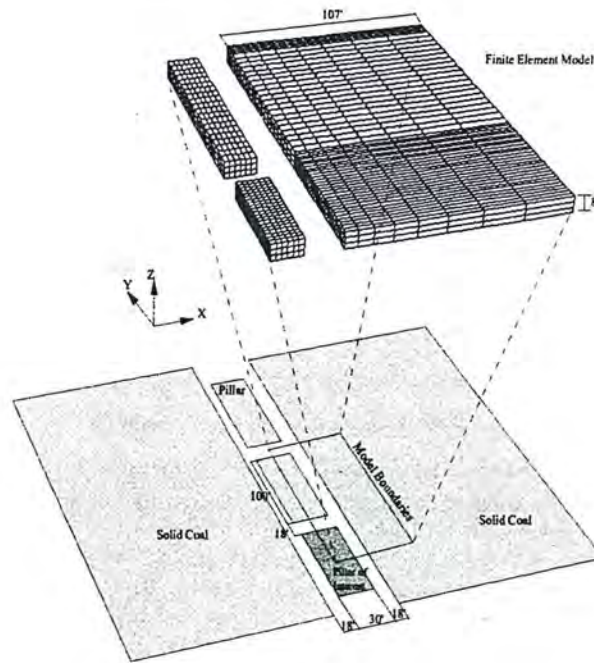
Figure 4-1 Finite Element Model Configurations
