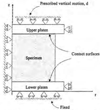
Figure 3-15 Uniaxial compression test with regular platens
