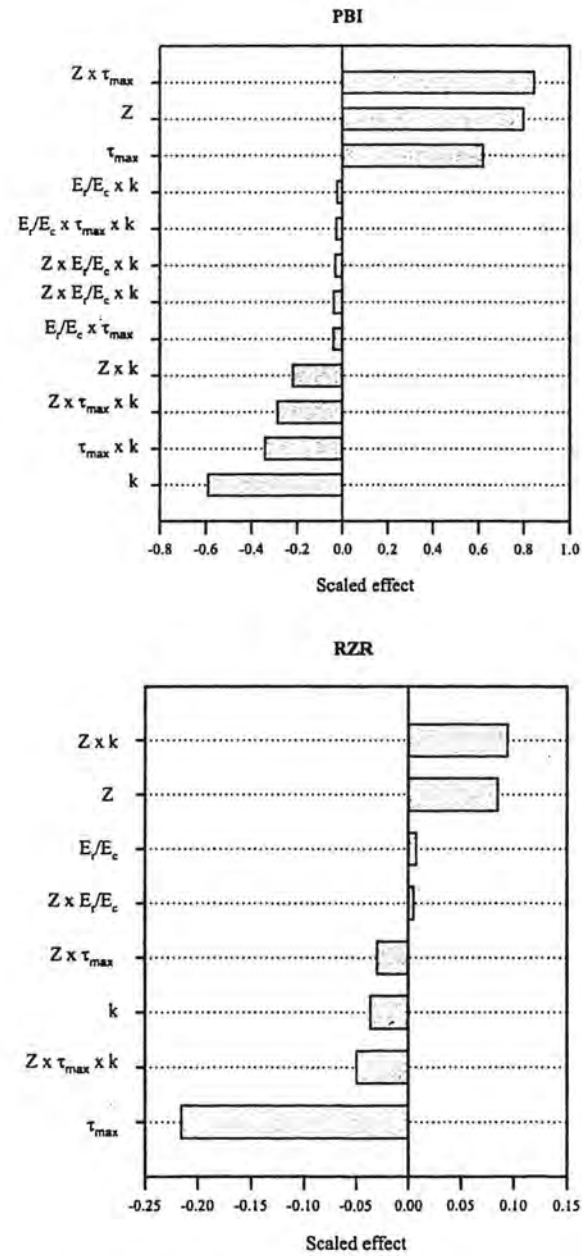
Figure 6-3 Scaled effect of geological and geometrical factors on PBI and RZR
