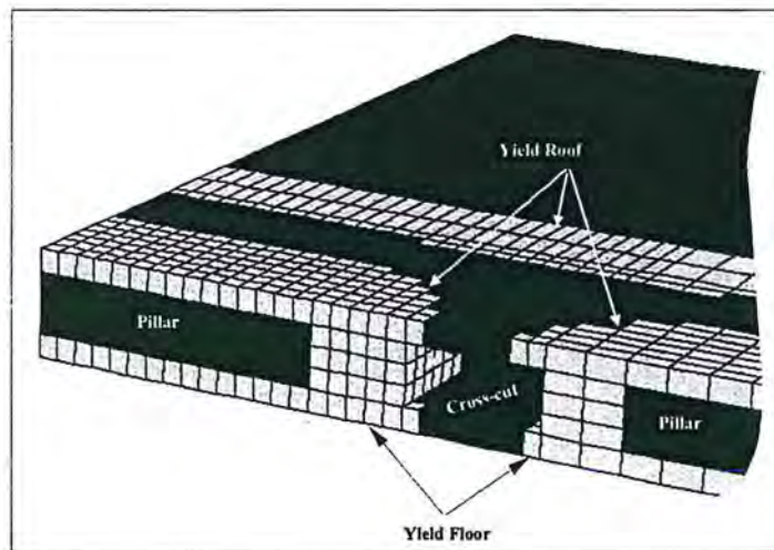
Figure 4-4 Locations of yield zones for YRF condition
