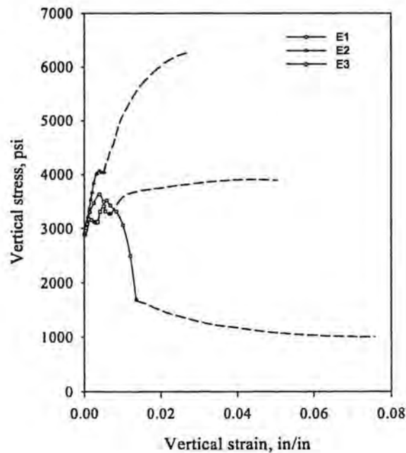
Figure 5-21 Stress-strain curves at different pillar zones, Site 1
