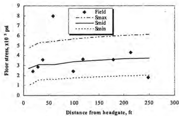
Figure 3-33 Vertical stress profiles under panel S-9
