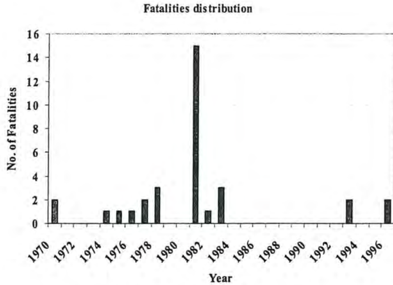
Figure 2-2 Coal bumps fatalities distribution
