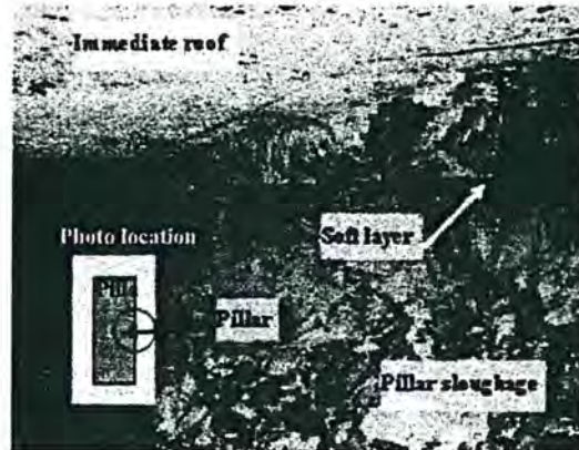
Figure 6-9 Rib sloughing
