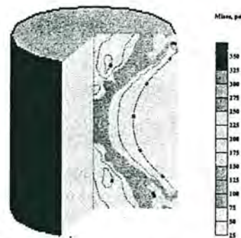
Figure 3-16 Specimen shear failure
