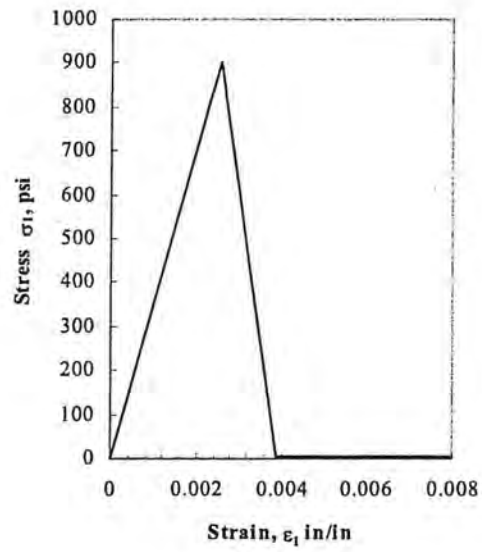
Figure 3-10 Rectilinear stress-strain curve for coal model
