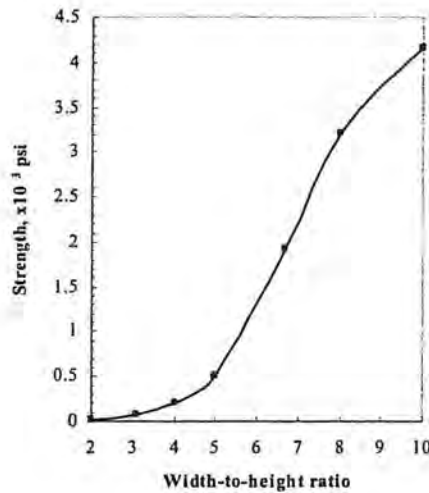
Figure 3-20 Estimated residual strength vs. width-to-height ratio
