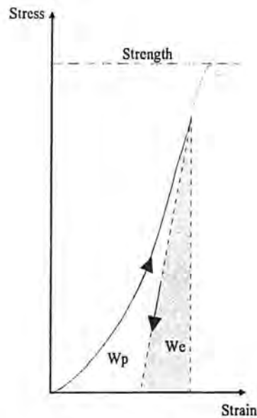
Figure 2-5 Determination of the strain energy storage index
