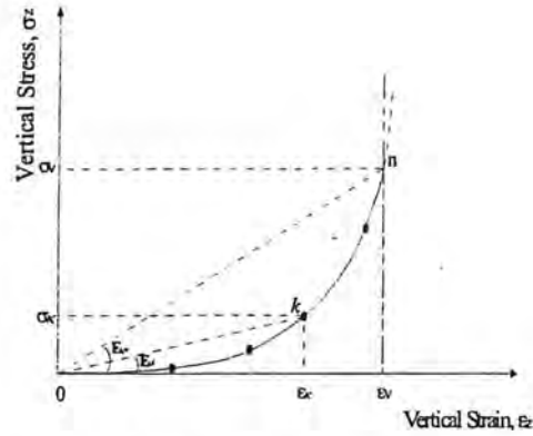
Figure 3-22 Stress-strain relationship for Terzaghi's model
