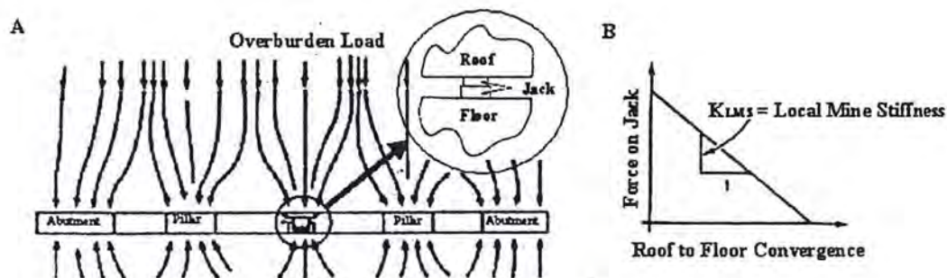
Figure 3-37 Illustration of Local Mine Stiffness Concept
