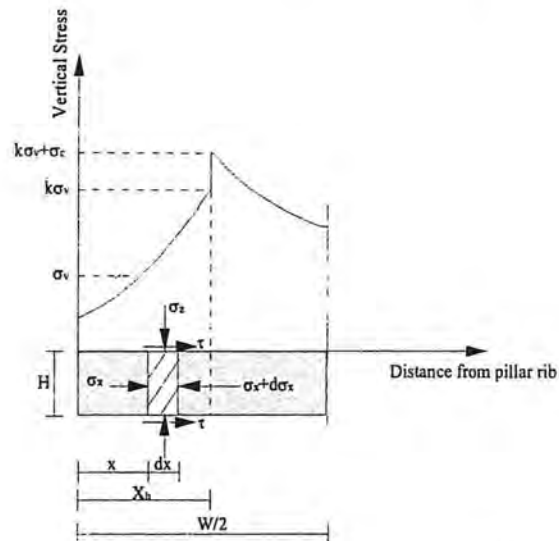
Figure 2-12 Forces acting on an element strip in wide pillar
