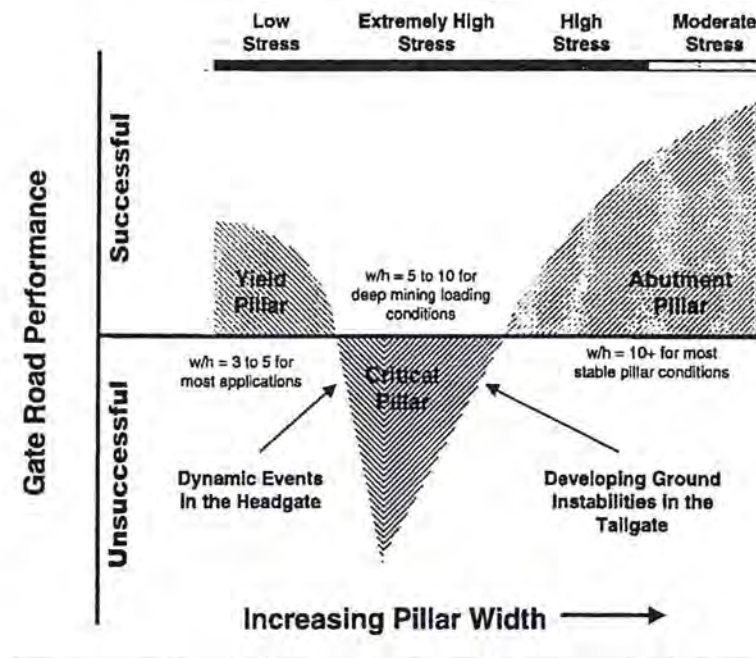
Figure 2-4 Conceptual diagram of the critical pillar [DeMarco, 1996]
