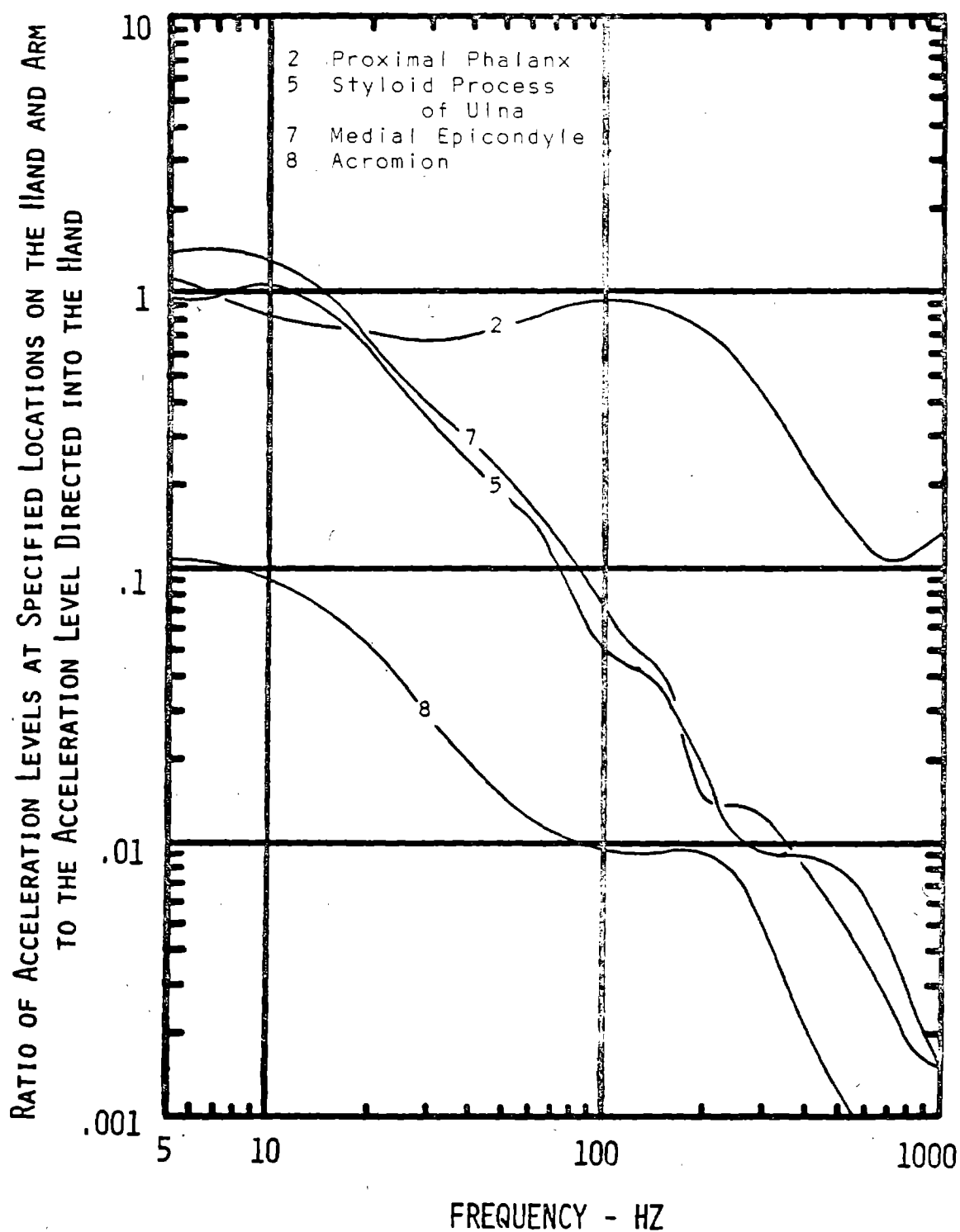
Figure 18 Average Value Transmissibility Curves for Vibration in the Horizontal Direction - 2 lb f Finger Grip
