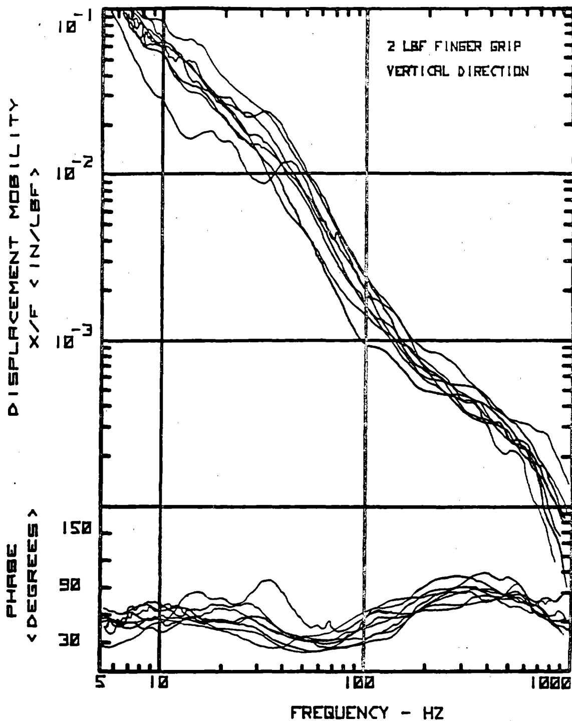
Figure 5 Typical Displacement Mobility Data Set for Eight Test Subjects
