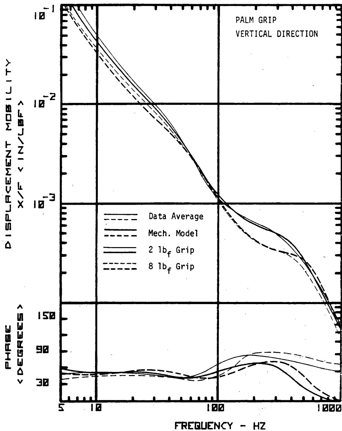
Figure 13 Comparison of the Displacement Mobility Response of the Hand and the Response Predicted by the Mechanical Model for the 2 lbf and 8 lbf Palm Grip - Vertical Direction
