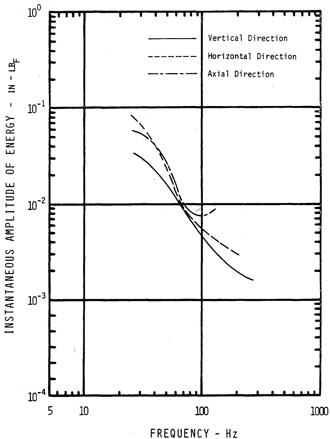
Figure 43 Amplitudes of the Instantaneous Stored Potential and Kinetic Energies for Vibration in the Vertical, Horizontal and Axial Directions - 2 lb f Finger Grip
