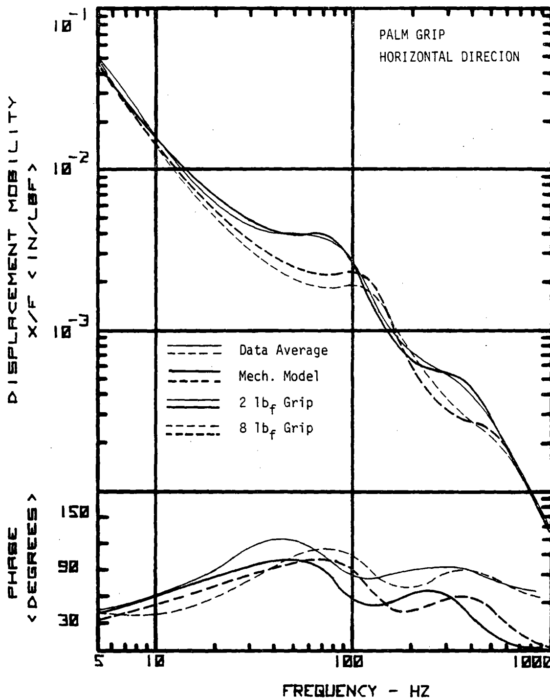
Figure 14 Comparison of the Displacement Mobility Response of the Hand and the Response Predicted by the Mechanical Model for the 2 lb f and 8 lb f Palm Grip - Horizontal Direction
