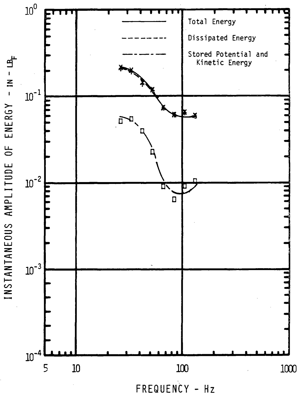
Figure 42 Make-Up of Instantaneous Energy Directed into the Hand for Vibration in the Axial Direction - 2 lb f Finger Grip
