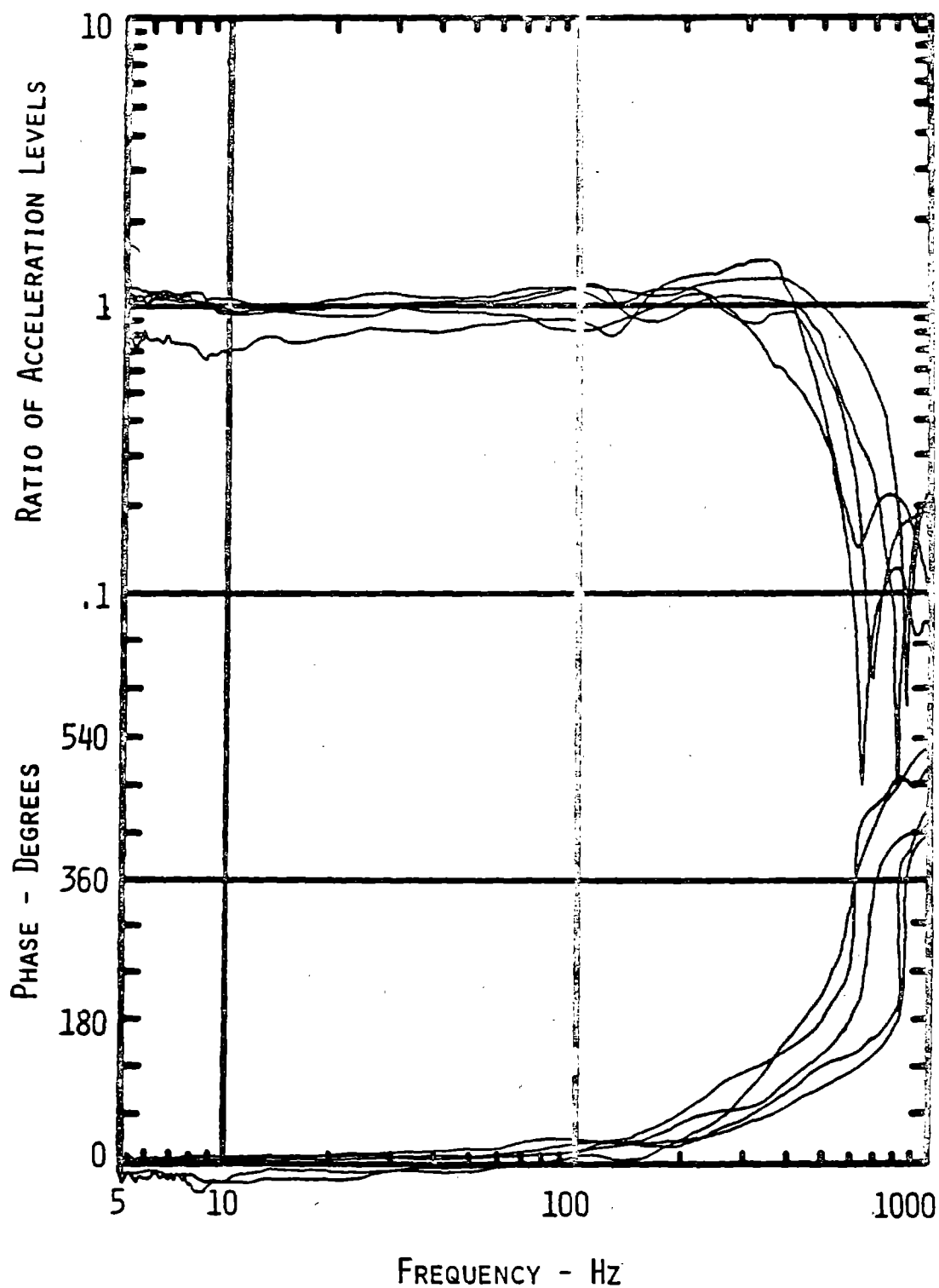
Figure 22 Ratio of Vibration Levels at Middle Phalanx (location 1) Divided by Vibration Levels Induced into the Hand with Phase Difference between Corresponding Signals for Individual Test Subjects - 2 lb f Finger Grip, Vertical Direction
