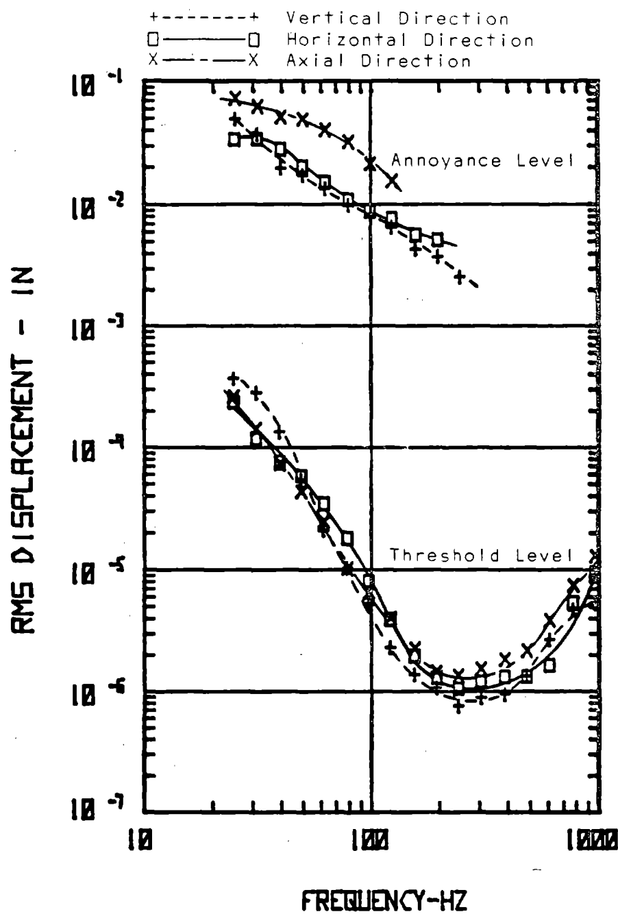
Figure 37 Discrete Frequency Threshold and Annoyance Level Curves for Vibration in the Vertical, Horizontal and Axial Directions - 8 lb f Finger Grip
