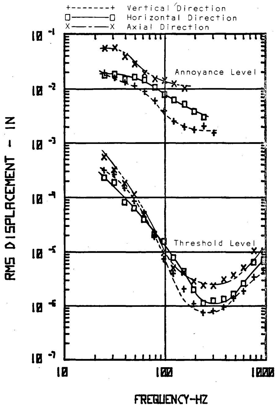
Figure 39 Discrete Frequency Threshold and Annoyance Level Curves for Vibration in the Vertical, Horizontal and Axial Directions - 8 lb f Palm Grip
