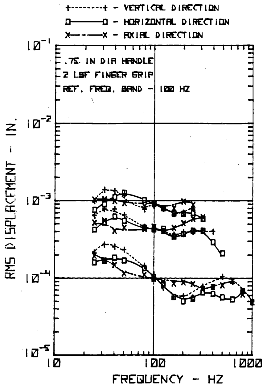
Figure 35 1/3 Octave Broad Band Equal Sensation Curves for Vibration in the Vertical, Horizontal and Axial Directions - 2 lb f Finger Grip
