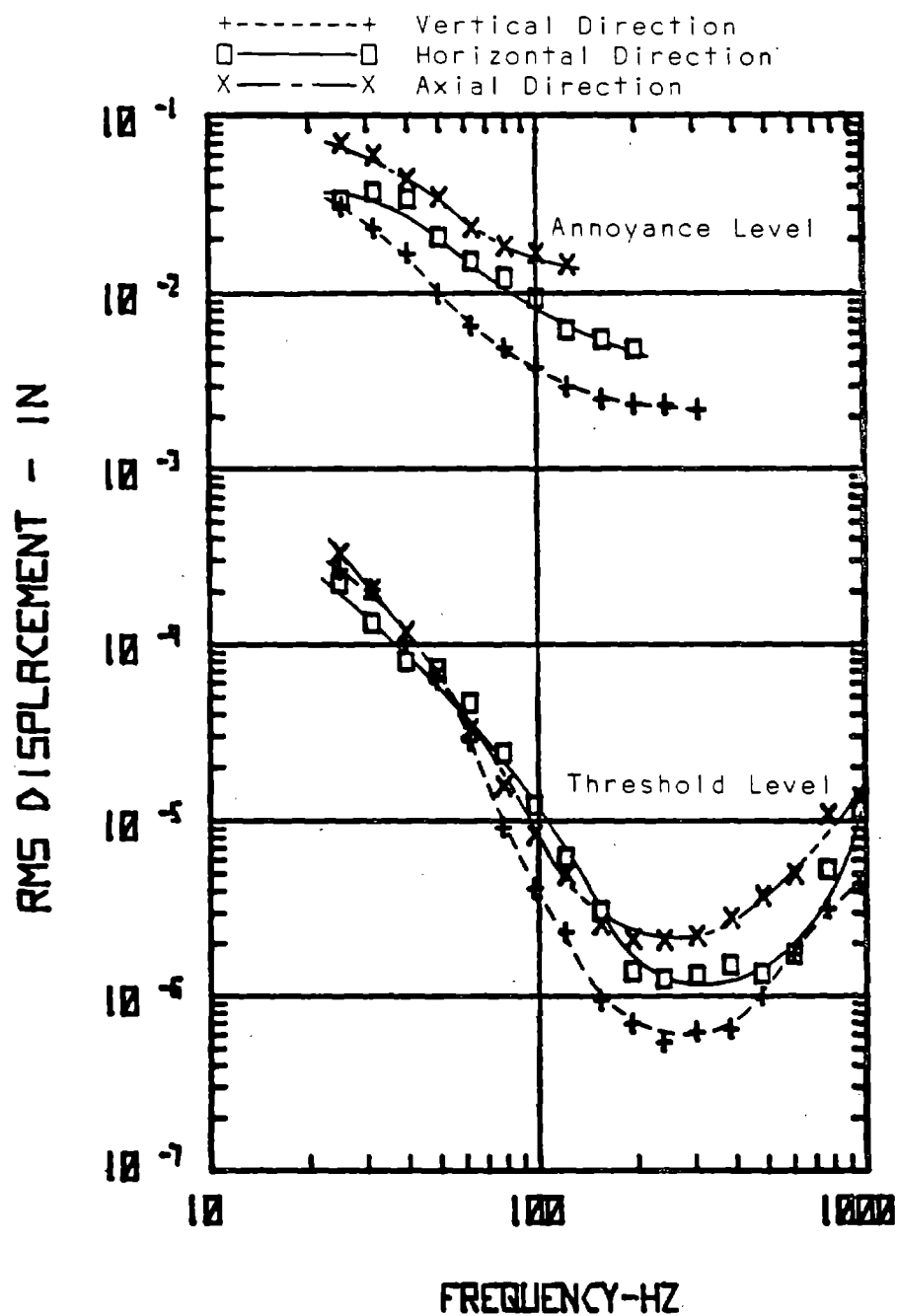
Figure 36 Discrete Frequency Threshold and Annoyance Level Curves for Vibration in the Vertical, Horizontal and Axial Directions - 2 lb f Finger Grip
