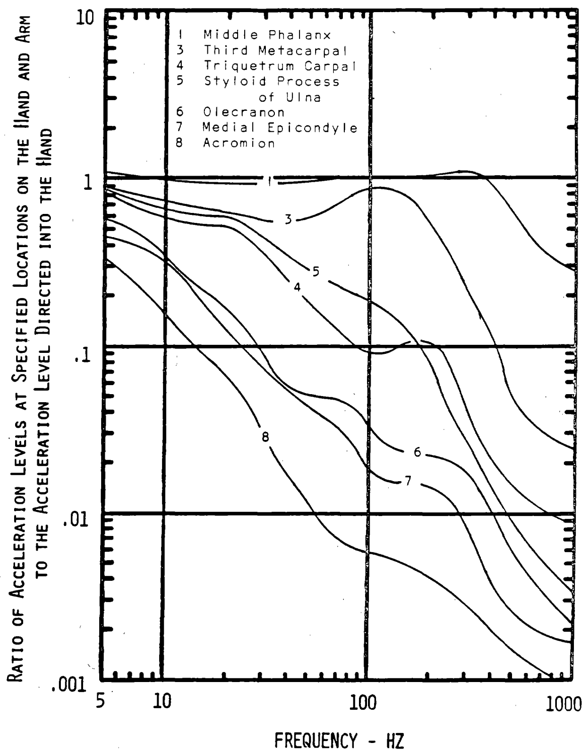
Figure 17 Average Value Transmissibility Curves for Vibration in the Vertical Direction - 2 lb f Finger Grip
