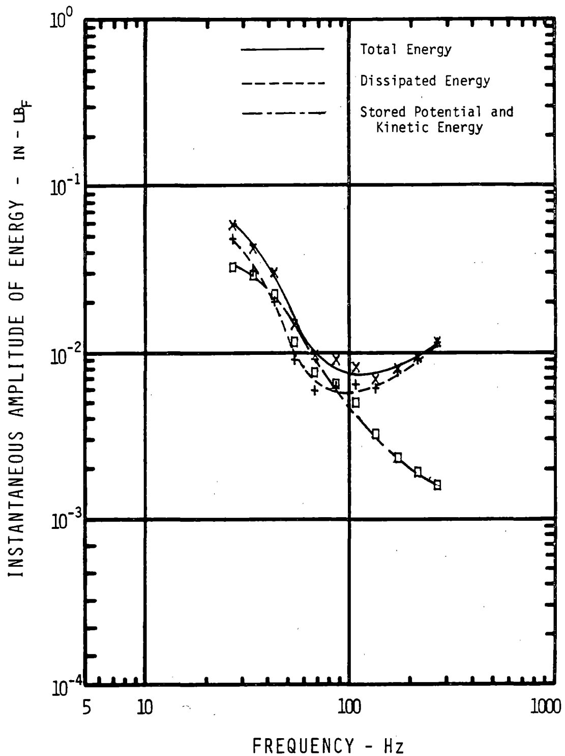
Figure 40 Make-Up of Instantaneous Energy Directed into the Hand for Vibration in the Vertical Direction - 2 lb f Finger Grip
