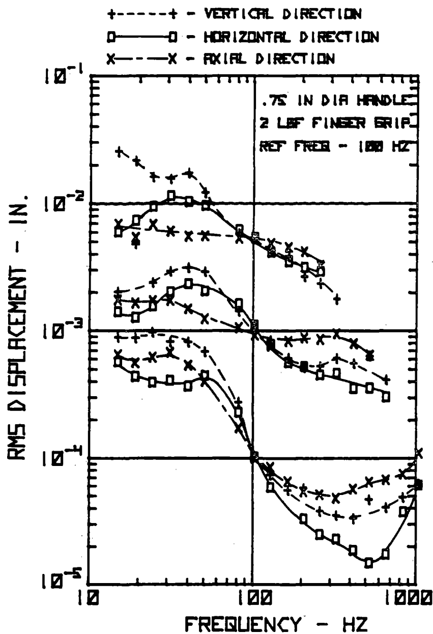
Figure 34 Discrete Frequency Equal Sensation Curves for Vibration in the Vertical, Horizontal and Axial Directions - 2 lb f Finger Grip
