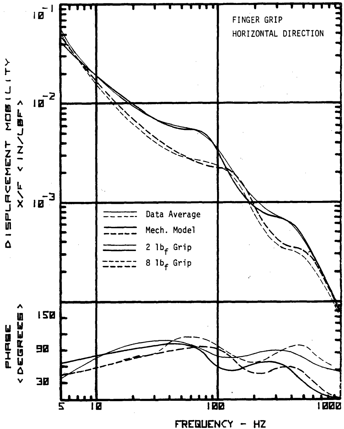
Figure 11 Comparison of the Displacement Mobility Response of the Hand and the Response Predicted by the Mechanical Model for the 2 lb f and 8 lb f Finger Grip - Horizontal Direction
