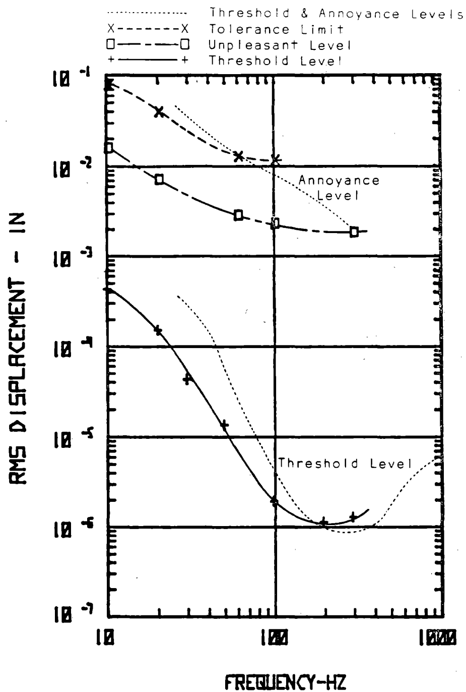
Figure 44 Comparison of 2 lb f Palm Grip Threshold and Annoyance Level Curves with the Threshold, Unpleasant and Tolerance Limit Curves Obtained from the Data of Miwa
