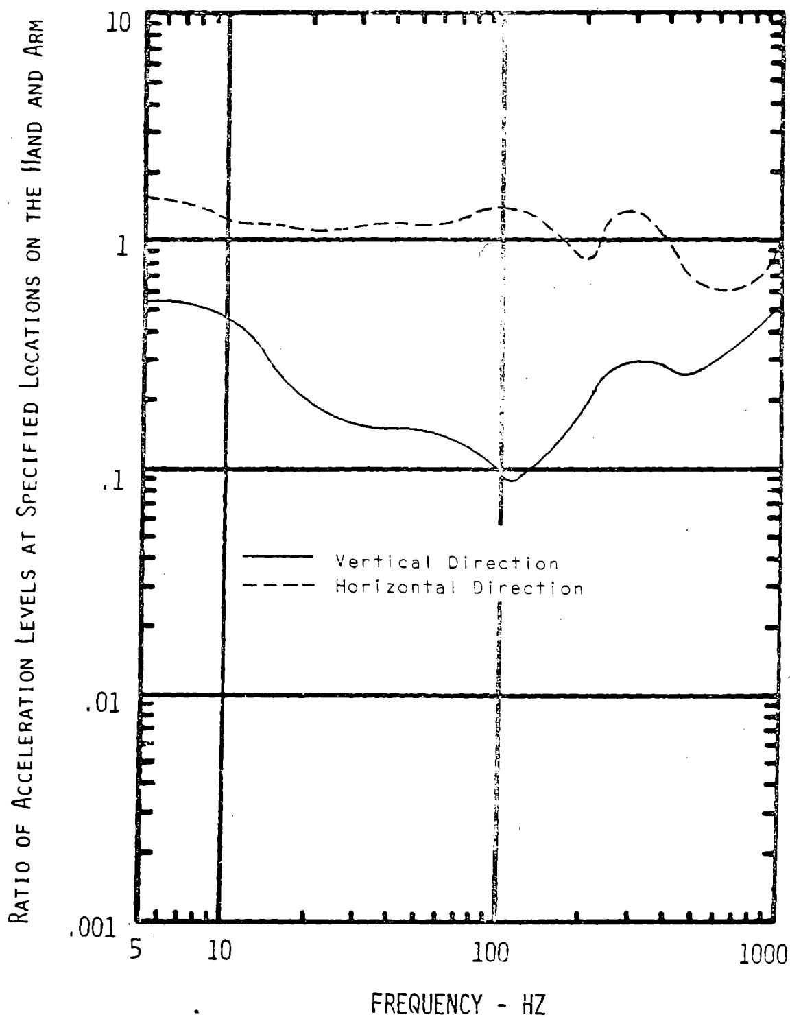
Figure 21 Calculated Ratios of the Vibration Levels at the Elbow Divided by the Vibration Levels at the Wrist for Vibration in the Horizontal and Vertical Directions - 2 lb f Finger Grip
