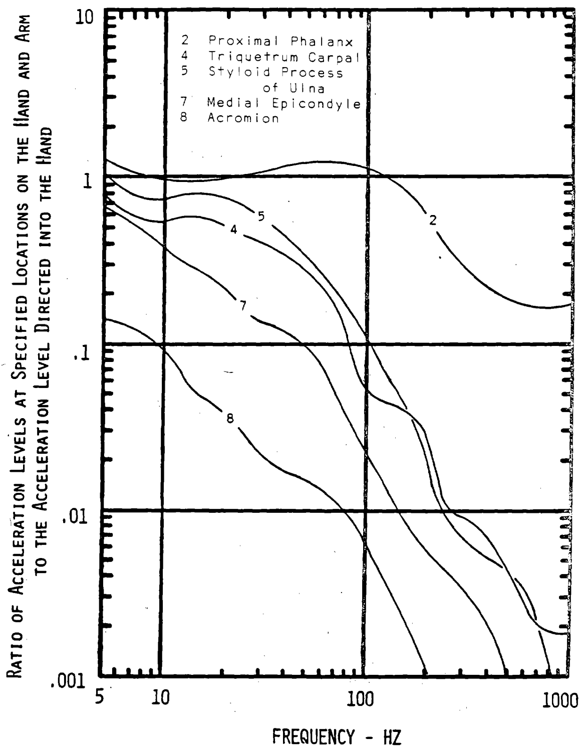
Figure 19 Average Value Transmissibility Curves for Vibration in the Axial Direction - Axial Direction
