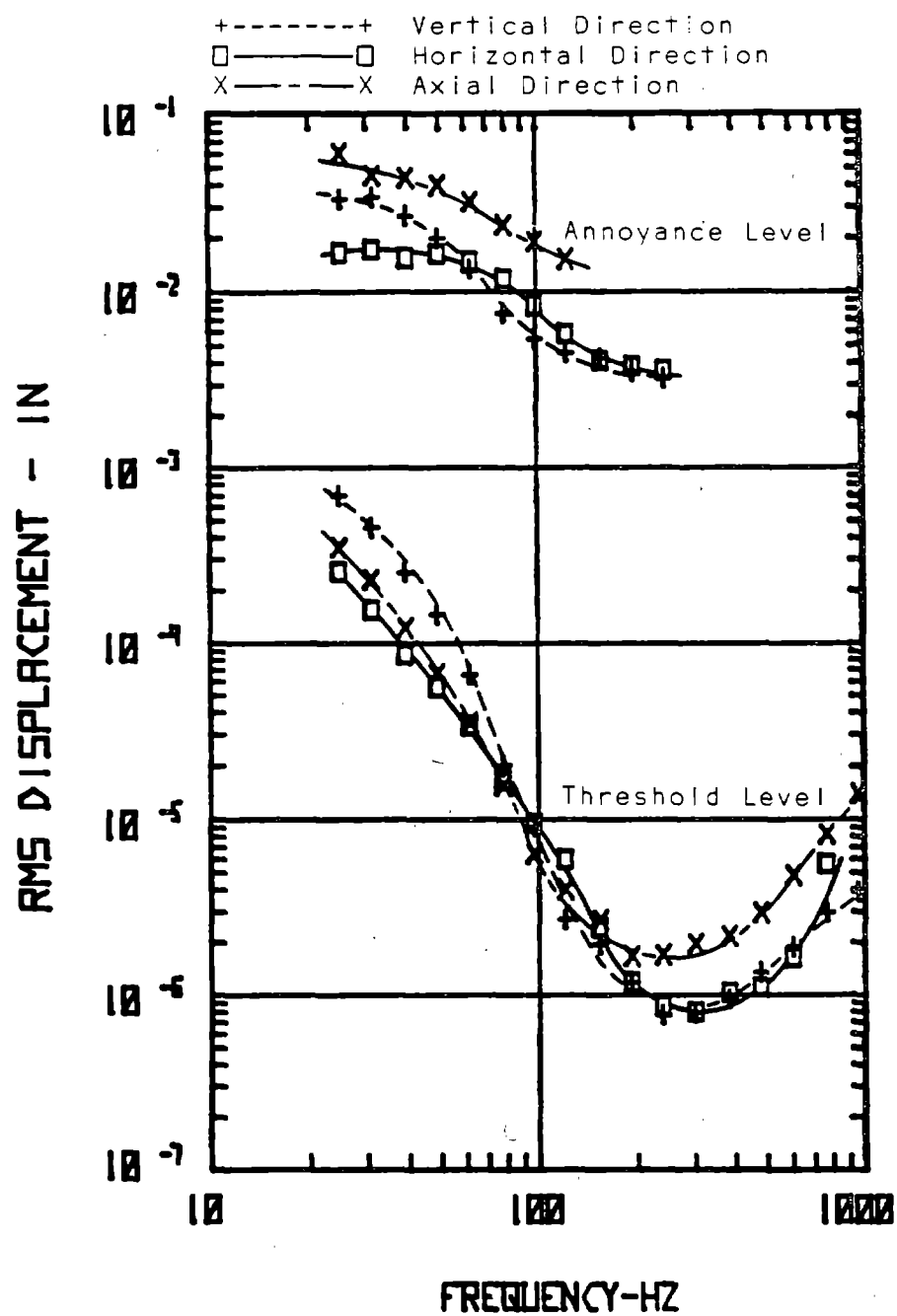
Figure 38 Discrete Frequency Threshold and Annoyance Level Curves for Vibration in the Vertical, Horizontal and Axial Directions - 2 lb f Palm Grip
