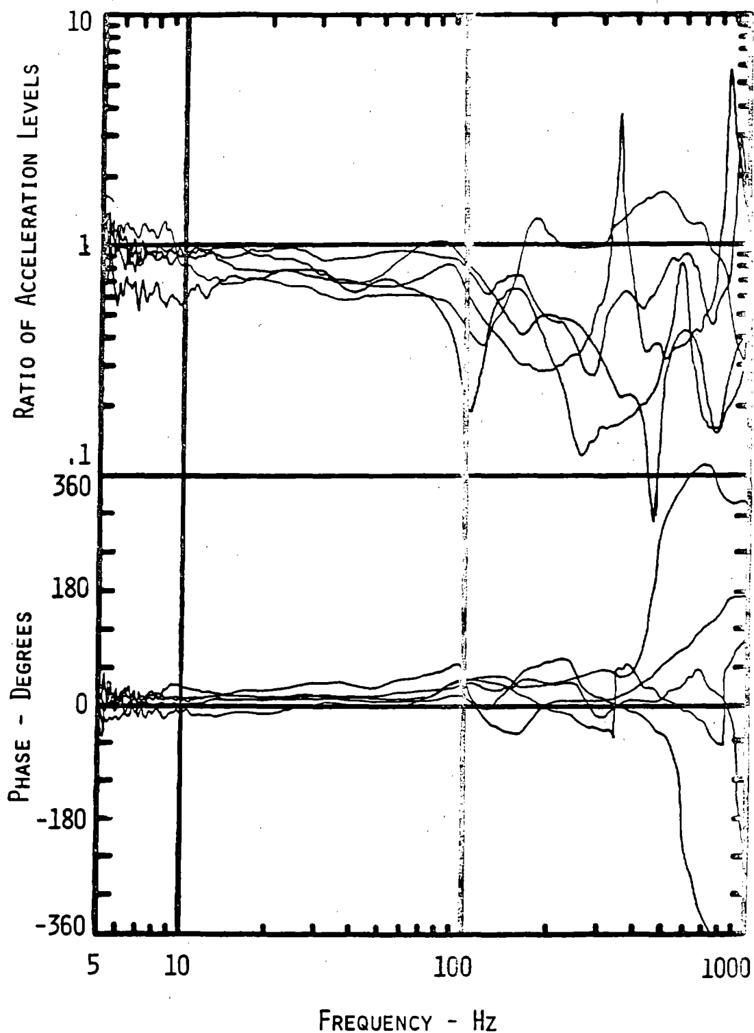
Figure 25 Ratio of Vibration Levels at Third Metacarpal (location 3) Divided by Vibration Levels at Proximal Phalanx (location 2) with Phase Difference between Corresponding Signals for Individual Test Subjects - 2 lb f Finger Grip, Vertical Direction
