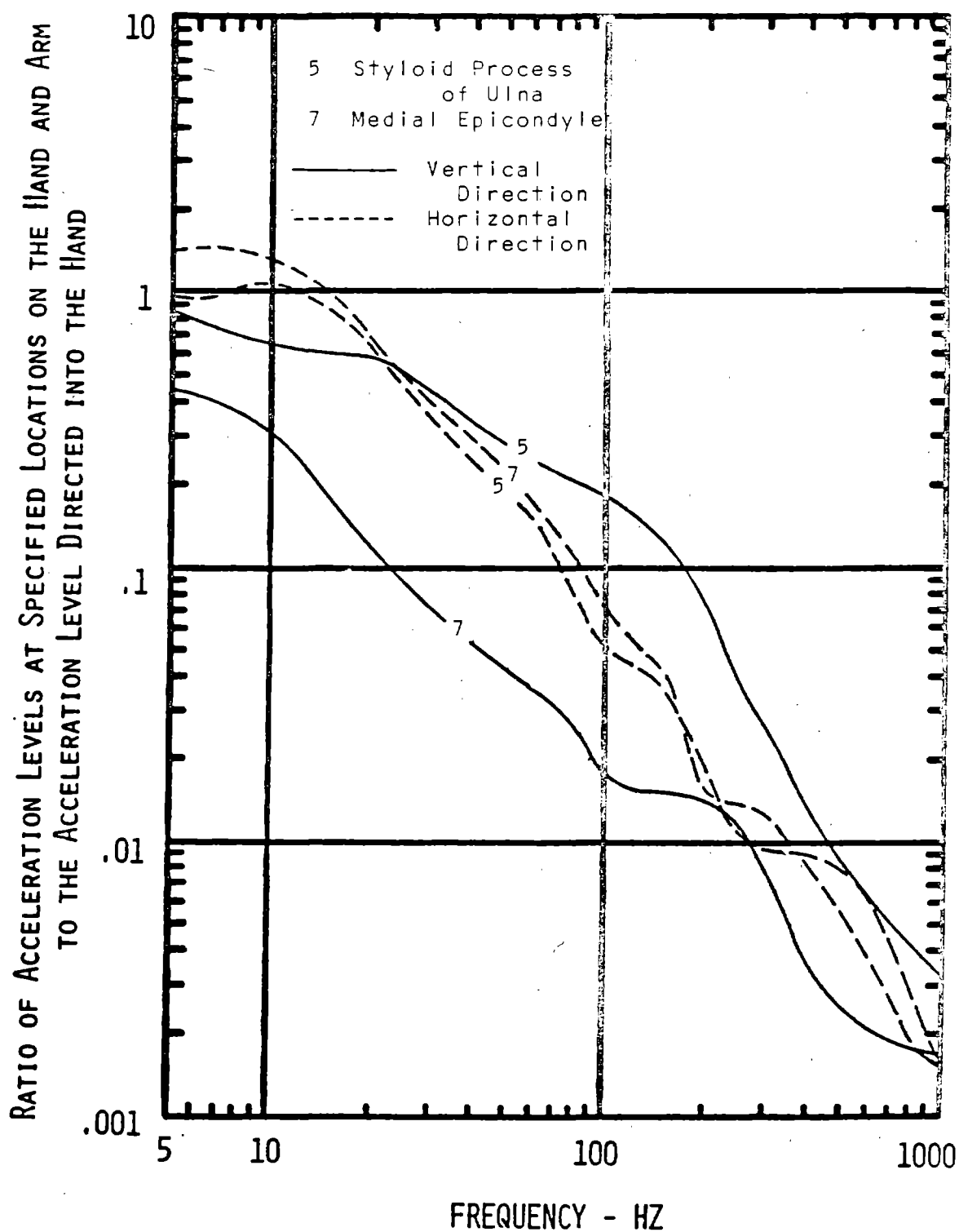
Figure 20 Comparison of the Average Value Transmissibility Curves for the Elbow and Wrist Joints for Vibration in the Horizontal and Vertical Directions - 2 lb f Finger Grip
