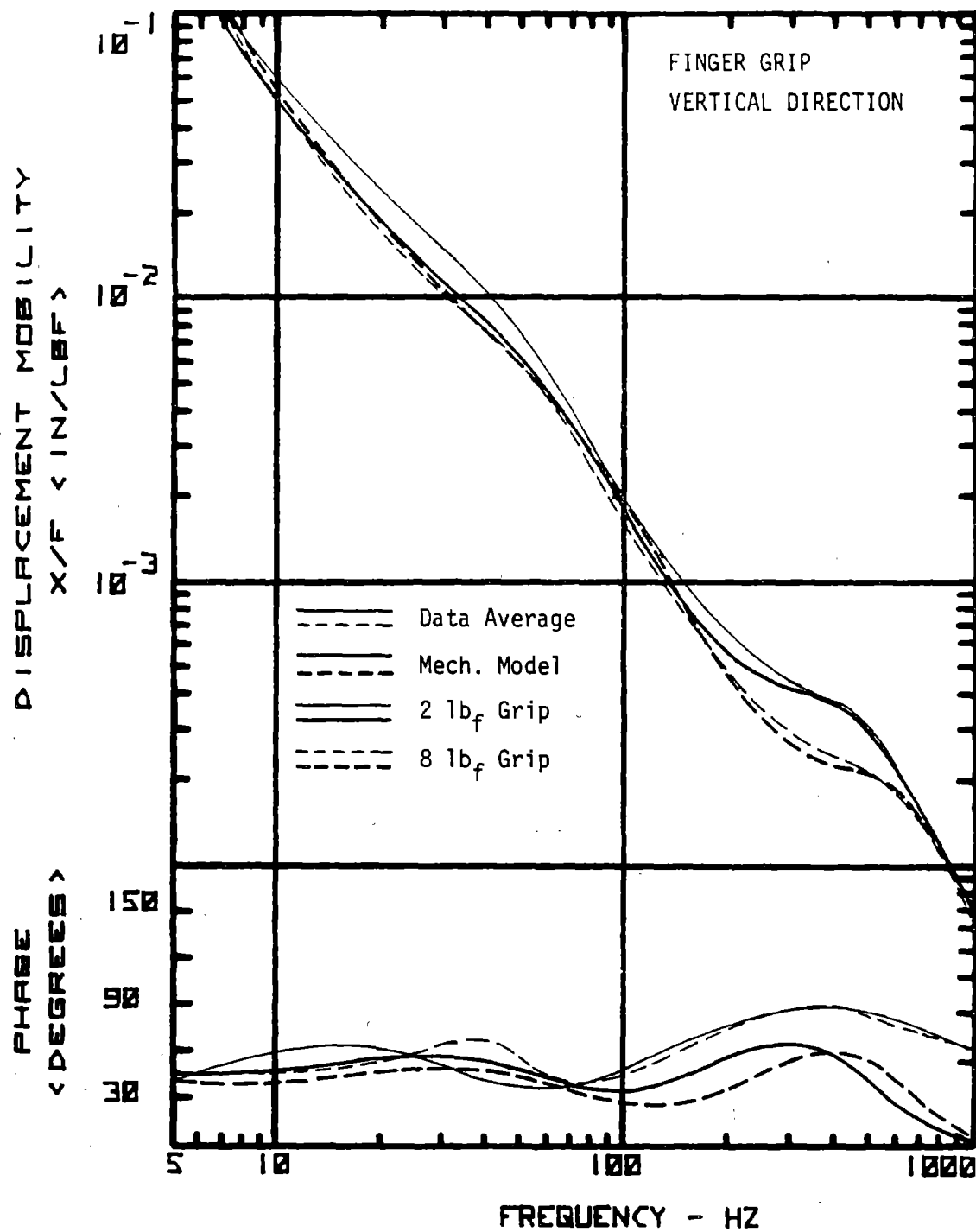
Figure 10 Comparison of the Displacement Mobility Response of the Hand and the Response Predicted by the Mechanical Model for the 2 lb f and 8 lb f Finger Grip - Vertical Direction
