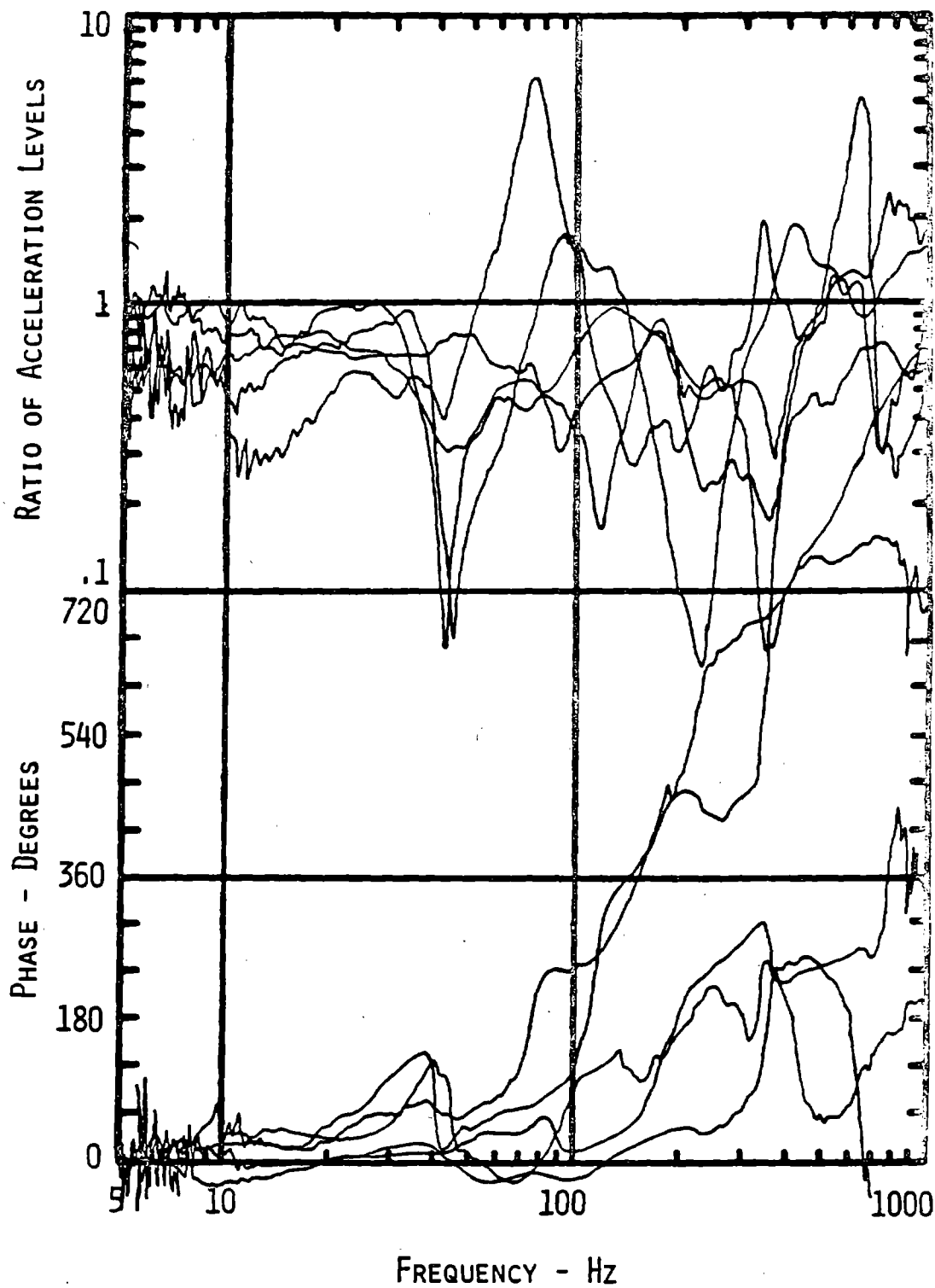
Figure 26 Ratio of Vibration Levels at Styloid Process of Ulna (location 5) Divided by Vibration Levels at Triquetrum Carpal (location 4) with Phase Difference between Corresponding Signals for Individual Test Subjects - 2 lb f Finger Grip, Vertical Direction
