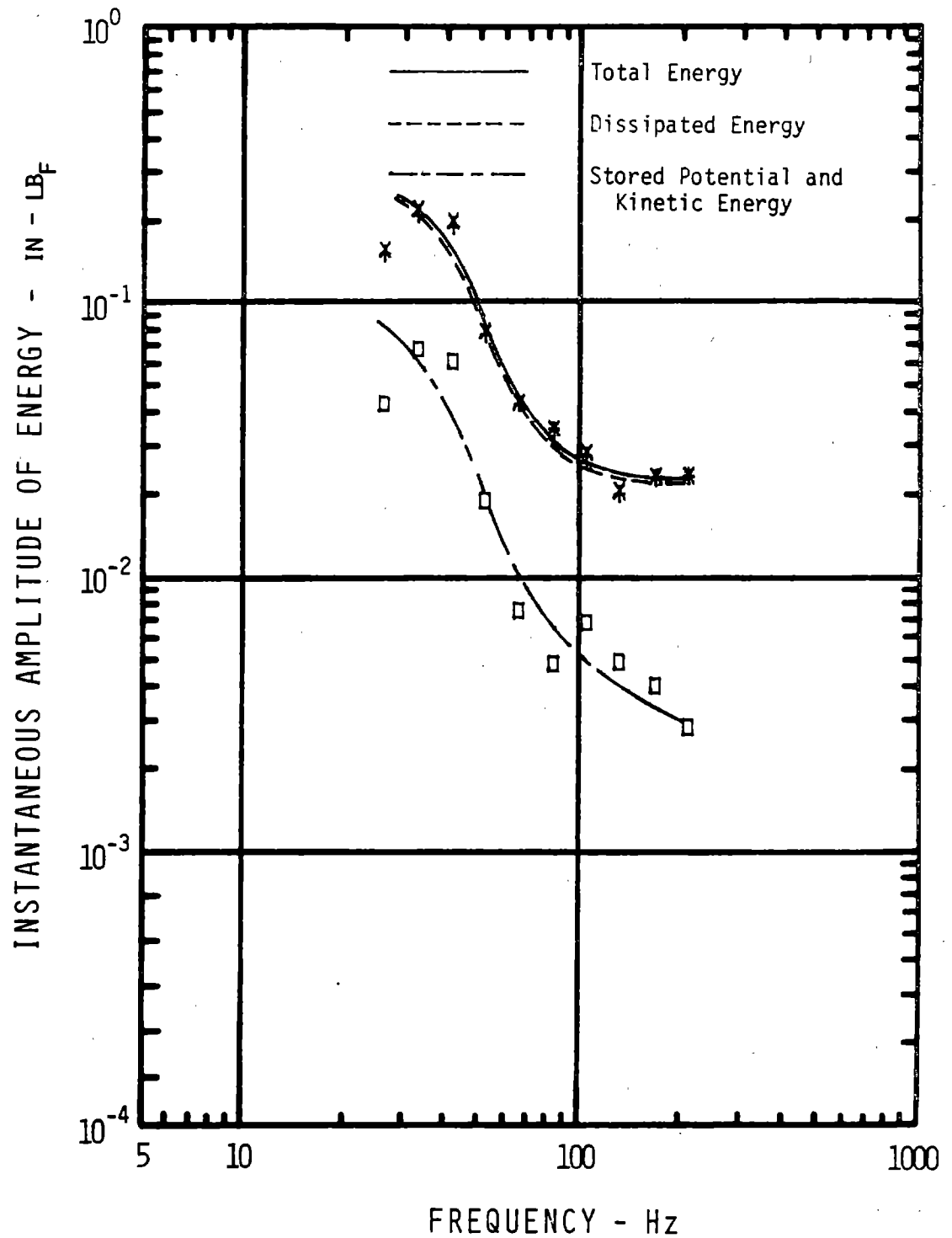
Figure 41 Make-Up of Instantaneous Energy Directed into the Hand for Vibration in the Horizontal Direction - 2 lb f Finger Grip
