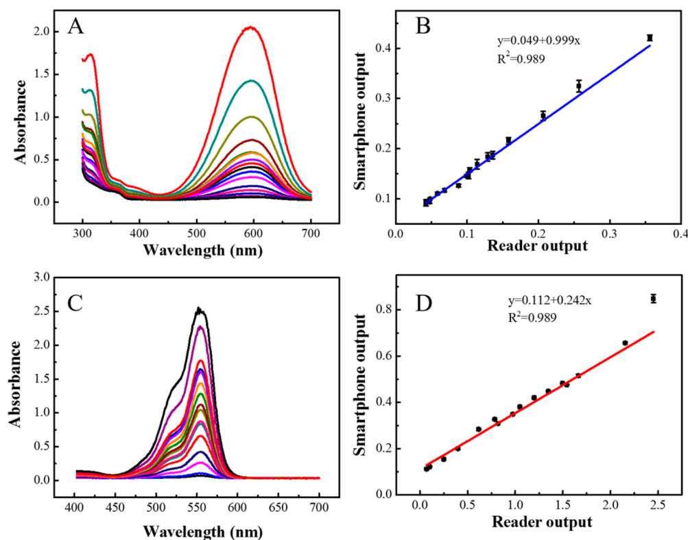
Figure 2. (A) UV spectrum with different concentrations of methyl blue obtained by a laboratory microplate reader. (B) Correlation of results obtained by laboratory microplate reader and the smartphone single-stripe reader using the red channel. (C) UV spectrum with different concentrations of rhodamine B obtained by a laboratory microplate reader. (D) Correlation of results obtained by using a laboratory microplate reader and the smartphone single-stripe reader using the green channel.
