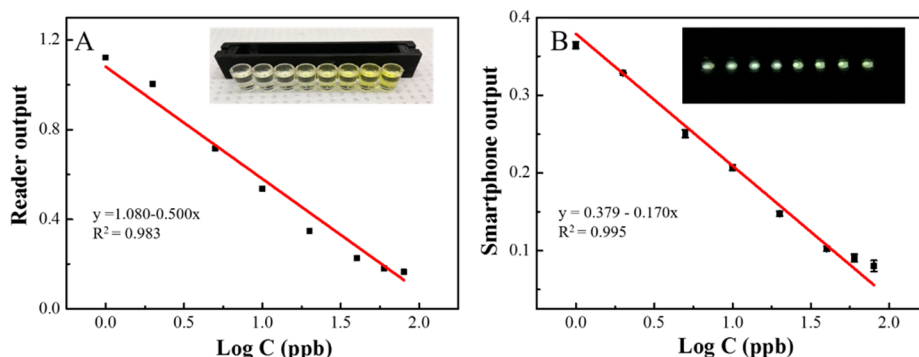
Figure 5. (A) Linear relationship between microplate reader output vs the logarithm of target concentration. Inset: visual figure of single stripe vs different concentrations of target 2,4-D (B) Linear relationship between smartphone output vs the logarithm of target concentration. Inset: smartphone image of single stripe vs different concentrations of target 2,4-D (from left to right: 80, 60, 40, 20, 10, 5, 2 and 1 ppb).
