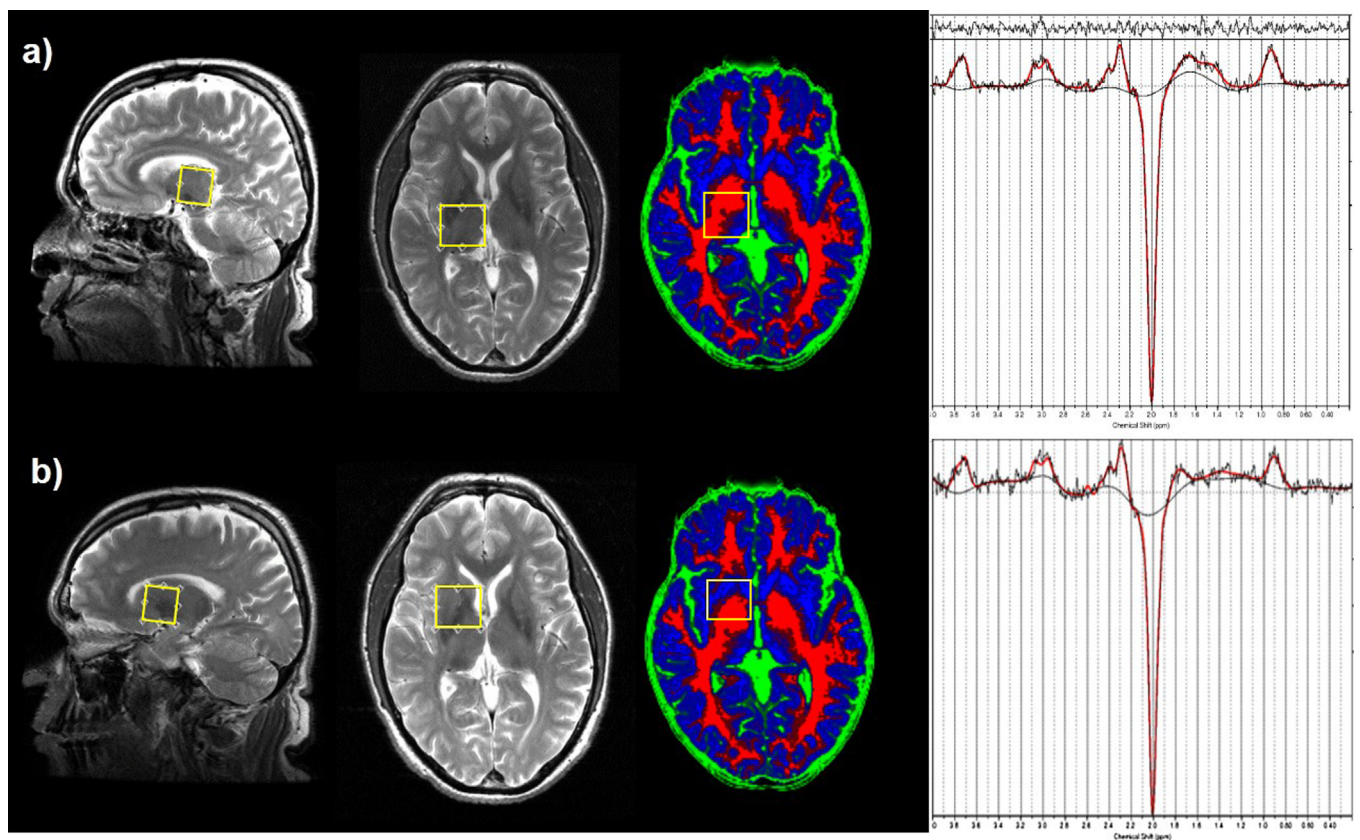
Fig. 2. Thalamus a) and striatum b) VOI for GABA measurements shown on sagittal and AC-PC aligned views on T2-weighted images, and on an axial view of a brain tissue map (red: white matter, blue: grey matter, green: CSF). Please note the tissue maps have a slightly different angulation from the AC-PC aligned T2-weighted images. Also shown are typical GABA-edited spectra from thalamus (top) and striatum (bottom) fitted with LCModel (red lines). (For interpretation of the references to colour in this figure legend, the reader is referred to the web version of this article.)
