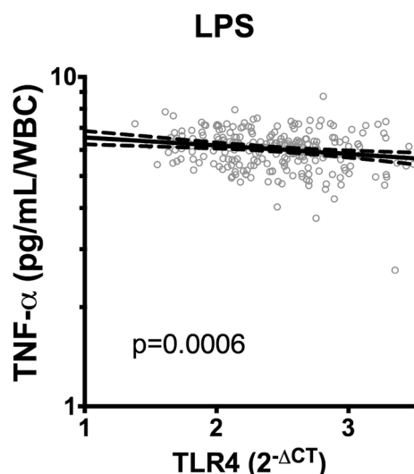
Fig. 2 TLR4 mRNA expression inversely correlates with TNF \alpha production. TLR4 mRNA was measured from unstimulated whole blood. TLR4 was normalized to the housekeeping gene 18s RNA using the 2^{-\Delta CT} method. TNF \alpha is measured after stimulation with lipopolysaccharide (LPS) (1 ng/ml) for 24 h. TNF \alpha (Logged) is reported as pg/ml/WBC. The center line is the line of best fit of a simple linear regression and the dashed lines are the 95% confidence intervals. The reported p value is whether the slope of the line is significantly non-zero
