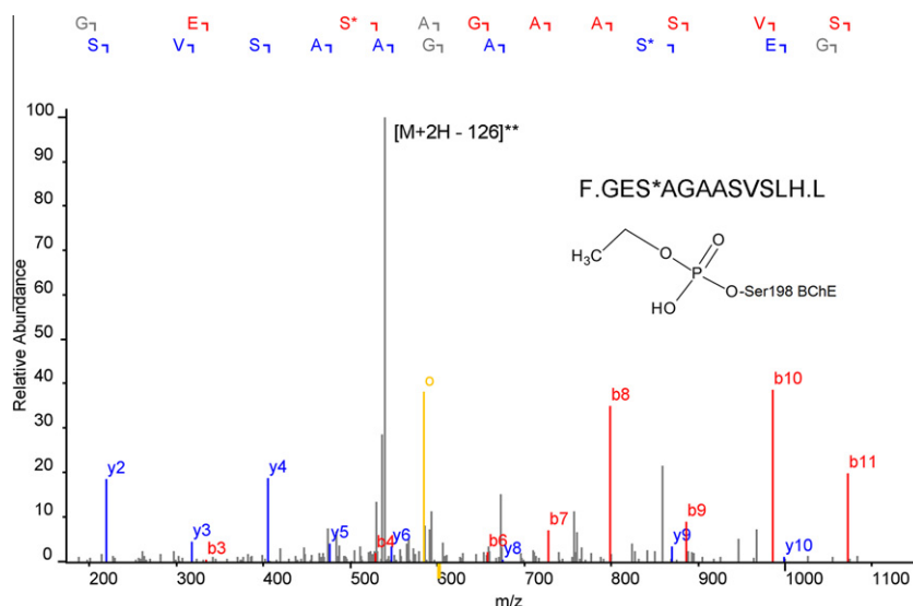
Fig. 4. Identification of chlorpyrifos exposure in plasma of an agricultural worker. The adduct on the active-site serine corresponds to the aged mono-ethyl phosphate.
