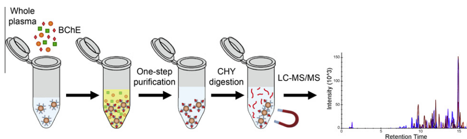
Fig. 1. Immunomagnetic bead separation of BChE coupled to LC-MS/MS analysis. This protocol efficiently purifies human BChE from 100 \mu l of plasma or less in one single step, and is readily adaptable for high-throughput analytical protocols. Samples are digested on-beads with chymotrypsin (CHY) and analyzed by LC-MS/MS.
