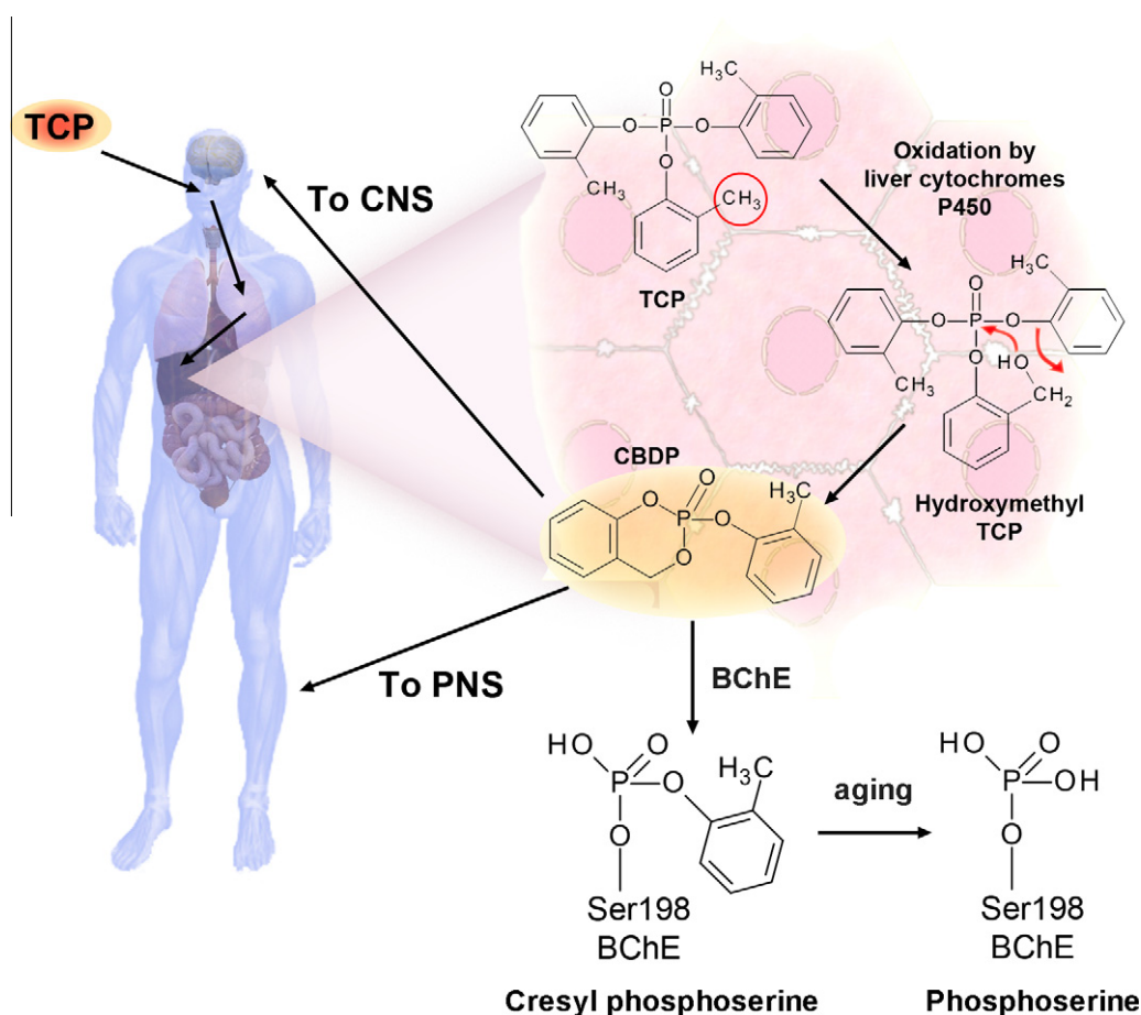
Fig. 2. Bioactivation of tricesyl phosphate (TCP) to the highly toxic metabolite cyclic saligenin cresyl phosphate (CBDP) by the liver cytochromes P450. CBDP affects both the central (CNS) and peripheral nervous system (PNS). CBDP inhibits BChE yielding a cresyl phosphate on the serine 198 of the active site that ages to phosphoserine.
