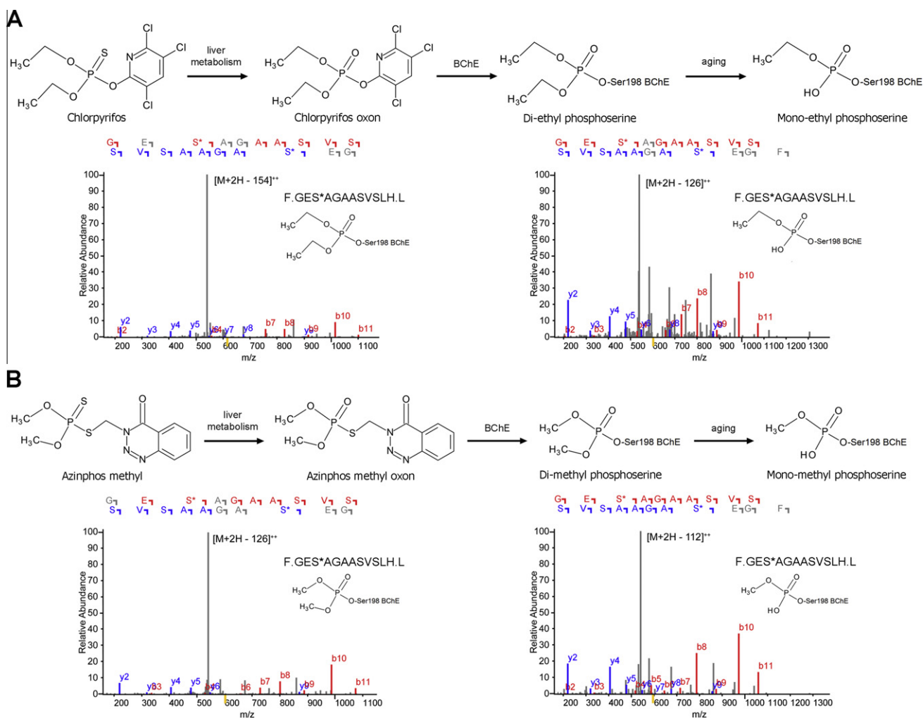
Fig. 3. OP insecticides and MS analysis using in vitro inhibited BChE. (A) Metabolism, BChE adduction and aging of chlorpyrifos. The MS analysis of the BChE active-site peptide detected both adducts, the di-ethyl phosphoserine and the aged mono-ethyl phosphoserine. (B) Metabolism, BChE adduction and aging of azinphos methyl. The MS analysis of the BChE active-site peptide detected both adducts, the di-methyl phosphoserine and the aged mono-methyl phosphoserine.
