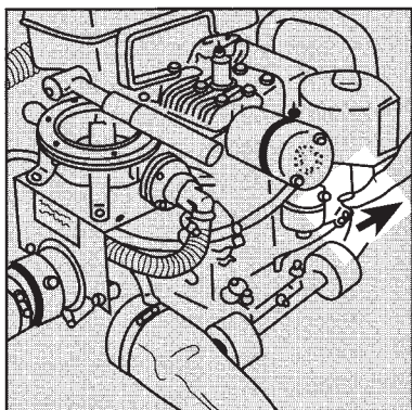
9. Choke
