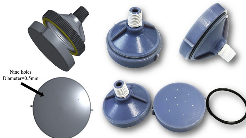
Figure 2. Nozzles for spraying.
