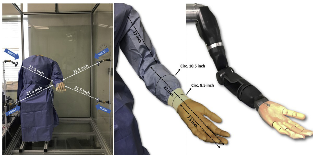
Figure 1. The experimental chamber and modular prosthetic limb.
