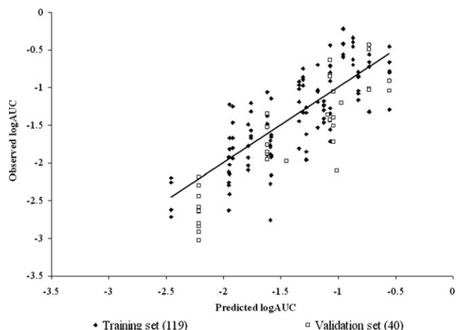
FIG. 4. Model of Abraham and Martins of the IPPSF training and validation set data with no MF. r^2 = 0.60 , adj. r^2 = 0.58 , q_{LOO}^2 = 0.56 , q_{L25\%}^2 = 0.56 , and q_{EXT}^2 = 0.72 .
