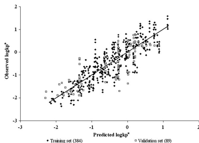
FIG. 2. Model of Abraham and Martins of the PSFT training and validation set data with MF = HBAcc (the number of hydrogen bond acceptors). r^2 = 0.73 , adj. r^2 = 0.73 , q^2_{\text{LOO}} = 0.73 , q^2_{\text{L25\%}} = 0.72 , and q^2_{\text{EXT}} = 0.61 .
