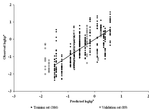
FIG. 1. Model of Abraham and Martins of the PSFT training and validation set data with no MF. r^2 = 0.53 , adj. r^2 = 0.52 , q^2_{\text{LOO}} = 0.51 , q^2_{\text{L25\%}} = 0.51 , and q^2_{\text{EXT}} = 0.41 .
