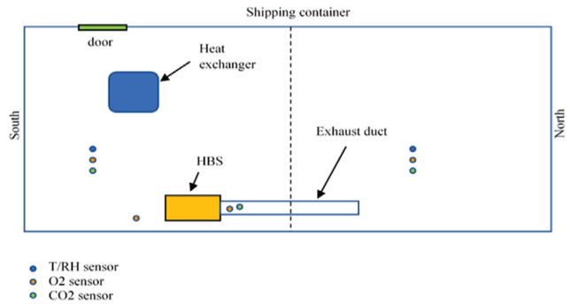
Fig. 5 Sensor locations inside the shipping container
