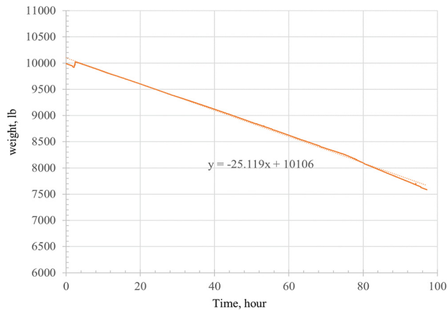
Fig. 10 The recorded gross weight during the test. The slope of the line showed the dewar lost 25.1 lb of cryogenic air per hour, i. e., the system supplied the shipping container with cryogenic air at a rate of 25.1 lb/h.
