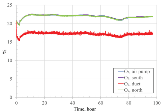
Fig. 11 The %O 2 measured at various locations during Test #2
