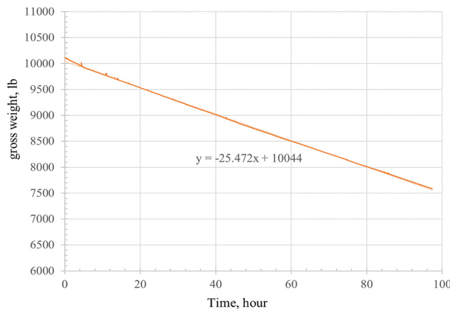
Fig. 7 The recorded gross dewar weight during the test. The slope of the line showed the dewar lost 25.5 lb of cryogenic air loss per hour, i.e., the system supplied the shipping container with cryogenic air at a rate of 25.5 lb/h.
