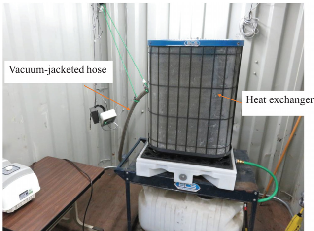
Fig. 4 The heat exchanger located inside of the shipping container. The cryogenic air was delivered to the heat exchanger through a vacuum-jacketed hose from the dewar. The liquid air vaporized at the heat exchanger and turned into gaseous air. The collected water was drained to the storage tank underneath.
