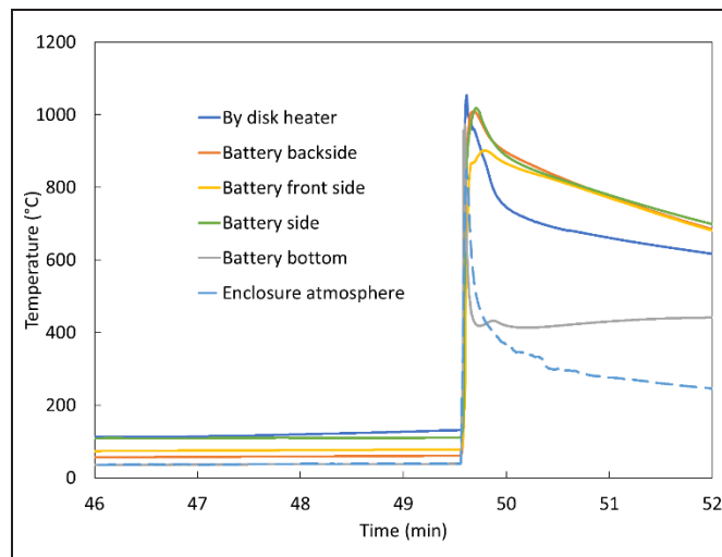
Figure 7. Time traces of battery pack and atmospheric temperatures inside of the XP enclosure
