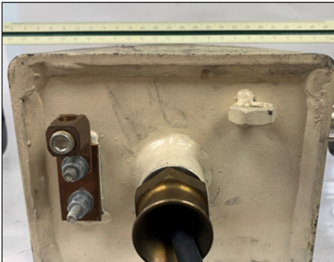
Figure 12. Thermal runaway pressure deformed the XP enclosure bottom plate beyond allowable limits
